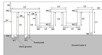
Figure 3: Antenna Dimensions
