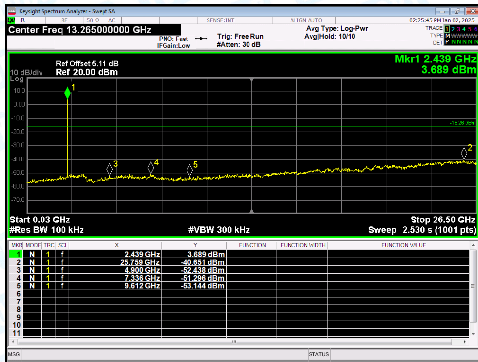
Tx. Spurious NVNT ZigBee 2445MHz Ant1 Emission
