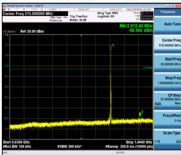
Band12-3MHz-QPSK-23165-1-0-High-30-1000--58.56-PASS
