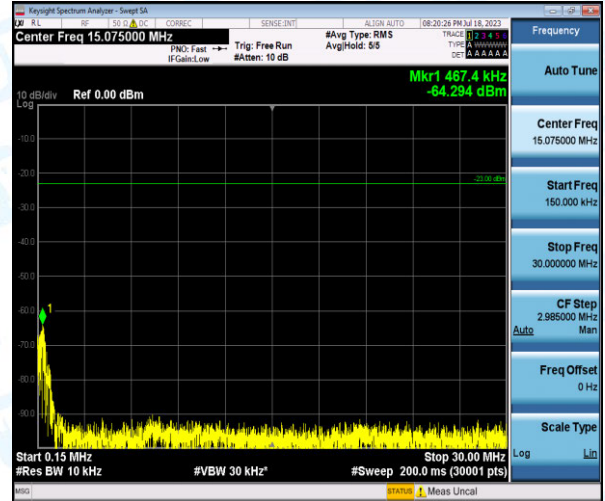
Band12-3MHz-QPSK-23025-1-0-Low-0.15-30--64.29-PASS
