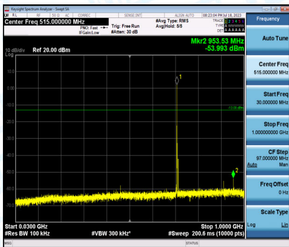
Band12-3MHz-16QAM-23165-1-0-High-30-1000--53.99-PASS
