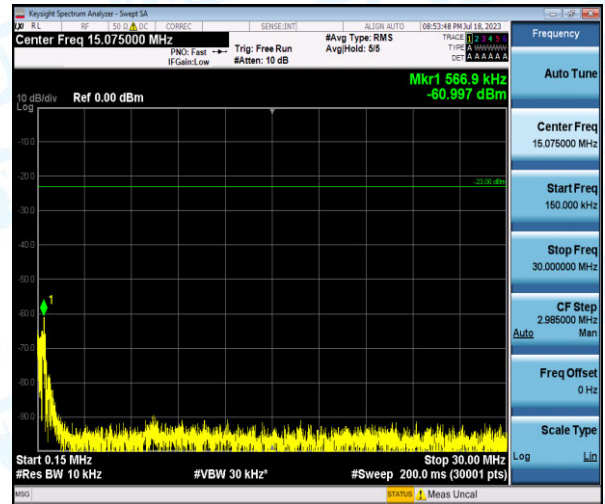
Band12-5MHz-16QAM-23035-1-0-Low-0.15-30--61-PASS
