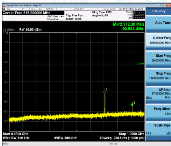
Band12-1.4MHz-QPSK-23173-1-0-High-30-1000--55.68-PASS
