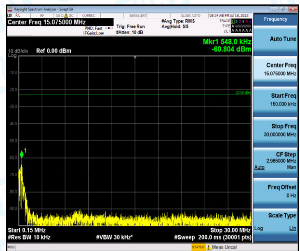
Band12-5MHz-16QAM-23095-1-0-Low-0.15-30--60.8-PASS
