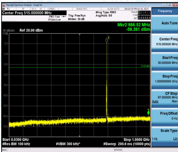
Band12-3MHz-QPSK-23025-1-0-Low-30-1000--59.26-PASS
