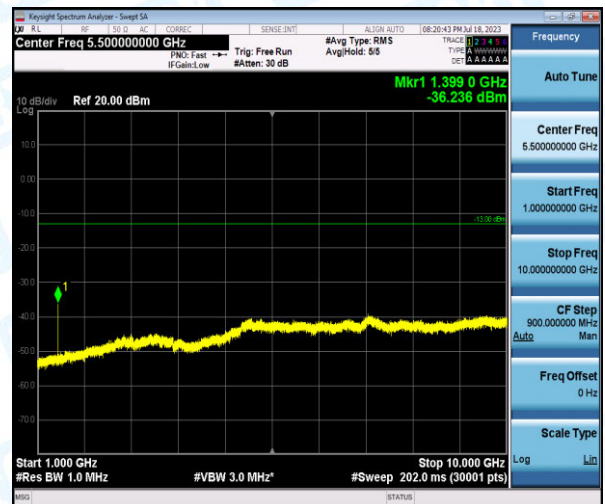
Band12-3MHz-QPSK-23025-1-0-Low-1000-10000--36.24-PASS
