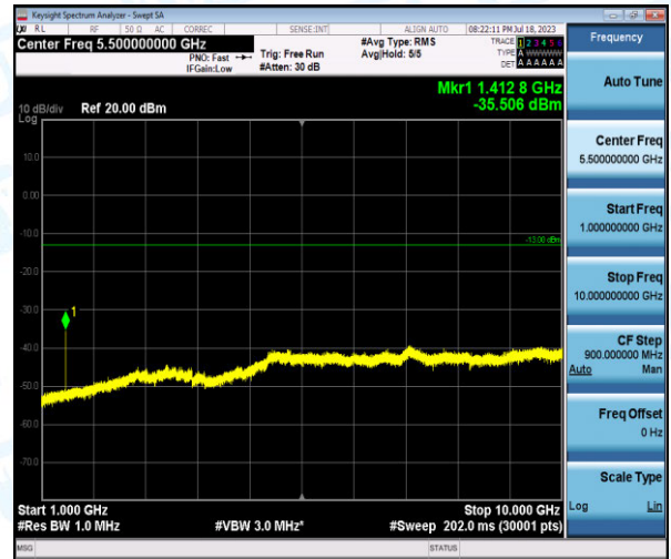
Band12-3MHz-16QAM-23095-1-0-Low-1000-10000--35.51-PASS
