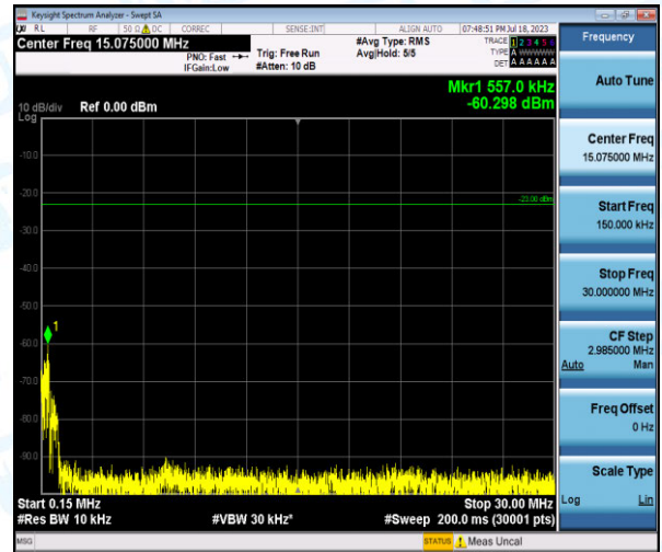
Band12-1.4MHz-16QAM-23017-1-0-Low-0.15-30--60.3-PASS
