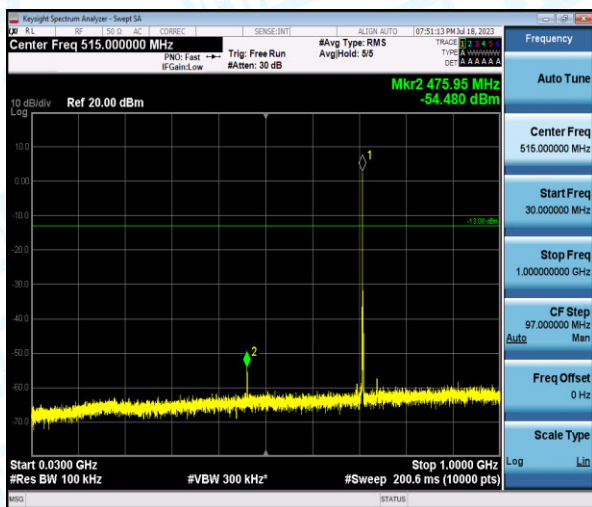
Band12-1.4MHz-16QAM-23173-1-0-High-30-1000--54.48-PASS
