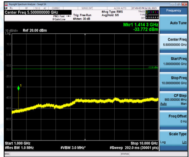
Band12-1.4MHz-QPSK-23095-1-0-Low-1000-10000--33.77-PASS
