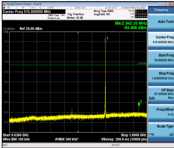
Band12-1.4MHz-16QAM-23095-1-0-Low-30-1000--54.47-PASS
