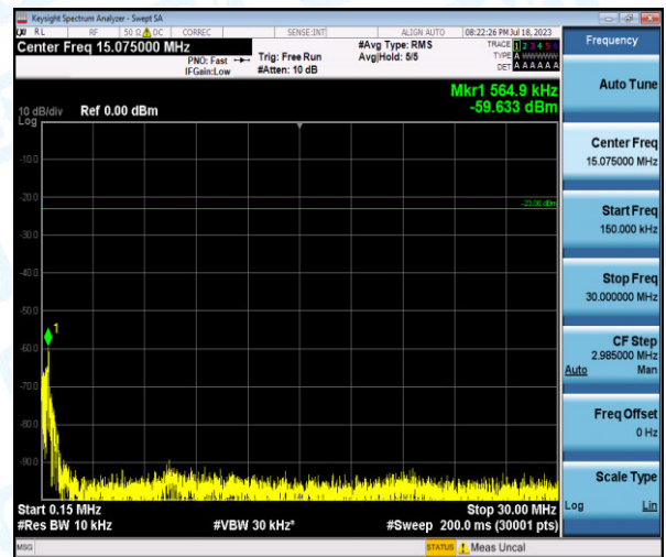
Band12-3MHz-QPSK-23165-1-0-High-0.15-30--59.63-PASS
