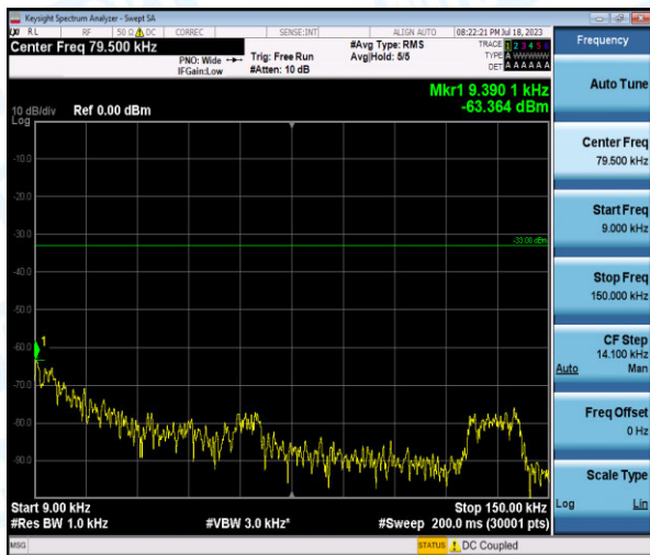
Band12-3MHz-QPSK-23165-1-0-High-0.009-0.15--63.36-PASS
