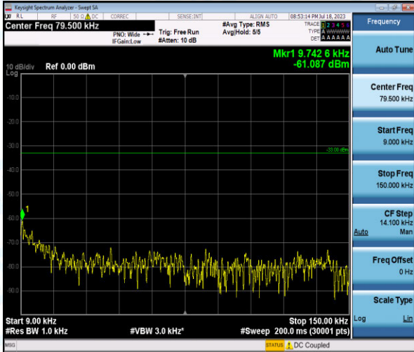
Band12-5MHz-QPSK-23035-1-0-Low-0.009-0.15--61.09-PASS
