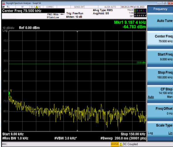
Band12-3MHz-QPSK-23025-1-0-Low-0.009-0.15--64.78-PASS
