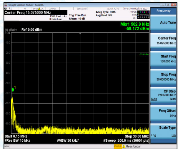
Band12-1.4MHz-16QAM-23173-1-0-High-0.15-30--59.17-PASS
