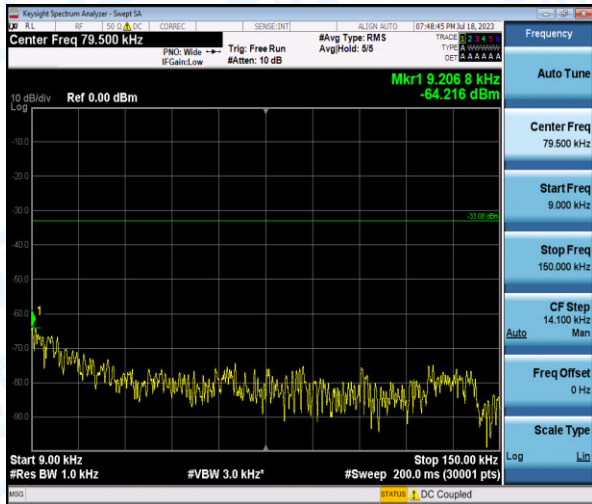
Band12-1.4MHz-16QAM-23017-1-0-Low-0.009-0.15--64.22-PASS
