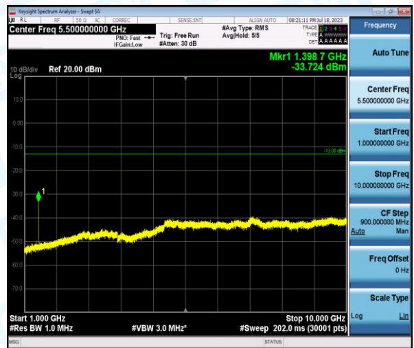
Band12-3MHz-16QAM-23025-1-0-Low-1000-10000--33.72-PASS
