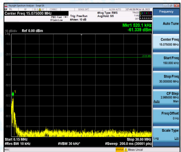
Band12-1.4MHz-16QAM-23095-1-0-Low-0.15-30--61.34-PASS
