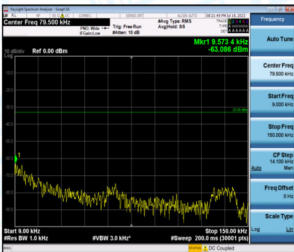
Band12-3MHz-16QAM-23095-1-0-Low-0.009-0.15--63.09-PASS
