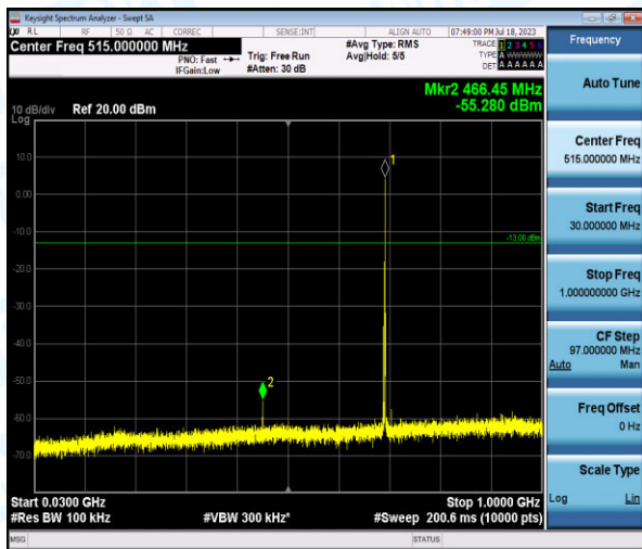
Band12-1.4MHz-16QAM-23017-1-0-Low-30-1000--55.28-PASS
