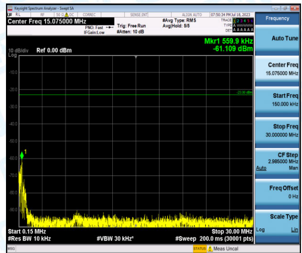
Band12-1.4MHz-QPSK-23173-1-0-High-0.15-30--61.11-PASS
