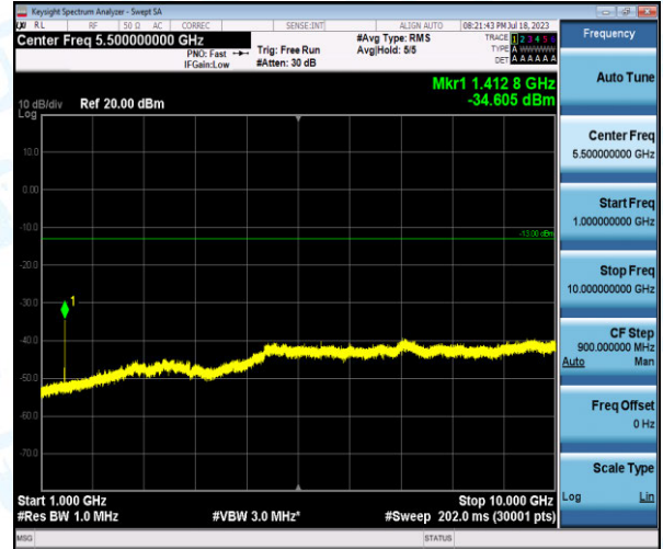
Band12-3MHz-QPSK-23095-1-0-Low-1000-10000--34.61-PASS
