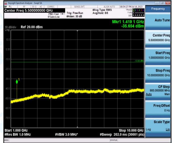
Band12-5MHz-QPSK-23095-1-0-Low-1000-10000--35.65-PASS
