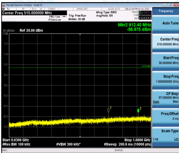
Band12-3MHz-16QAM-23025-1-0-Low-30-1000--56.98-PASS
