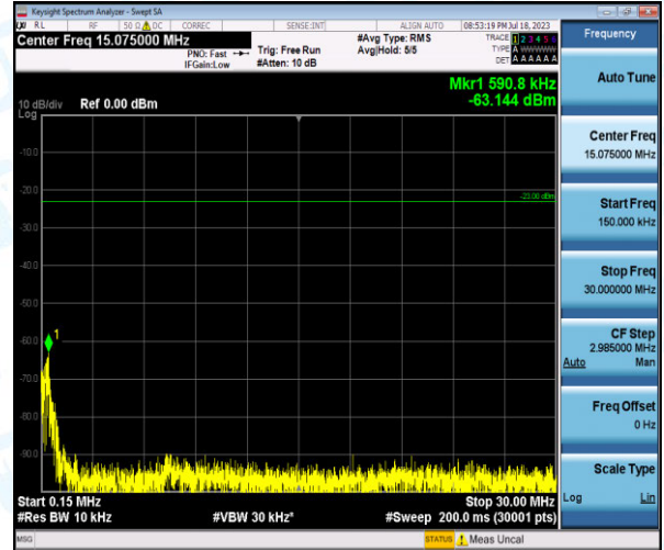
Band12-5MHz-QPSK-23035-1-0-Low-0.15-30--63.14-PASS
