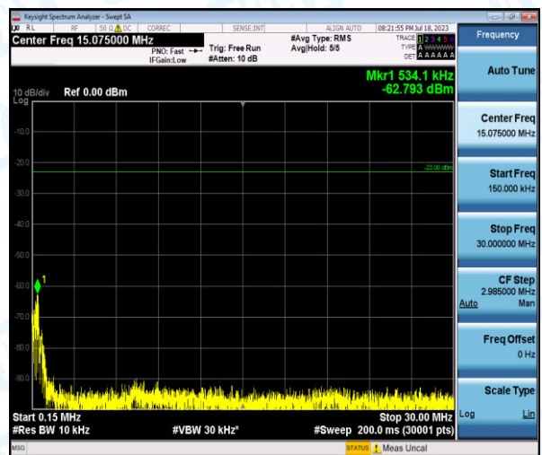
Band12-3MHz-16QAM-23095-1-0-Low-0.15-30--62.79-PASS
