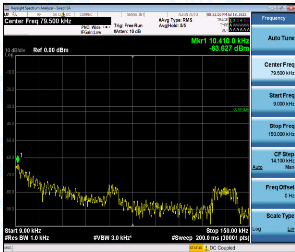
Band12-3MHz-16QAM-23165-1-0-High-0.009-0.15--63.63-PASS
