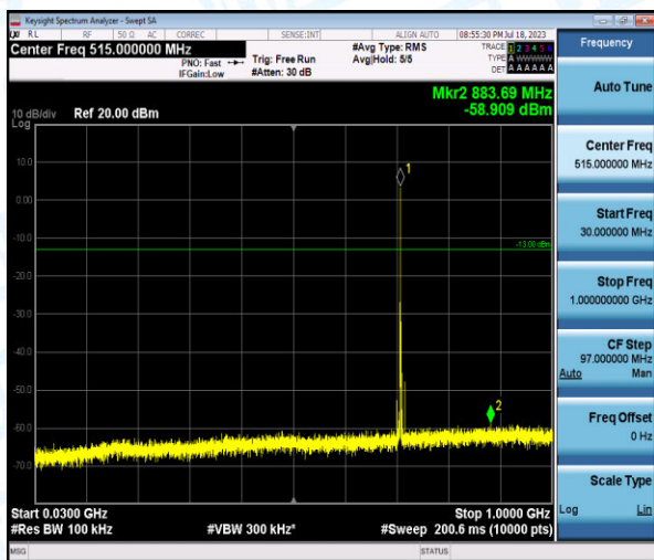
Band12-5MHz-QPSK-23155-1-0-High-30-1000--58.91-PASS
