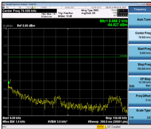
Band12-5MHz-QPSK-23155-1-0-High-0.009-0.15--64.83-PASS
