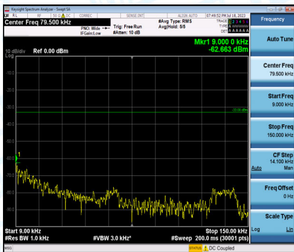
Band12-1.4MHz-16QAM-23095-1-0-Low-0.009-0.15--62.66-PASS
