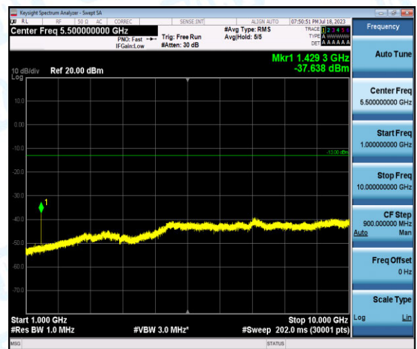
Band12-1.4MHz-QPSK-23173-1-0-High-1000-10000--37.64-PASS
