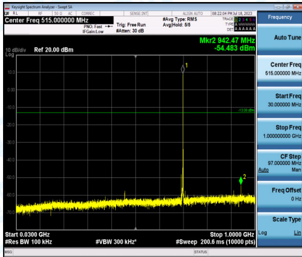
Band12-3MHz-16QAM-23095-1-0-Low-30-1000--54.48-PASS
