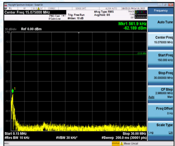
Band12-5MHz-QPSK-23155-1-0-High-0.15-30--62.19-PASS
