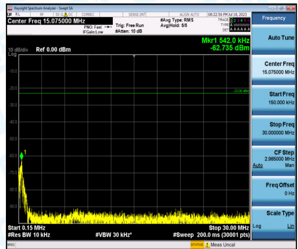
Band12-3MHz-16QAM-23165-1-0-High-0.15-30--62.74-PASS
