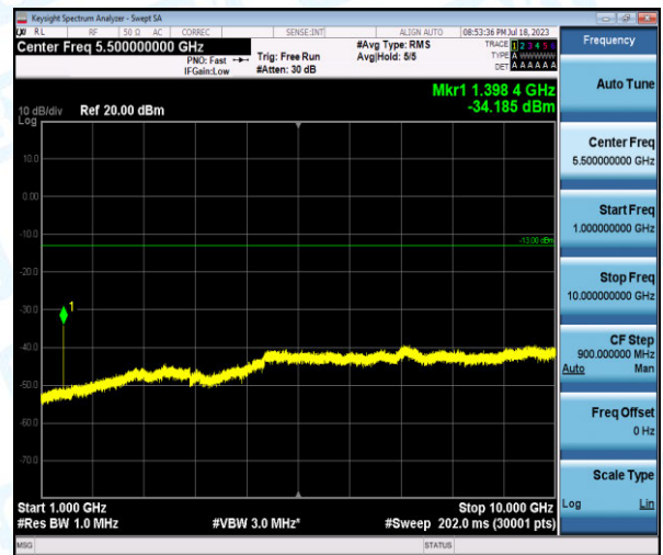
Band12-5MHz-QPSK-23035-1-0-Low-1000-10000--34.19-PASS
