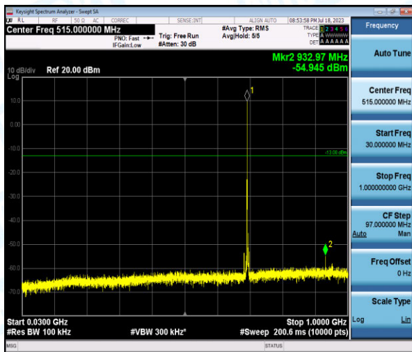
Band12-5MHz-16QAM-23035-1-0-Low-30-1000--54.95-PASS
