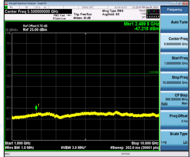
Band26-15MHz-16QAM-26915-1-0-Low-1000-10000--47.22-PASS
