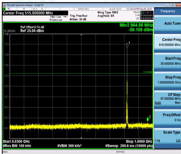
Band26-15MHz-QPSK-26865-1-0-Low-30-1000--59.11-PASS
