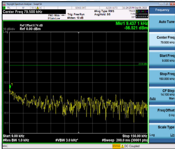
Band26-15MHz-16QAM-26865-1-0-Low-0.009-0.15--56.52-PASS
