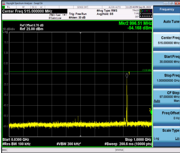
Band26-15MHz-16QAM-26915-1-0-Low-30-1000--54.17-PASS
