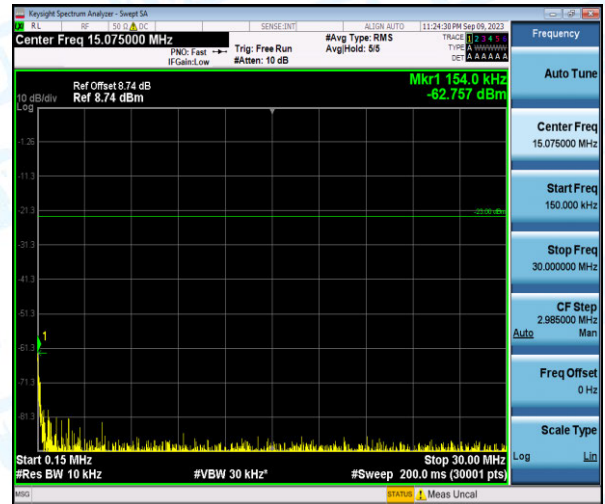
Band26-15MHz-16QAM-26865-1-0-Low-0.15-30--62.76-PASS
