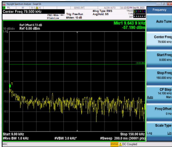
Band26-10MHz-QPSK-26840-1-0-Low-0.009-0.15--57.19-PASS
