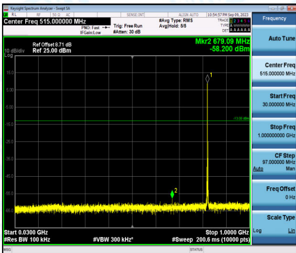
Band26-3MHz-16QAM-26805-1-0-Low-30-1000--58.2-PASS
