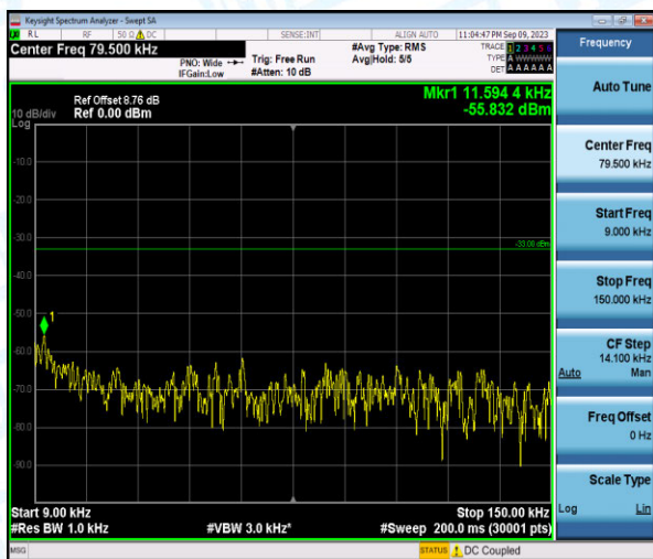
Band26-5MHz-QPSK-26915-1-0-Low-0.009-0.15--55.83-PASS
