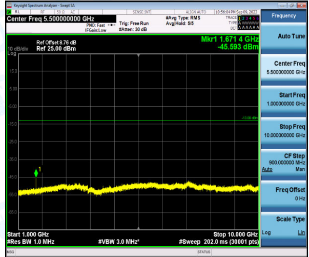
Band26-3MHz-16QAM-26915-1-0-Low-1000-10000--45.59-PASS
