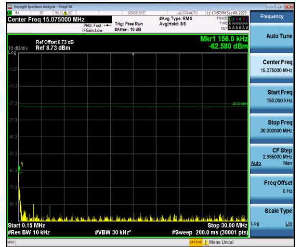
Band26-10MHz-QPSK-26840-1-0-Low-0.15-30--62.58-PASS
