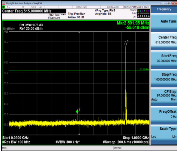
Band26-3MHz-16QAM-26915-1-0-Low-30-1000--55.02-PASS
