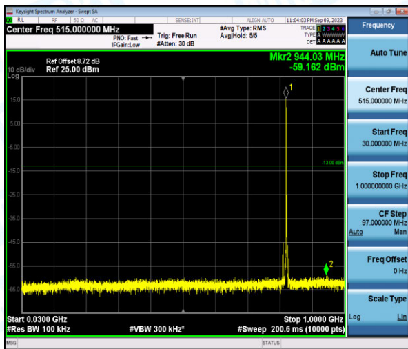
Band26-5MHz-QPSK-26815-1-0-Low-30-1000--59.16-PASS
