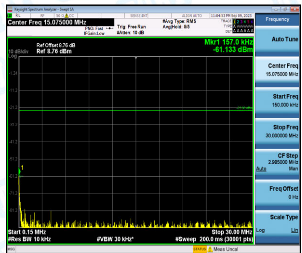
Band26-5MHz-QPSK-26915-1-0-Low-0.15-30--61.13-PASS
