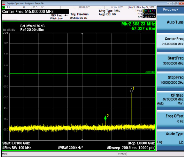
Band26-1.4MHz-QPSK-26915-1-0-Low-30-1000--57.03-PASS
