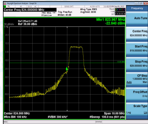
Band26-5MHz-16QAM-26815-6-0-Low--22.84-PASS
