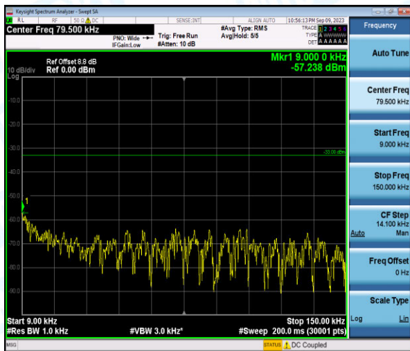
Band26-3MHz-QPSK-27025-1-0-High-0.009-0.15--57.24-PASS
