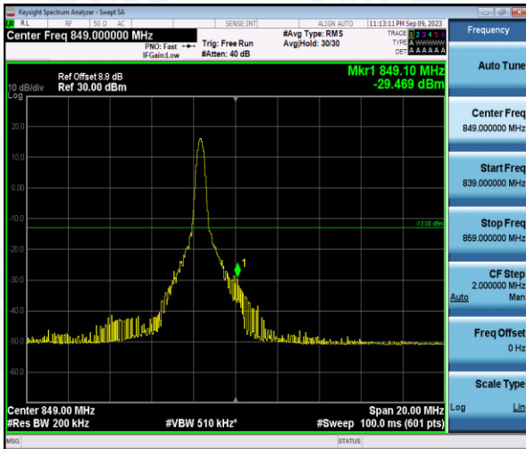
Band26-10MHz-QPSK-26990-1-0-High--29.47-PASS
