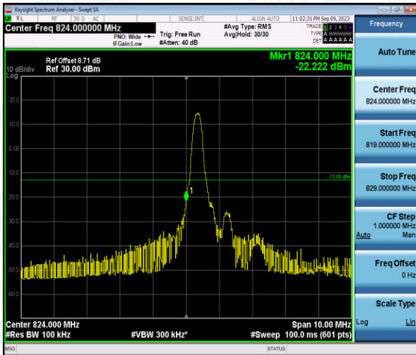
Band26-5MHz-16QAM-26815-1-0-Low--22.22-PASS
