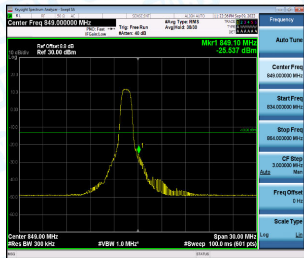
Band26-15MHz-QPSK-26965-6-0-High--25.54-PASS
