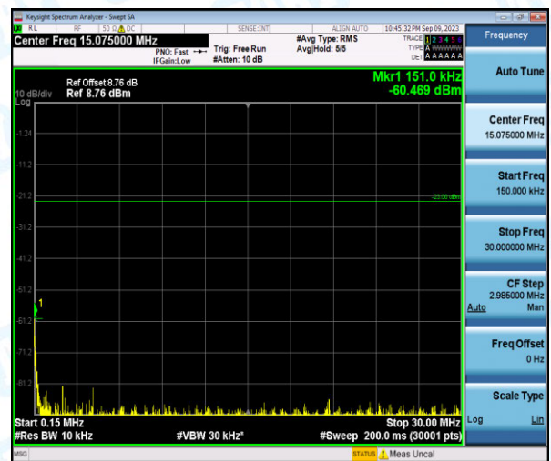
Band26-1.4MHz-16QAM-26915-1-0-Low-0.15-30--60.47-PASS
