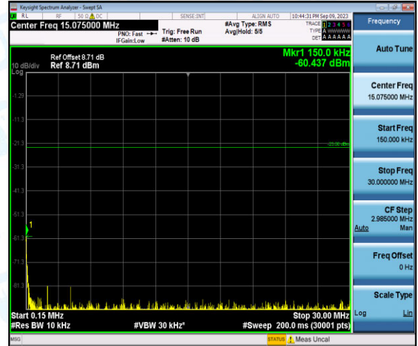
Band26-1.4MHz-16QAM-26797-1-0-Low-0.15-30--60.44-PASS
