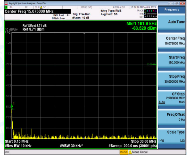
Band26-3MHz-QPSK-26805-1-0-Low-0.15-30--63.52-PASS
