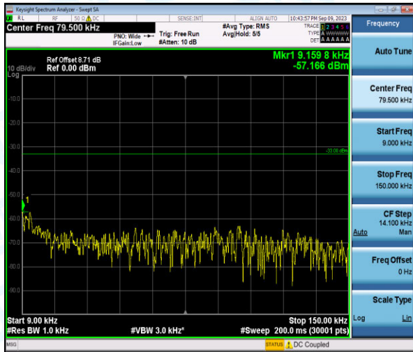
Band26-1.4MHz-QPSK-26797-1-0-Low-0.009-0.15-57.17-PASS
