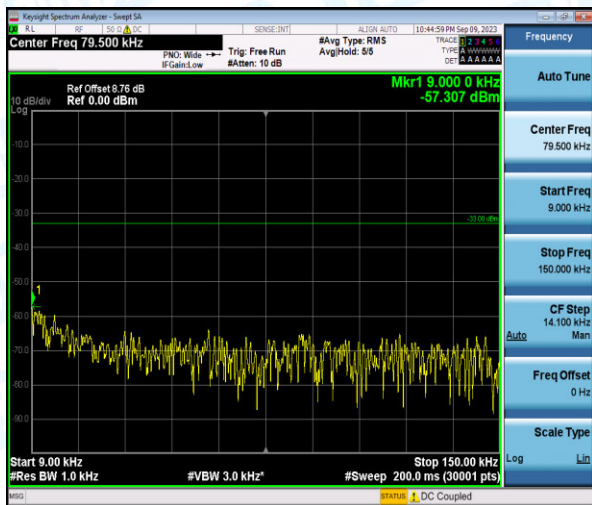
Band26-1.4MHz-QPSK-26915-1-0-Low-0.009-0.15-57.31-PASS
