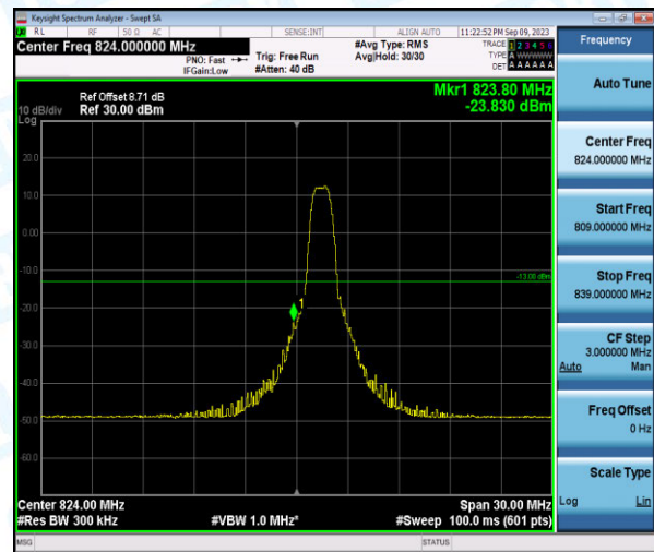
Band26-15MHz-QPSK-26865-6-0-Low--23.83-PASS
