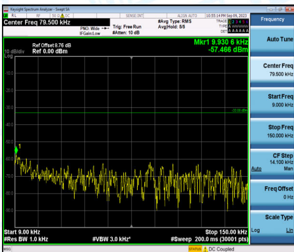
Band26-3MHz-QPSK-26915-1-0-Low-0.009-0.15--57.47-PASS
