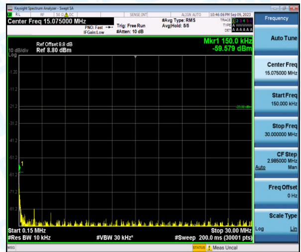
Band26-1.4MHz-QPSK-27033-1-0-High-0.15-30--59.58-PASS
