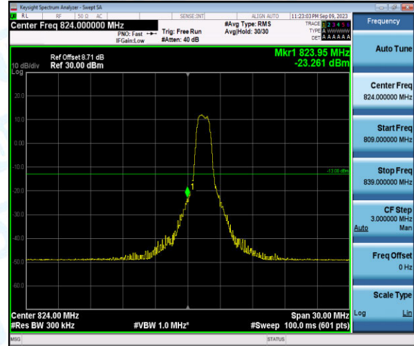
Band26-15MHz-16QAM-26865-6-0-Low--23.26-PASS
