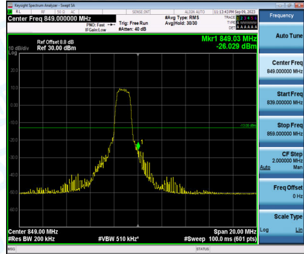
Band26-10MHz-16QAM-26990-6-0-High--26.03-PASS
