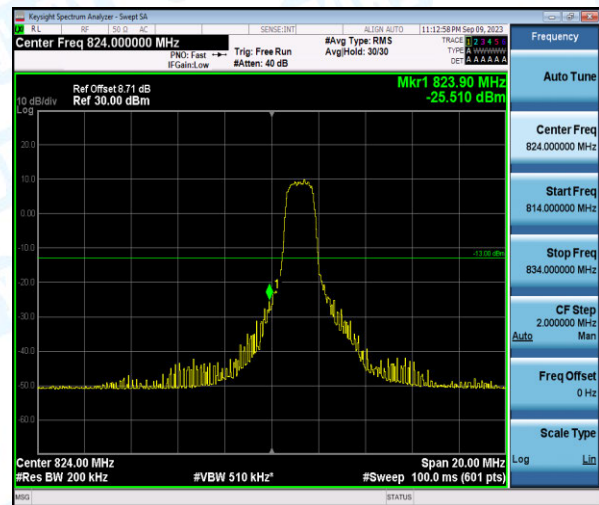
Band26-10MHz-16QAM-26840-6-0-Low--25.51-PASS
