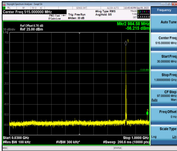
Band26-1.4MHz-16QAM-26915-1-0-Low-30-1000--56.22-PASS
