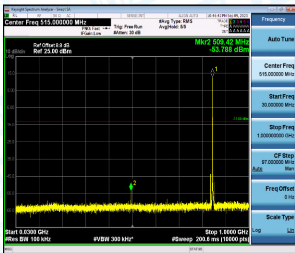
Band26-1.4MHz-16QAM-27033-1-0-High-30-1000--53.79-PASS
