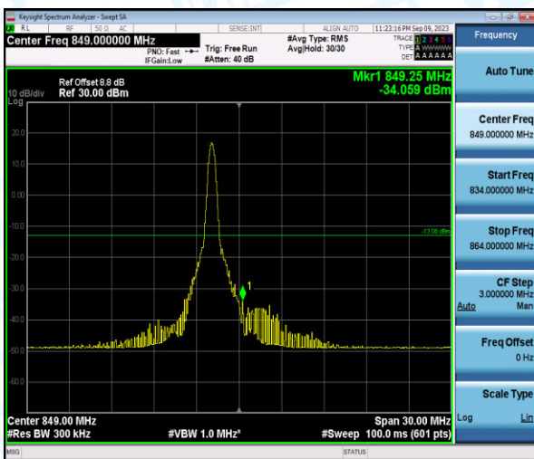
Band26-15MHz-QPSK-26965-1-0-High--34.06-PASS
