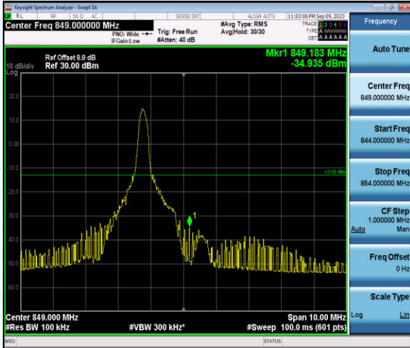
Band26-5MHz-QPSK-27015-1-0-High--34.94-PASS
