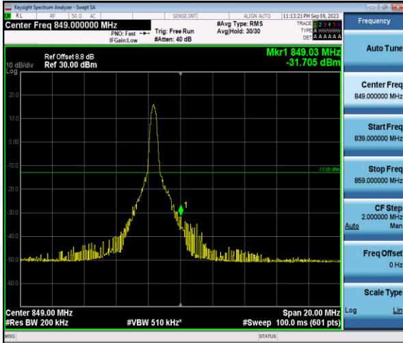
Band26-10MHz-16QAM-26990-1-0-High--31.71-PASS
