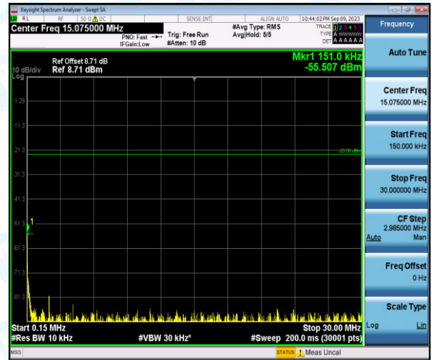
Band26-1.4MHz-QPSK-26797-1-0-Low-0.15-30--55.51-PASS
