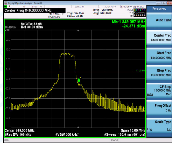
Band26-5MHz-QPSK-27015-6-0-High--24.37-PASS
