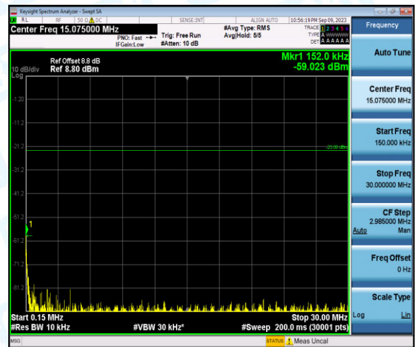
Band26-3MHz-QPSK-27025-1-0-High-0.15-30--59.02-PASS
