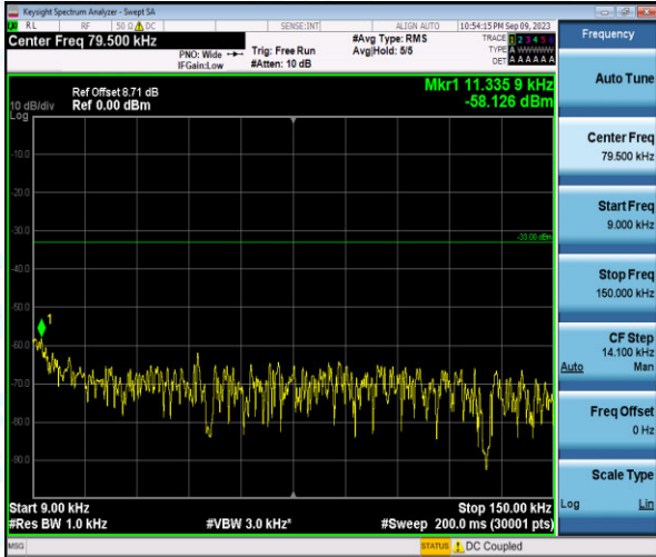
Band26-3MHz-QPSK-26805-1-0-Low-0.009-0.15--58.13-PASS
