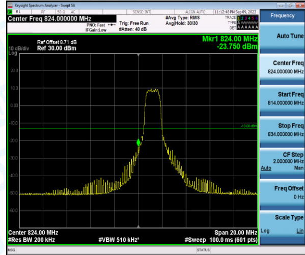
Band26-10MHz-QPSK-26840-6-0-Low--23.75-PASS
