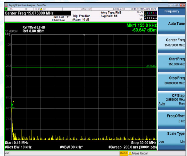
Band26-1.4MHz-16QAM-27033-1-0-High-0.15-30--60.65-PASS
