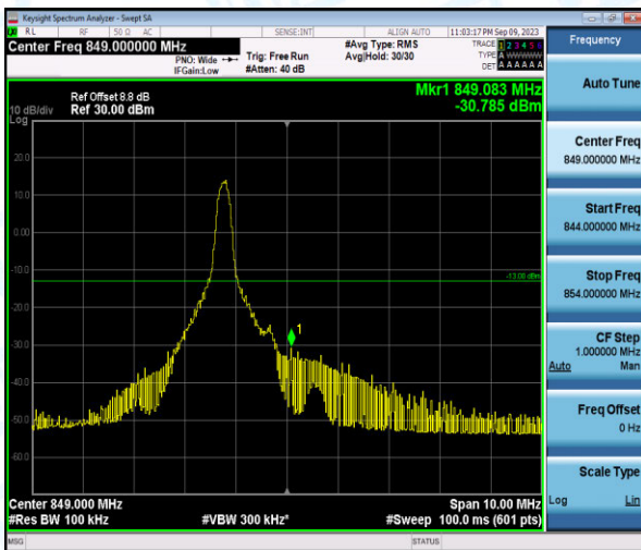
Band26-5MHz-16QAM-27015-1-0-High--30.79-PASS
