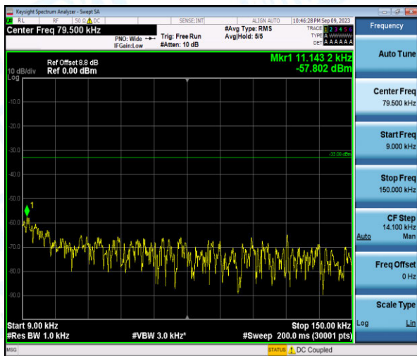
Band26-1.4MHz-16QAM-27033-1-0-High-0.009-0.15--57.8-PASS
