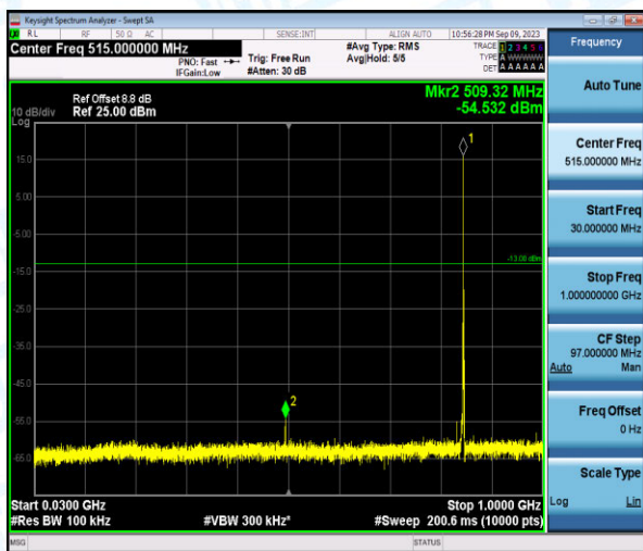
Band26-3MHz-QPSK-27025-1-0-High-30-1000--54.53-PASS
