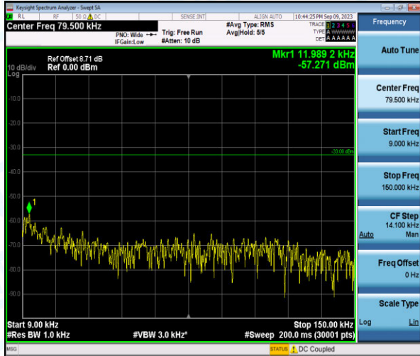
Band26-1.4MHz-16QAM-26797-1-0-Low-0.009-0.15--57.27-PASS
