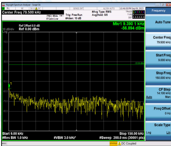
Band26-1.4MHz-QPSK-27033-1-0-High-0.009-0.15--56.89-PASS
