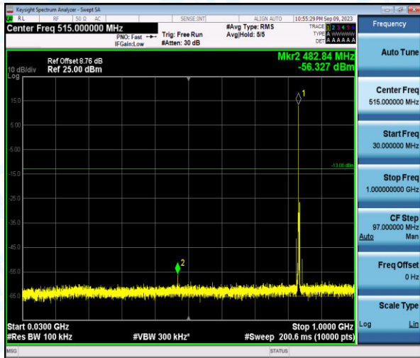
Band26-3MHz-QPSK-26915-1-0-Low-30-1000--56.33-PASS
