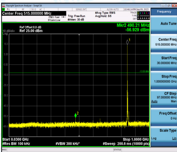
Band26-1.4MHz-QPSK-27033-1-0-High-30-1000--56.93-PASS
