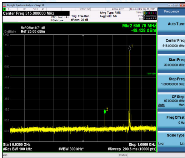
Band26-1.4MHz-16QAM-26797-1-0-Low-30-1000--49.43-PASS
