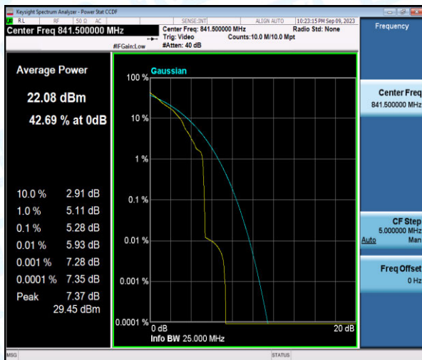
Band26-15MHz-QPSK-26965-1-0-High-5.28-<=13-PASS
