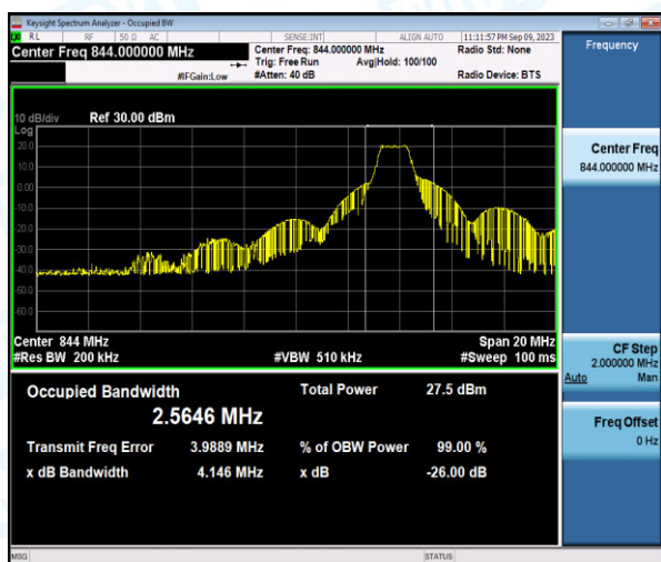
Band26-10MHz-QPSK-26990-6-0-High-2.5646-4.146-PASS
