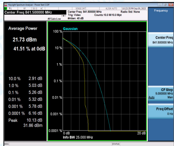
Band26-15MHz-QPSK-26965-6-0-High-5.26-<=13-PASS
