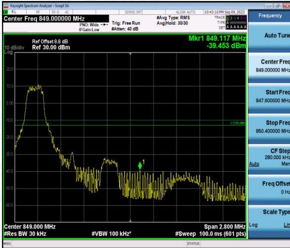
Band26-1.4MHz-QPSK-27033-1-0-High--39.45-PASS
