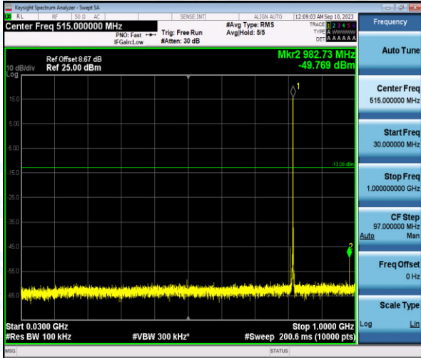
Band26-1.4MHz-16QAM-26740-1-0-Low-30-1000--49.77-PASS
