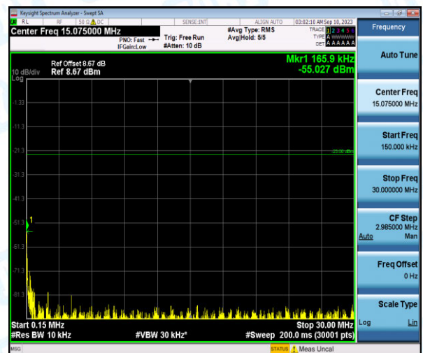
Band26-10MHz-16QAM-26740-1-0-Low-0.15-30--55.03-PASS
