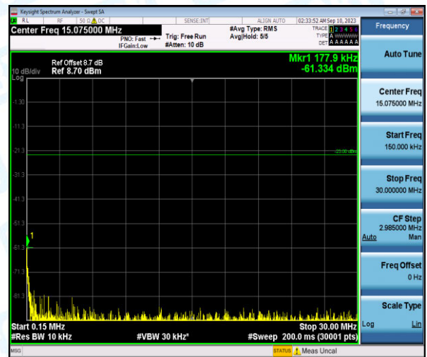
Band26-5MHz-QPSK-26785-1-0-High-0.15-30--61.33-PASS
