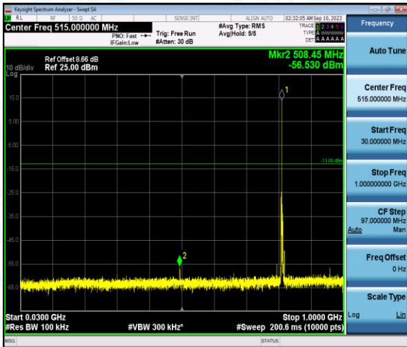
Band26-5MHz-QPSK-26715-1-0-Low-30-1000--56.53-PASS
