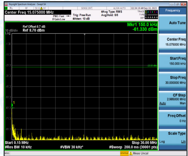
Band26-5MHz-16QAM-26785-1-0-High-0.15-30--61.33-PASS
