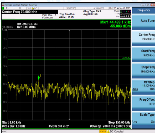
Band26-10MHz-16QAM-26740-1-0-Low-0.009-0.15--55.88-PASS
