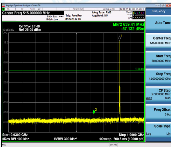
Band26-1.4MHz-16QAM-26783-1-0-High-30-1000--57.13-PASS
