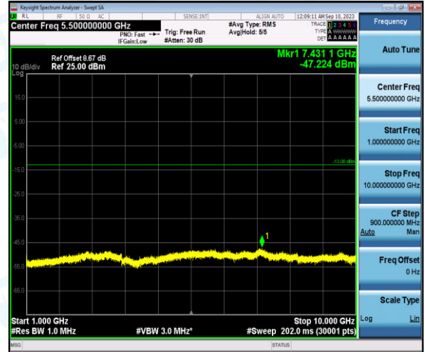
Band26-1.4MHz-16QAM-26740-1-0-Low-1000-10000--47.22-PASS
