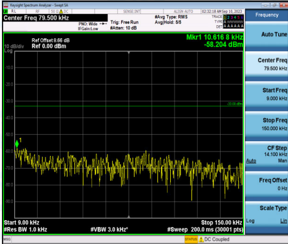
Band26-5MHz-16QAM-26715-1-0-Low-0.009-0.15--58.2-PASS
