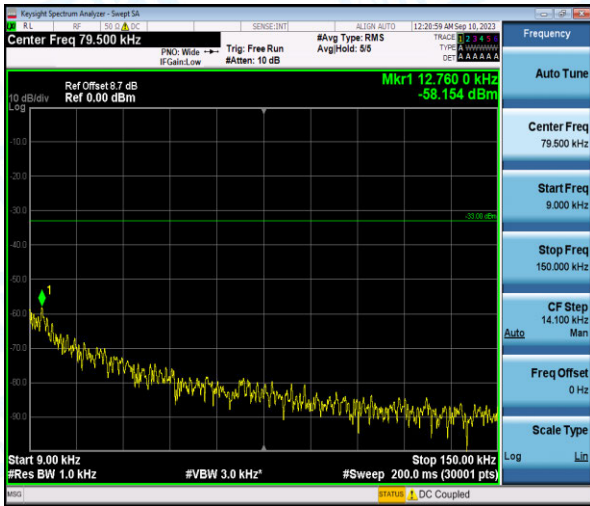
Band26-3MHz-16QAM-26775-1-0-High-0.009-0.15--58.15-PASS
