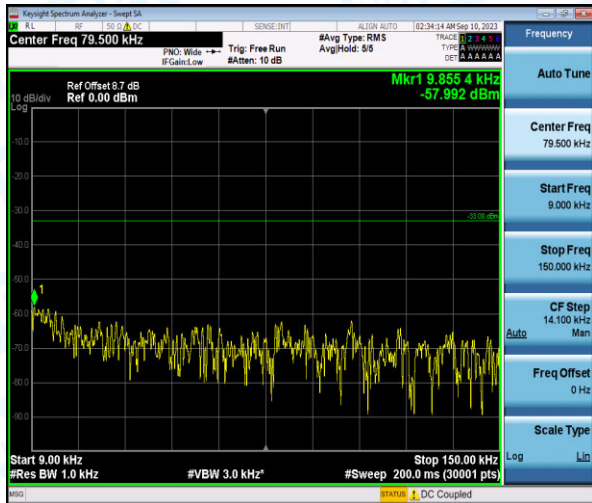
Band26-5MHz-16QAM-26785-1-0-High-0.009-0.15--57.99-PASS
