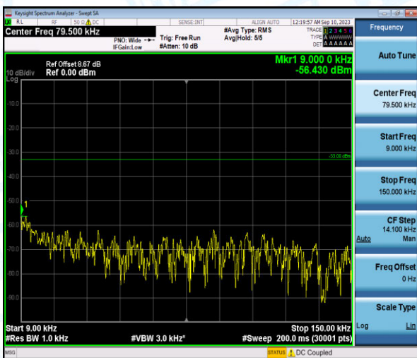
Band26-3MHz-16QAM-26740-1-0-Low-0.009-0.15--56.43-PASS
