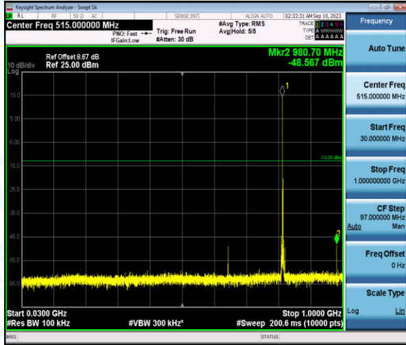
Band26-5MHz-16QAM-26740-1-0-Low-30-1000--48.57-PASS
