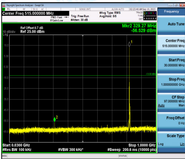
Band26-3MHz-16QAM-26775-1-0-High-30-1000--56.53-PASS
