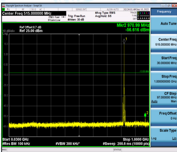
Band26-5MHz-QPSK-26785-1-0-High-30-1000--56.62-PASS
