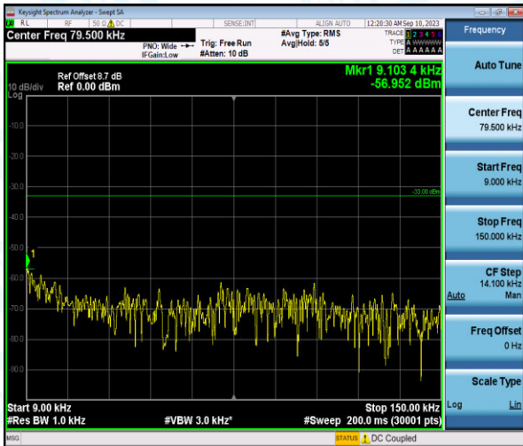
Band26-3MHz-QPSK-26775-1-0-High-0.009-0.15--56.95-PASS
