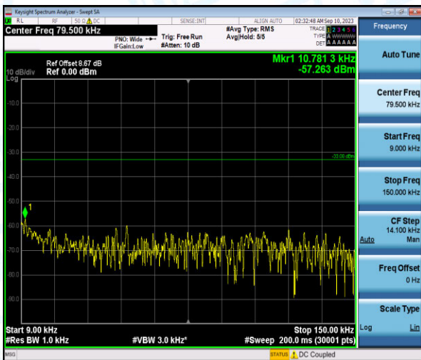
Band26-5MHz-QPSK-26740-1-0-Low-0.009-0.15--57.26-PASS
