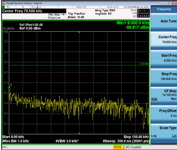
Band26-3MHz-16QAM-26705-1-0-Low-0.009-0.15--56.92-PASS
