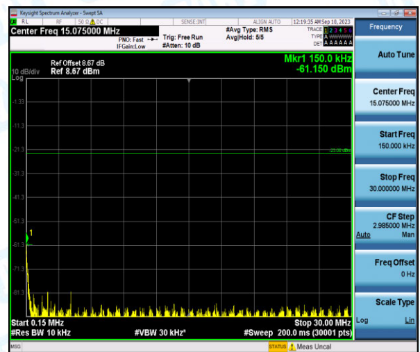
Band26-3MHz-QPSK-26740-1-0-Low-0.15-30--61.15-PASS
