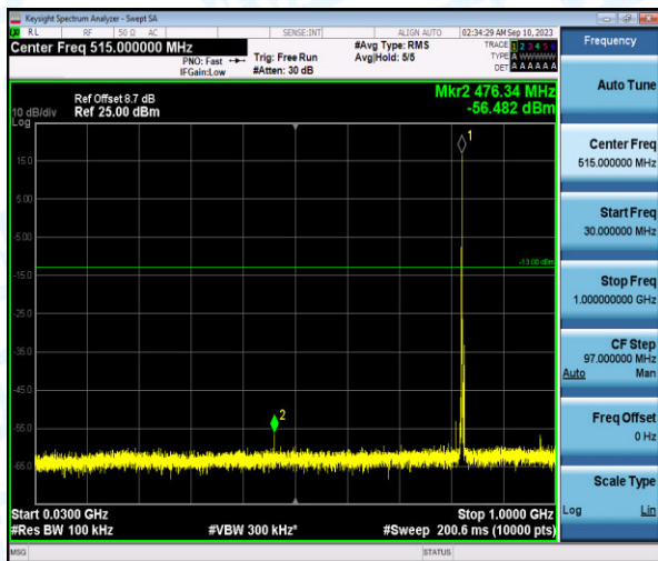
Band26-5MHz-16QAM-26785-1-0-High-30-1000--56.48-PASS
