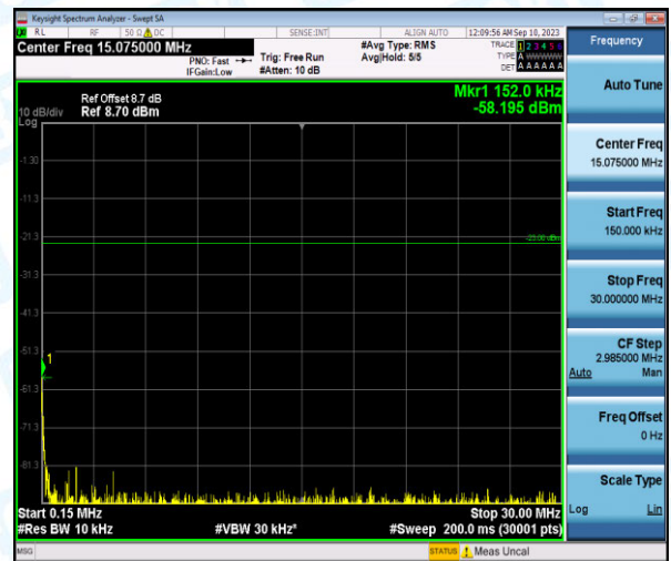
Band26-1.4MHz-16QAM-26783-1-0-High-0.15-30--58.2-PASS
