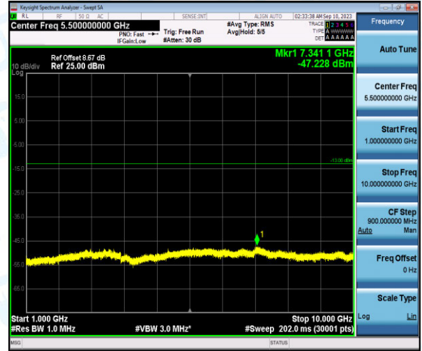
Band26-5MHz-16QAM-26740-1-0-Low-1000-10000--47.23-PASS
