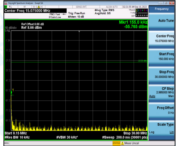
Band26-5MHz-QPSK-26715-1-0-Low-0.15-30--55.77-PASS
