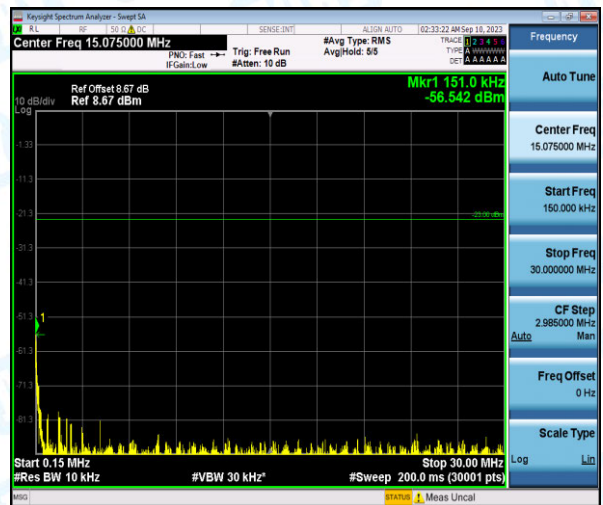
Band26-5MHz-16QAM-26740-1-0-Low-0.15-30--56.54-PASS
