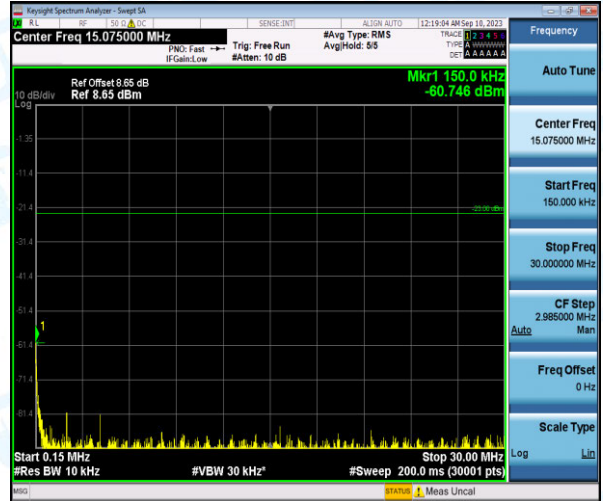
Band26-3MHz-16QAM-26705-1-0-Low-0.15-30--60.75-PASS
