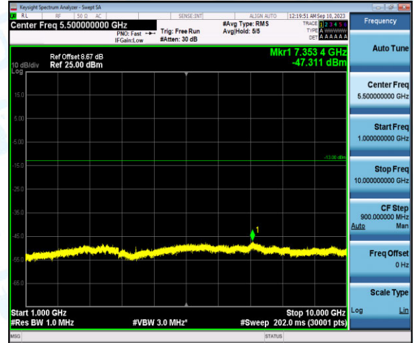
Band26-3MHz-QPSK-26740-1-0-Low-1000-10000--47.31-PASS
