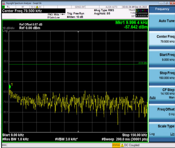
Band26-10MHz-QPSK-26740-1-0-Low-0.009-0.15--57.64-PASS
