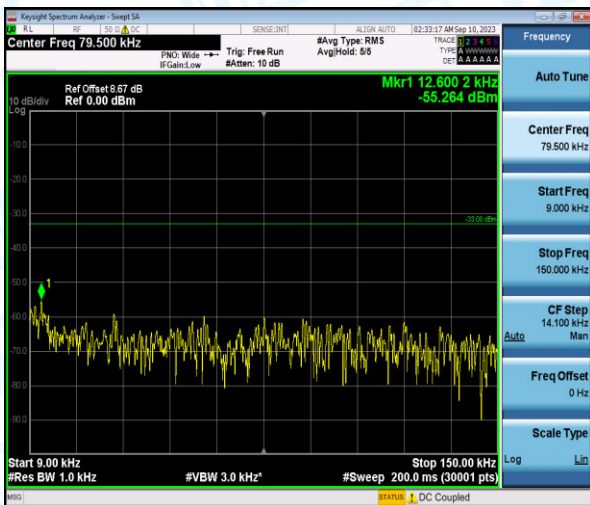
Band26-5MHz-16QAM-26740-1-0-Low-0.009-0.15--55.26-PASS
