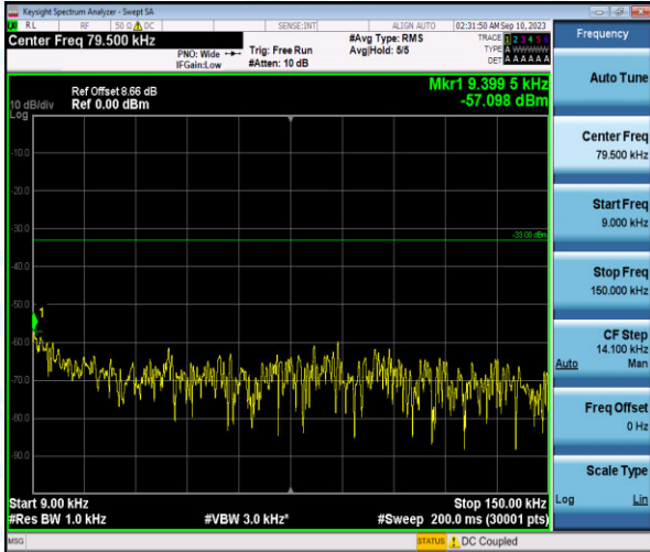
Band26-5MHz-QPSK-26715-1-0-Low-0.009-0.15--57.1-PASS
