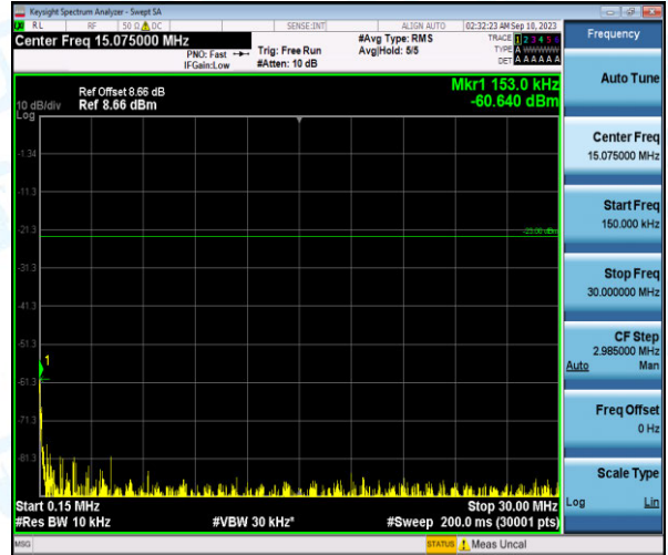
Band26-5MHz-16QAM-26715-1-0-Low-0.15-30--60.64-PASS
