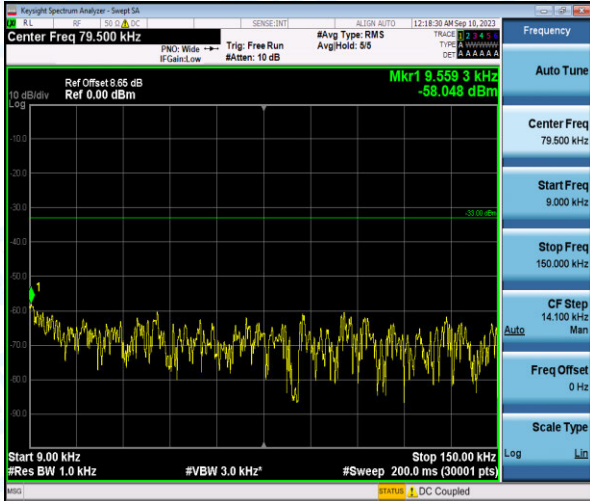
Band26-3MHz-QPSK-26705-1-0-Low-0.009-0.15--58.05-PASS
