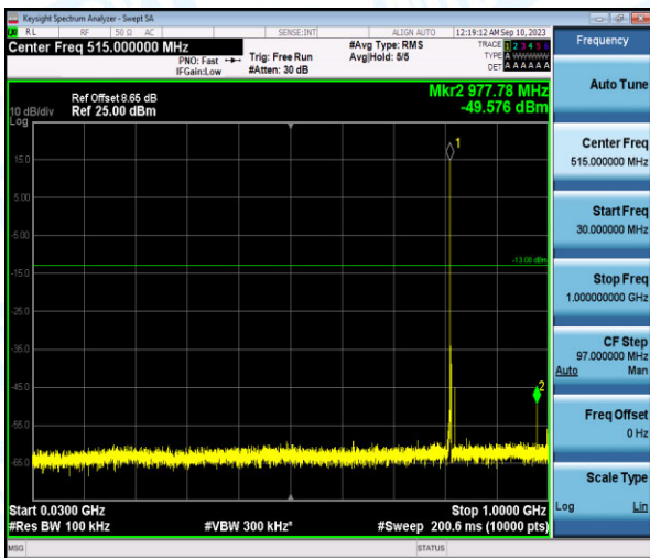
Band26-3MHz-16QAM-26705-1-0-Low-30-1000--49.58-PASS
