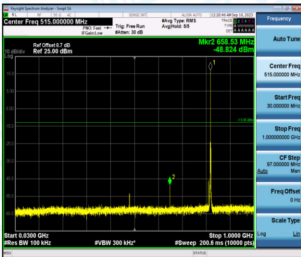
Band26-3MHz-QPSK-26775-1-0-High-30-1000--48.82-PASS
