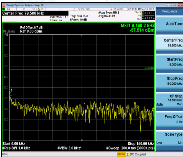
Band26-5MHz-QPSK-26785-1-0-High-0.009-0.15--57.51-PASS
