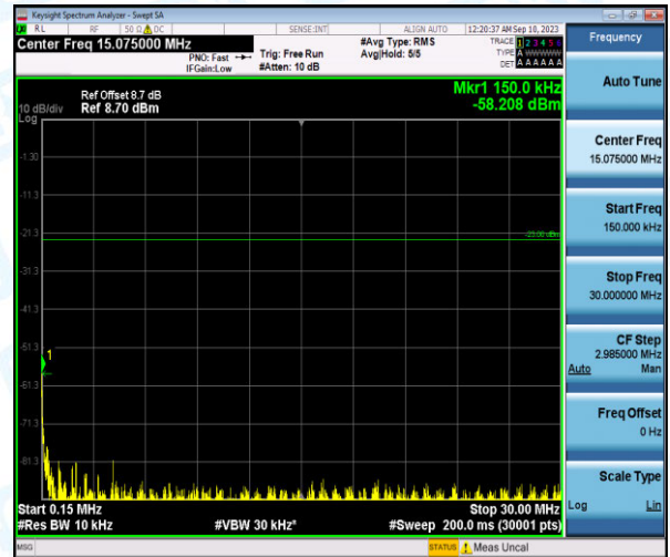
Band26-3MHz-QPSK-26775-1-0-High-0.15-30--58.21-PASS
