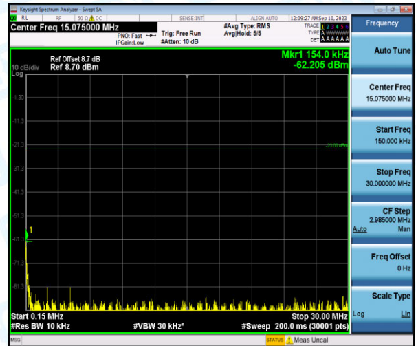
Band26-1.4MHz-QPSK-26783-1-0-High-0.15-30--62.21-PASS
