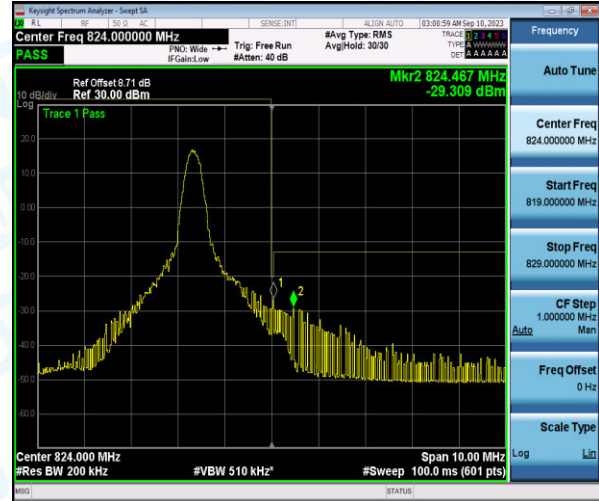
Band26-10MHz-QPSK-26740-1-0-High--26.75,-29.31-PASS
