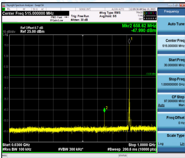
Band26-1.4MHz-QPSK-26783-1-0-High-30-1000--47.99-PASS
