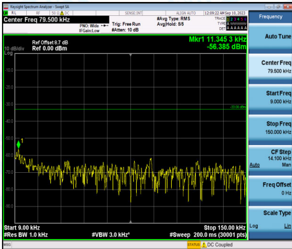
Band26-1.4MHz-QPSK-26783-1-0-High-0.009-0.15--56.39-PASS
