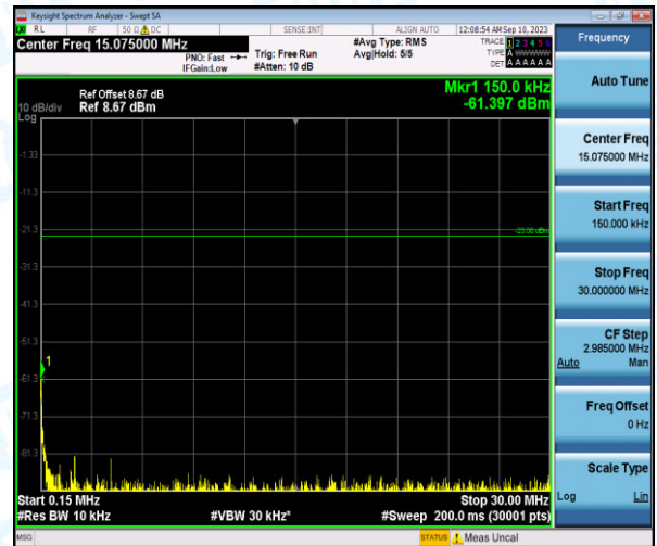
Band26-1.4MHz-16QAM-26740-1-0-Low-0.15-30--61.4-PASS
