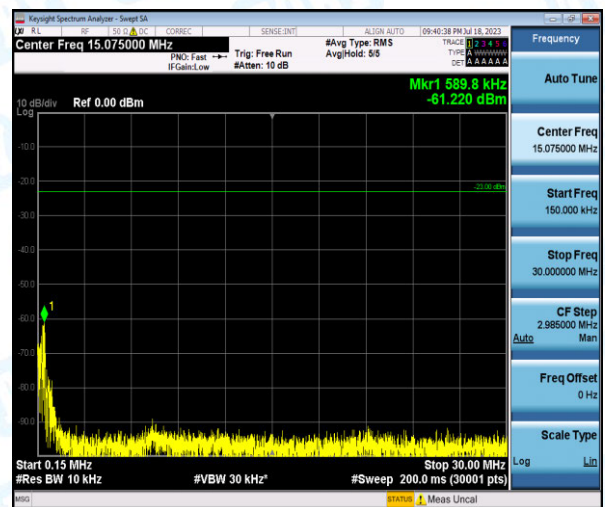
Band12-10MHz-QPSK-23095-1-0-Low-0.15-30--61.22-PASS
