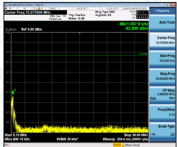
Band12-10MHz-QPSK-23130-1-0-High-0.15-30--62.9-PASS
