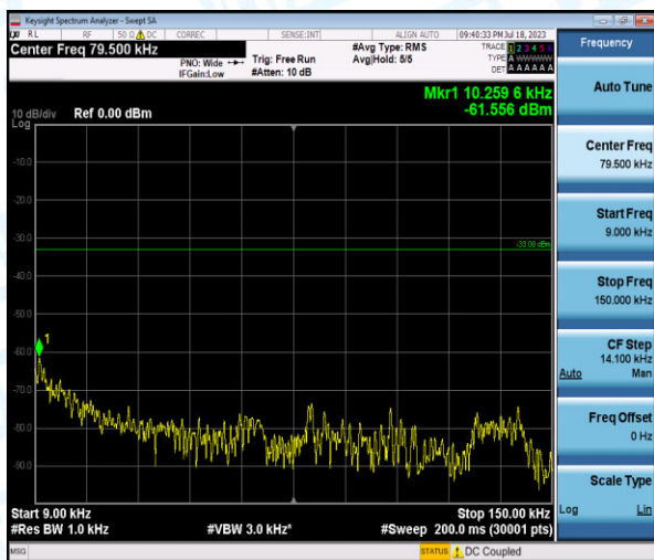
Band12-10MHz-QPSK-23095-1-0-Low-0.009-0.15--61.56-PASS
