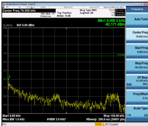
Band12-10MHz-QPSK-23130-1-0-High-0.009-0.15--62.17-PASS
