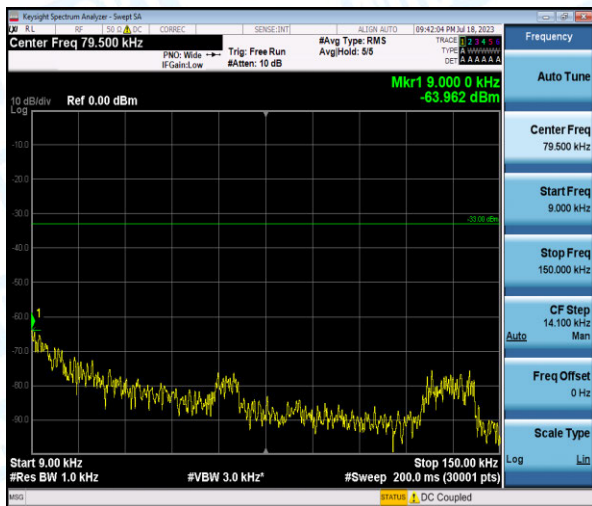
Band12-10MHz-16QAM-23130-1-0-High-0.009-0.15--63.96-PASS
