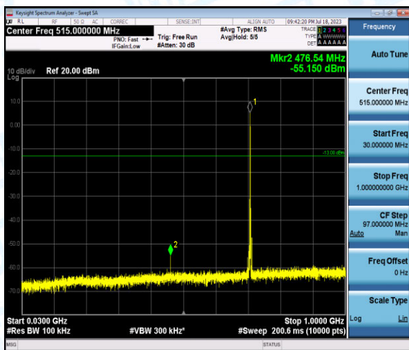
Band12-10MHz-16QAM-23130-1-0-High-30-1000--55.15-PASS
