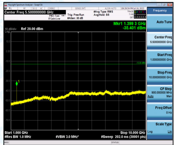
Band12-10MHz-QPSK-23060-1-0-Low-1000-10000--35.4-PASS
