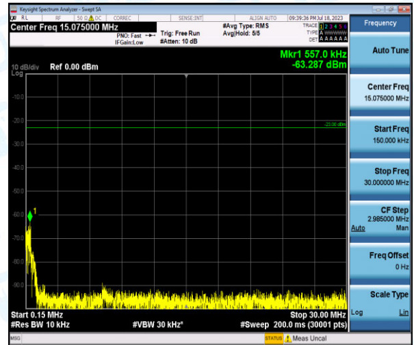
Band12-10MHz-QPSK-23060-1-0-Low-0.15-30--63.29-PASS
