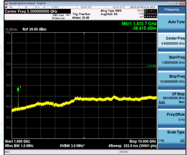
Band12-5MHz-16QAM-23095-1-0-Low-1000-10000--36.42-PASS
