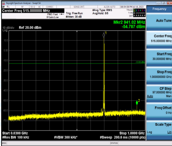
Band12-5MHz-16QAM-23095-1-0-Low-30-1000--54.79-PASS
