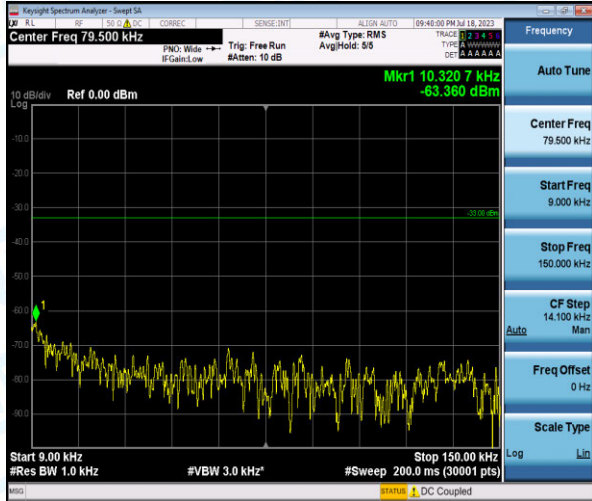
Band12-10MHz-16QAM-23060-1-0-Low-0.009-0.15--63.36-PASS
