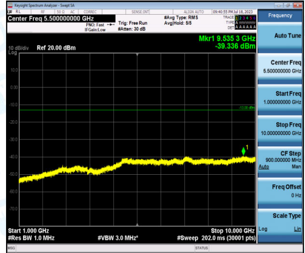
Band12-10MHz-QPSK-23095-1-0-Low-1000-10000--39.34-PASS
