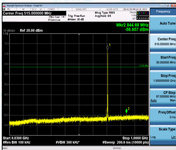
Band12-10MHz-QPSK-23130-1-0-High-30-1000--58.66-PASS
