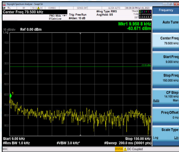
Band12-10MHz-QPSK-23060-1-0-Low-0.009-0.15--63.67-PASS
