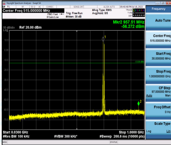
Band12-10MHz-QPSK-23095-1-0-Low-30-1000--56.27-PASS
