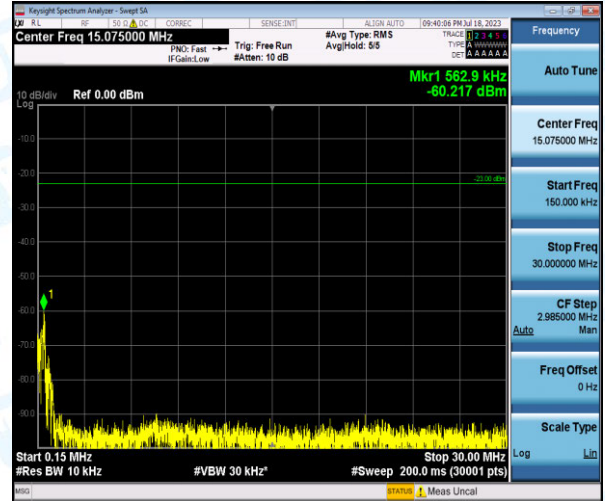
Band12-10MHz-16QAM-23060-1-0-Low-0.15-30--60.22-PASS
