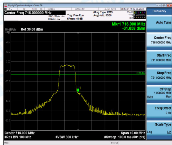
Band12-5MHz-16QAM-23155-6-0-High--31.66-PASS
