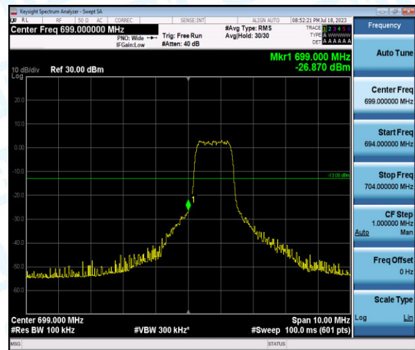
Band12-5MHz-16QAM-23035-6-0-Low--26.87-PASS
