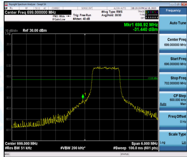
Band12-3MHz-QPSK-23025-6-0-Low--31.44-PASS
