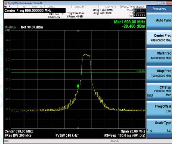
Band12-10MHz-QPSK-23060-6-0-Low--29.46-PASS
