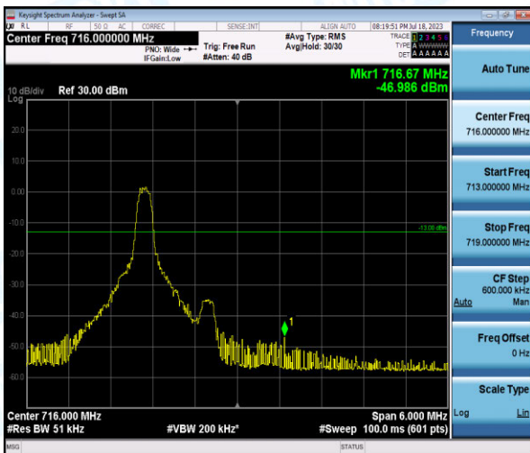
Band12-3MHz-16QAM-23165-1-0-High--46.99-PASS
