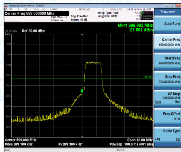
Band12-5MHz-QPSK-23035-6-0-Low--27.69-PASS
