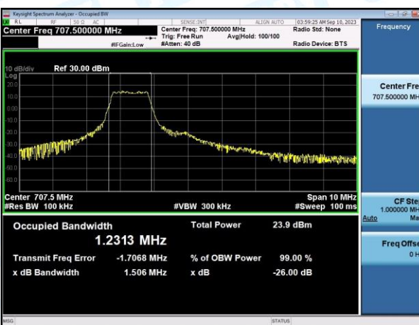
Band12-10MHz-16QAM-23095-6-0-Low-1.2313-12.03-PASS
