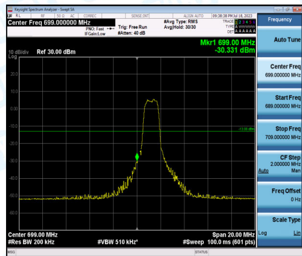
Band12-10MHz-16QAM-23060-6-0-Low--30.33-PASS
