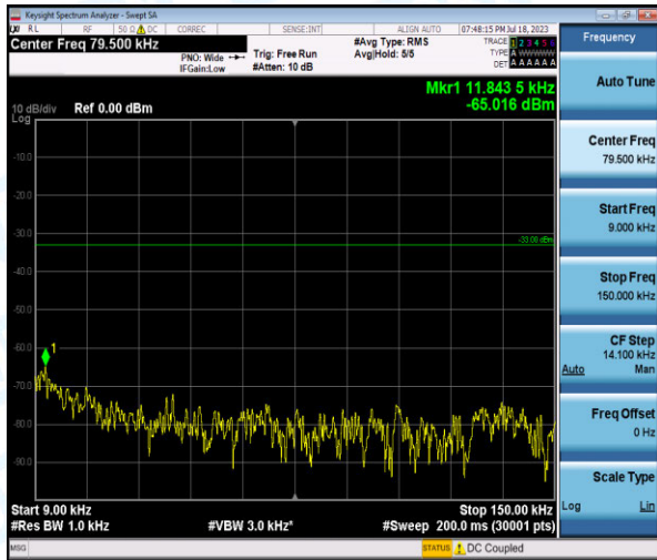
Band12-1.4MHz-QPSK-23017-1-0-Low-0.009-0.15-65.02-PASS
