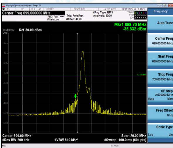
Band12-10MHz-16QAM-23060-1-0-Low--35.83-PASS
