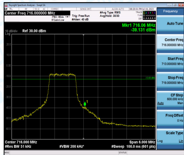
Band12-3MHz-QPSK-23165-6-0-High--39.13-PASS
