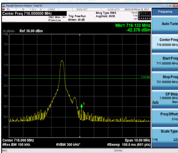
Band12-5MHz-16QAM-23155-1-0-High--42.38-PASS
