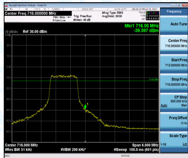
Band12-3MHz-16QAM-23165-6-0-High--39.60-PASS
