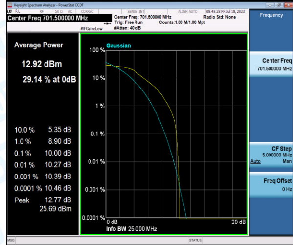
Band12-5MHz-16QAM-23035-6-0-Low-10.00-<=13-PASS
