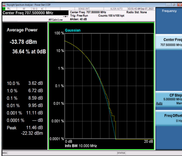
Band12-3MHz-QPSK-23095-1-0-Low-8.59-<=13-PASS
