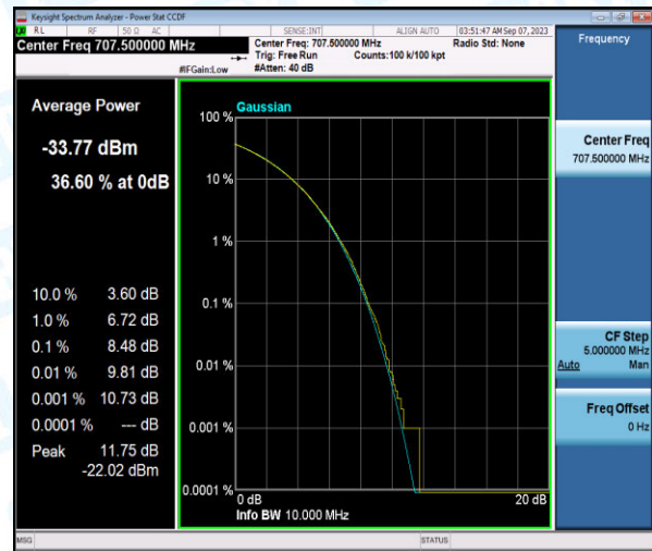
Band12-3MHz-QPSK-23095-6-0-Low-8.48-<=13-PASS
