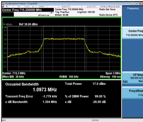
Band12-1.4MHz-QPSK-23173-6-0-High-1.0973-1.304-PASS
