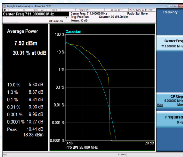
Band12-10MHz-QPSK-23130-1-0-High-9.81-<=13-PASS
