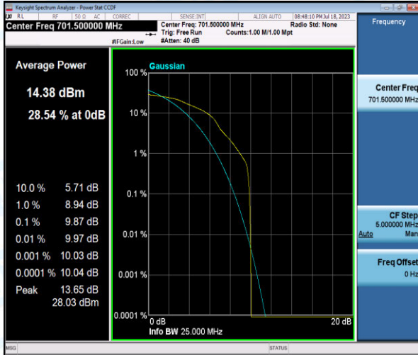
Band12-5MHz-16QAM-23035-1-0-Low-9.87-<=13-PASS
