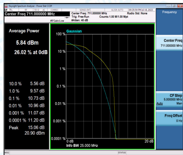
Band12-10MHz-QPSK-23130-6-0-High-10.73-<=13-PASS
