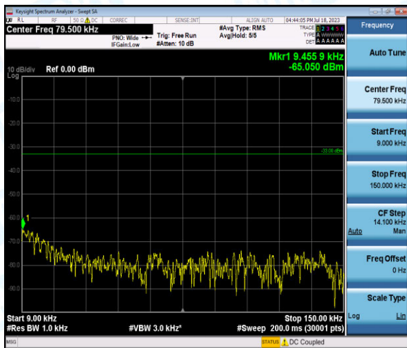
Band5-3MHz-QPSK-20635-1-0-High-0.009-0.15--65.05-PASS
