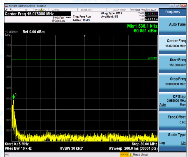
Band5-3MHz-16QAM-20525-1-0-Low-0.15-30--60.85-PASS
