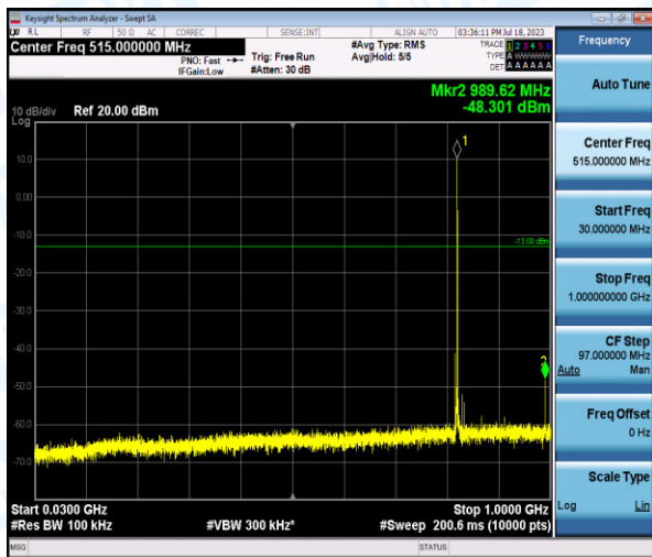
Band5-1.4MHz-16QAM-20407-1-0-Low-30-1000--48.3-PASS
