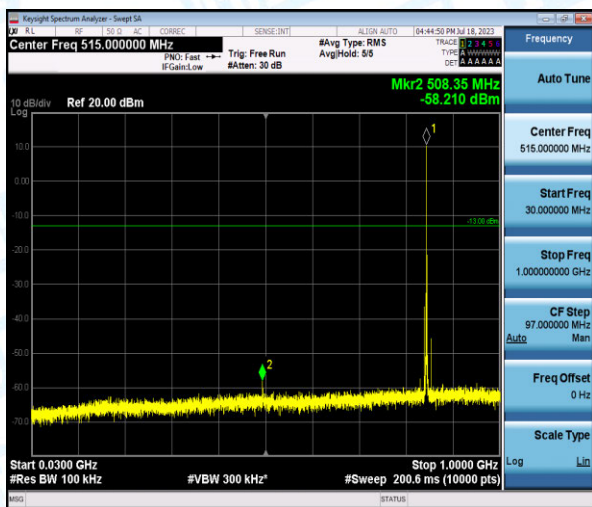
Band5-3MHz-16QAM-20635-1-0-High-30-1000--58.21-PASS
