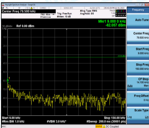
Band5-5MHz-QPSK-20525-1-0-Low-0.009-0.15--62.06-PASS
