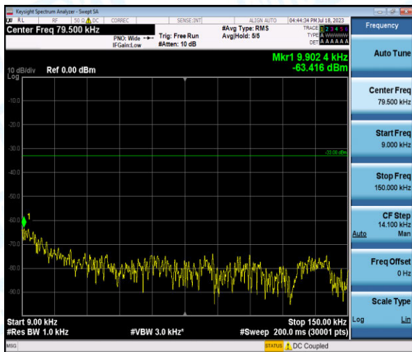
Band5-3MHz-16QAM-20635-1-0-High-0.009-0.15--63.42-PASS
