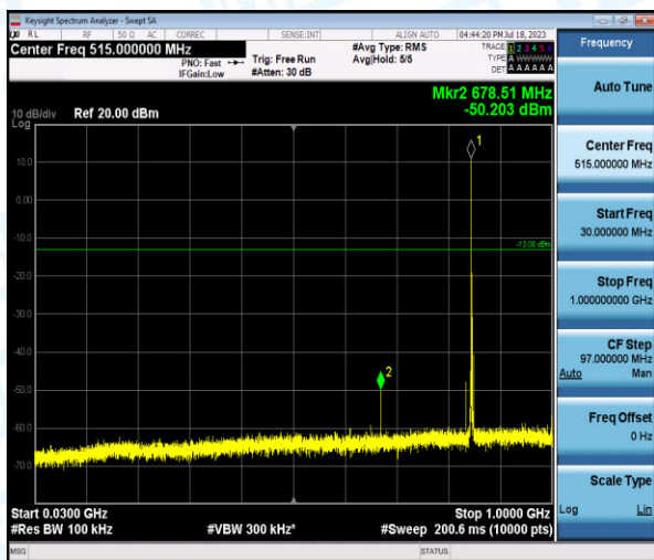
Band5-3MHz-QPSK-20635-1-0-High-30-1000--50.2-PASS
