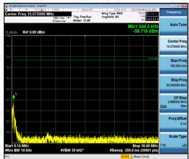
Band5-1.4MHz-16QAM-20525-1-0-Low-0.15-30--59.72-PASS
