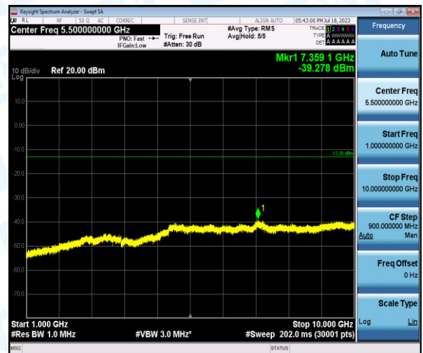
Band5-5MHz-QPSK-20425-1-0-Low-1000-10000--39.28-PASS
