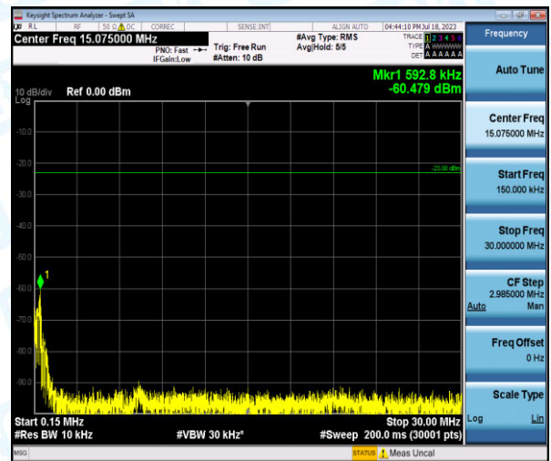
Band5-3MHz-QPSK-20635-1-0-High-0.15-30--60.48-PASS
