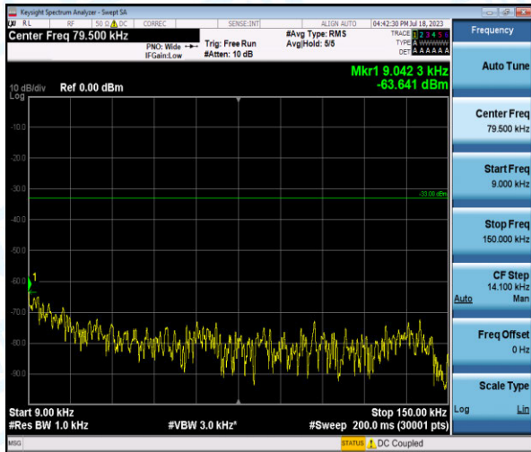
Band5-3MHz-16QAM-20415-1-0-Low-0.009-0.15--63.64-PASS
