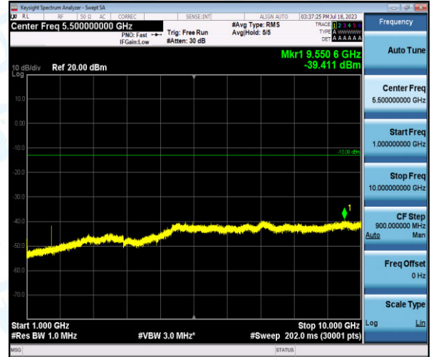
Band5-1.4MHz-16QAM-20525-1-0-Low-1000-10000--39.41-PASS
