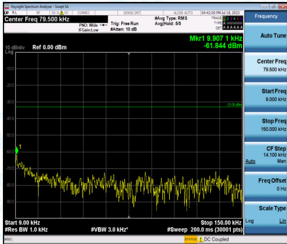
Band5-3MHz-QPSK-20415-1-0-Low-0.009-0.15--61.84-PASS
