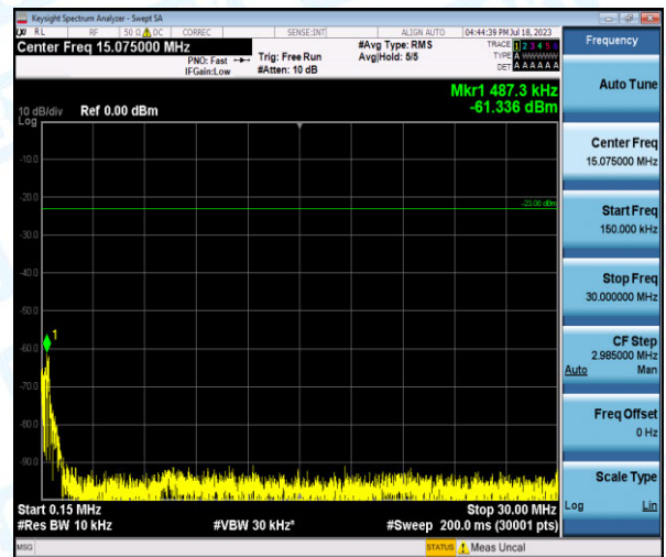
Band5-3MHz-16QAM-20635-1-0-High-0.15-30--61.34-PASS
