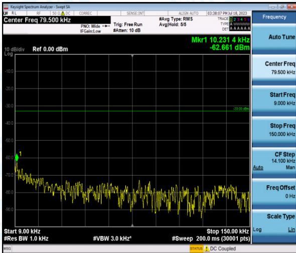
Band5-1.4MHz-16QAM-20643-1-0-High-0.009-0.15--62.66-PASS
