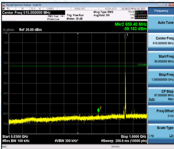
Band5-1.4MHz-16QAM-20643-1-0-High-30-1000--59.18-PASS
