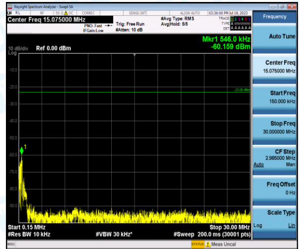
Band5-1.4MHz-16QAM-20407-1-0-Low-0.15-30--60.16-PASS
