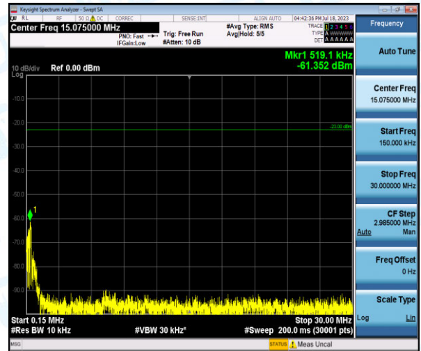
Band5-3MHz-16QAM-20415-1-0-Low-0.15-30--61.35-PASS
