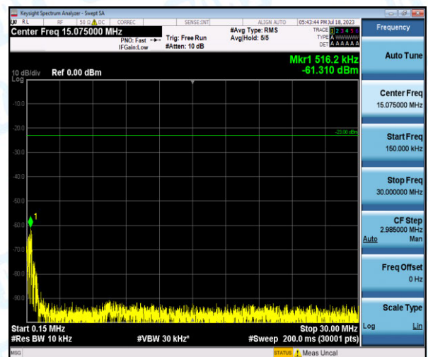
Band5-5MHz-QPSK-20525-1-0-Low-0.15-30--61.31-PASS
