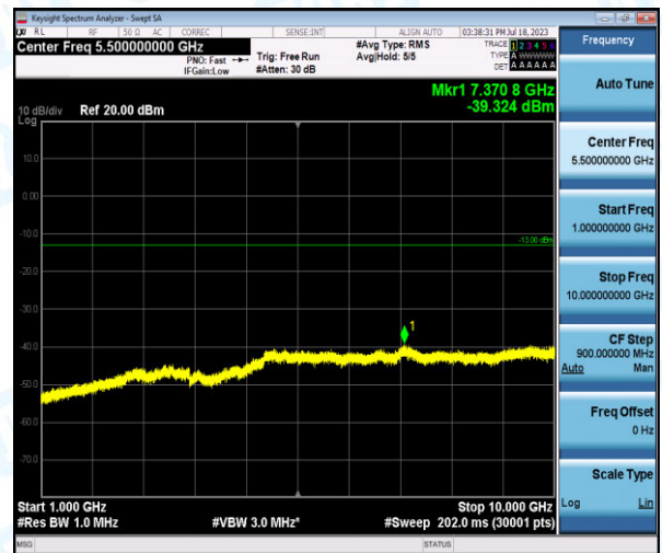
Band5-1.4MHz-16QAM-20643-1-0-High-1000-10000--39.32-PASS
