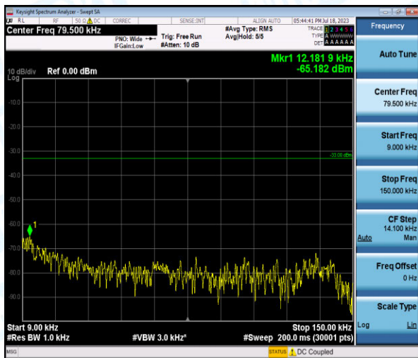
Band5-5MHz-QPSK-20625-1-0-High-0.009-0.15--65.18-PASS
