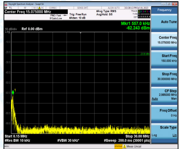
Band5-1.4MHz-16QAM-20643-1-0-High-0.15-30--62.24-PASS
