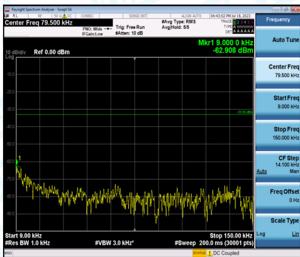
Band5-3MHz-QPSK-20525-1-0-Low-0.009-0.15--62.91-PASS
