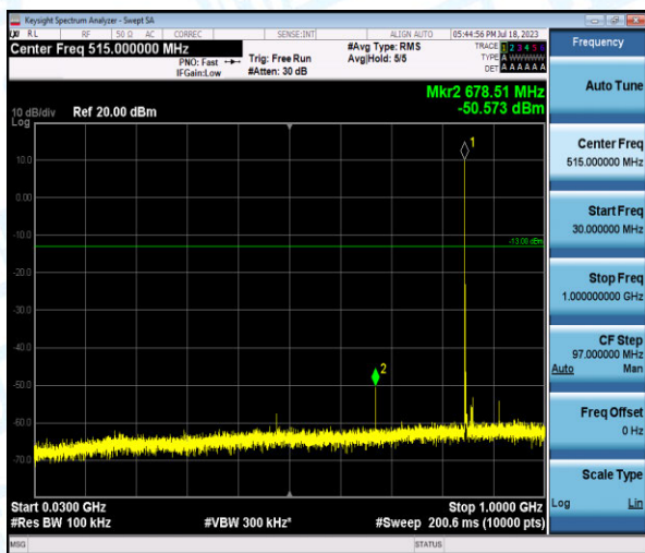
Band5-5MHz-QPSK-20625-1-0-High-30-1000--50.57-PASS
