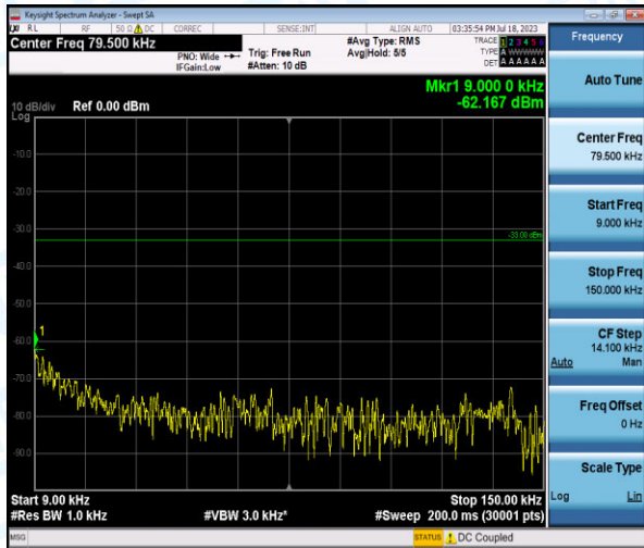
Band5-1.4MHz-16QAM-20407-1-0-Low-0.009-0.15--62.17-PASS
