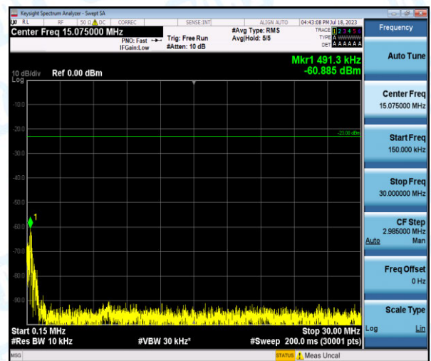
Band5-3MHz-QPSK-20525-1-0-Low-0.15-30--60.89-PASS
