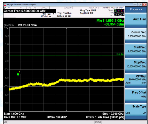
Band5-5MHz-QPSK-20625-1-0-High-1000-10000--38.35-PASS
