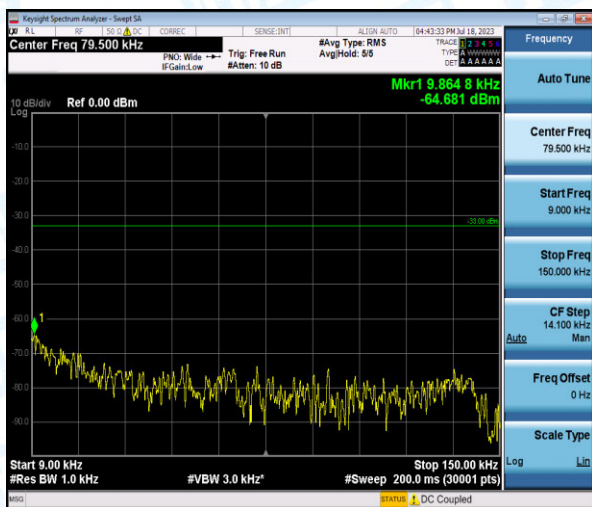
Band5-3MHz-16QAM-20525-1-0-Low-0.009-0.15--64.68-PASS
