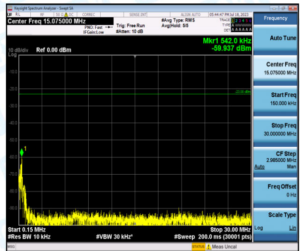
Band5-5MHz-QPSK-20625-1-0-High-0.15-30--59.94-PASS
