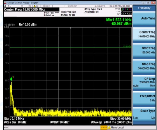
Band5-5MHz-QPSK-20425-1-0-Low-0.15-30--60.97-PASS
