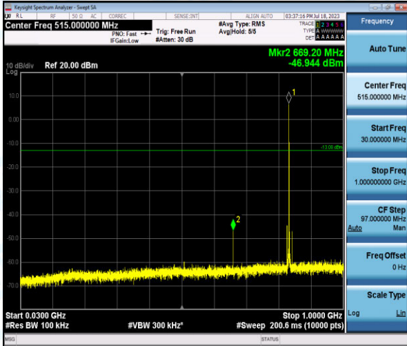
Band5-1.4MHz-16QAM-20525-1-0-Low-30-1000--46.94-PASS
