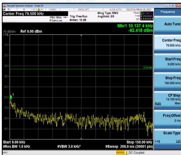
Band5-1.4MHz-16QAM-20525-1-0-Low-0.009-0.15--62.42-PASS
