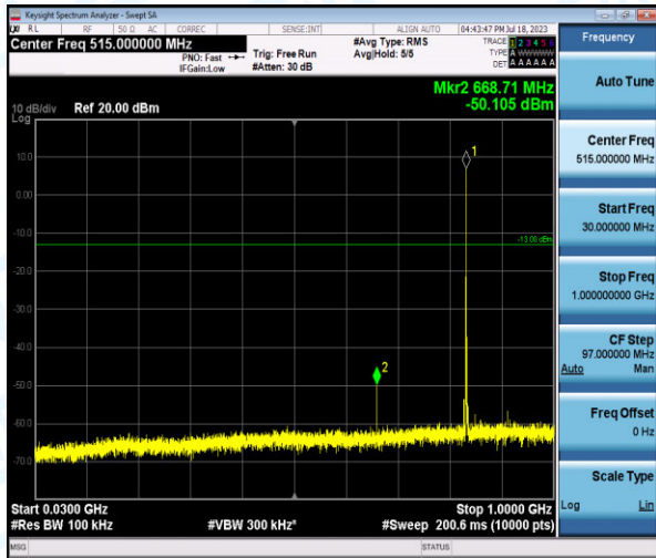
Band5-3MHz-16QAM-20525-1-0-Low-30-1000--50.11-PASS
