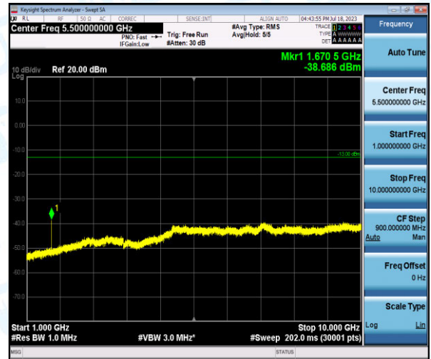
Band5-3MHz-16QAM-20525-1-0-Low-1000-10000--38.69-PASS
