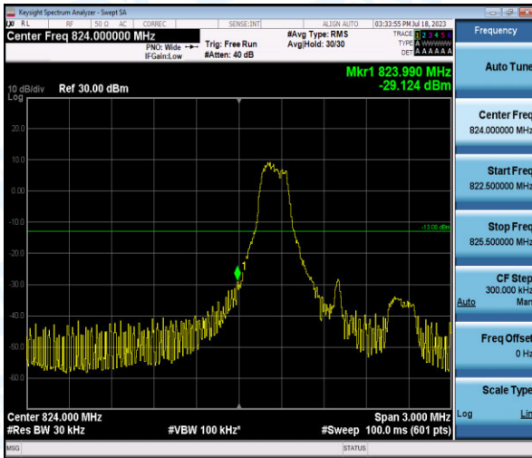
Band5-1.4MHz-QPSK-20407-1-0-Low--29.12-PASS
