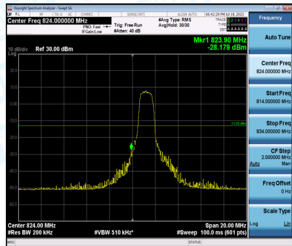
Band5-10MHz-16QAM-20450-6-0-Low--28.18-PASS
