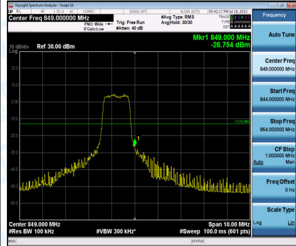
Band5-5MHz-QPSK-20625-6-0-High--26.75-PASS
