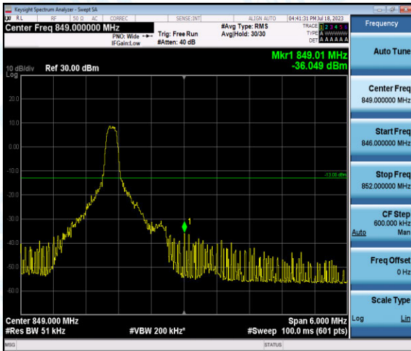
Band5-3MHz-16QAM-20635-1-0-High--36.05-PASS
