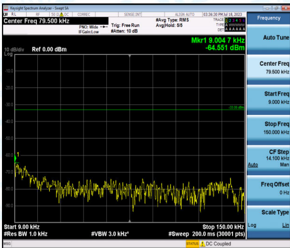
Band5-1.4MHz-QPSK-20525-1-0-Low-0.009-0.15--64.55-PASS
