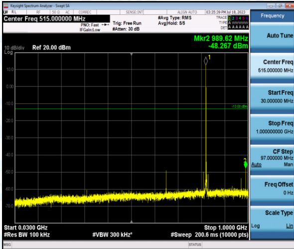
Band5-1.4MHz-QPSK-20407-1-0-Low-30-1000--48.27-PASS
