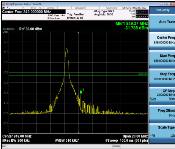
Band5-10MHz-QPSK-20600-1-0-High--31.78-PASS
