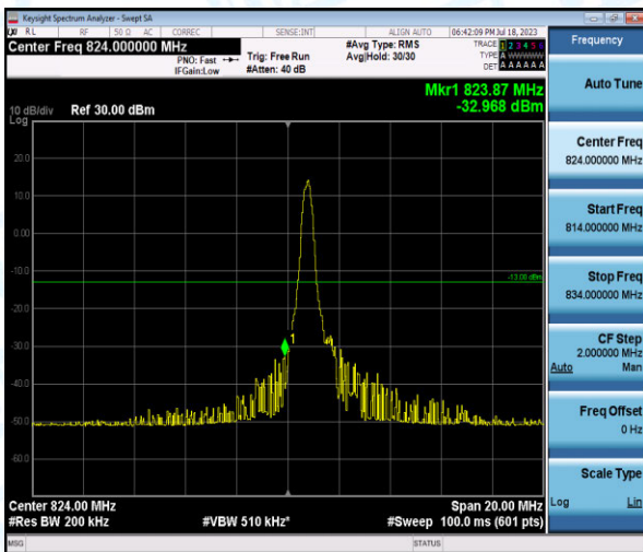
Band5-10MHz-16QAM-20450-1-0-Low--32.97-PASS
