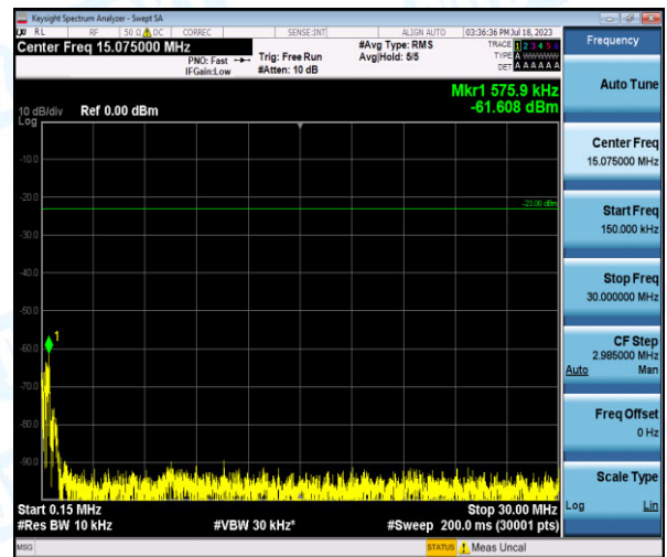
Band5-1.4MHz-QPSK-20525-1-0-Low-0.15-30--61.61-PASS
