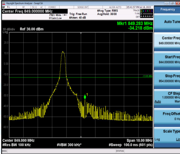
Band5-5MHz-QPSK-20625-1-0-High--34.22-PASS
