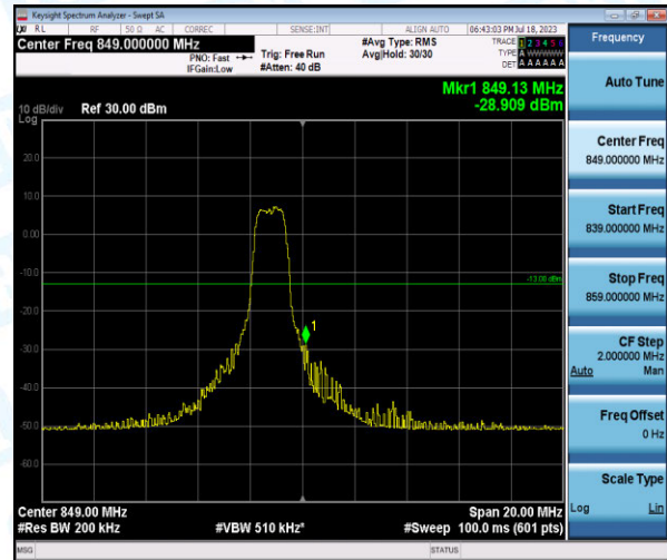
Band5-10MHz-QPSK-20600-6-0-High--28.91-PASS
