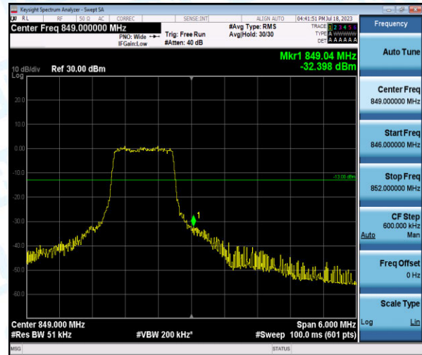
Band5-3MHz-16QAM-20635-6-0-High--32.40-PASS
