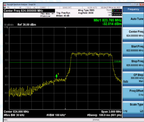
Band5-1.4MHz-16QAM-20407-6-0-Low--32.01-PASS
