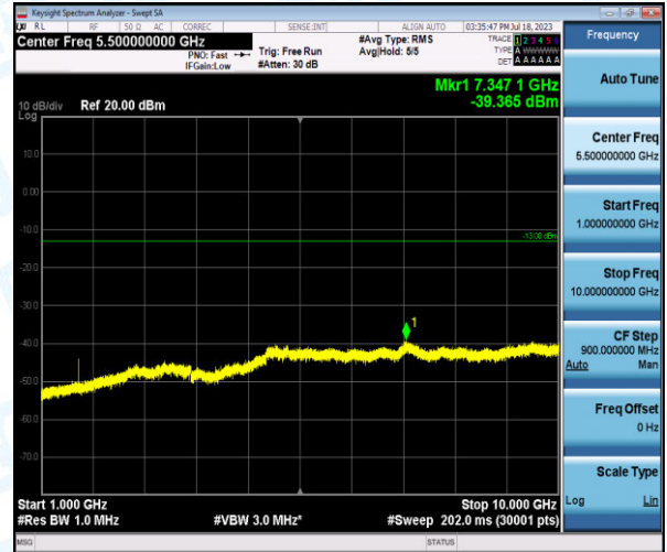
Band5-1.4MHz-QPSK-20407-1-0-Low-1000-10000--39.37-PASS
