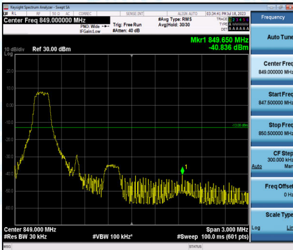
Band5-1.4MHz-QPSK-20643-1-0-High--40.84-PASS
