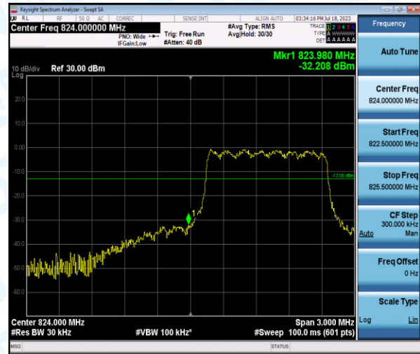
Band5-1.4MHz-QPSK-20407-6-0-Low--32.21-PASS
