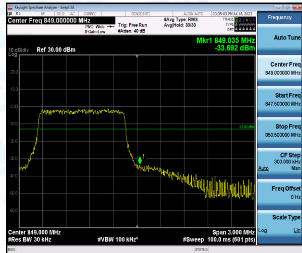
Band5-1.4MHz-QPSK-20643-6-0-High--33.69-PASS
