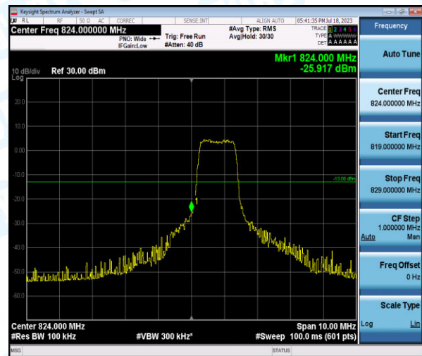
Band5-5MHz-QPSK-20425-6-0-Low--25.92-PASS
