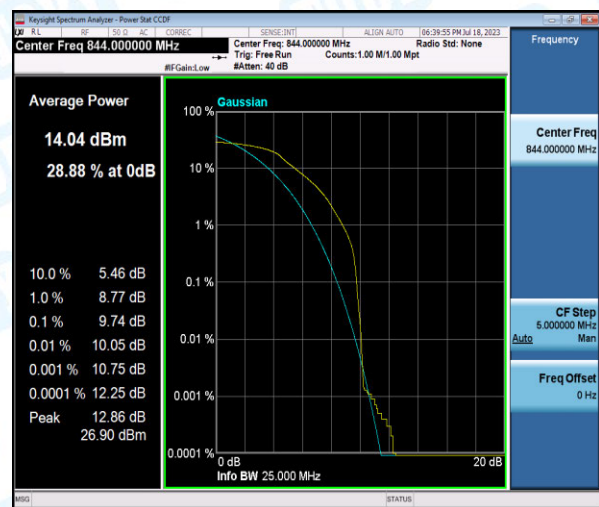
Band5-10MHz-16QAM-20600-6-0-High-9.74-<=13-PASS
