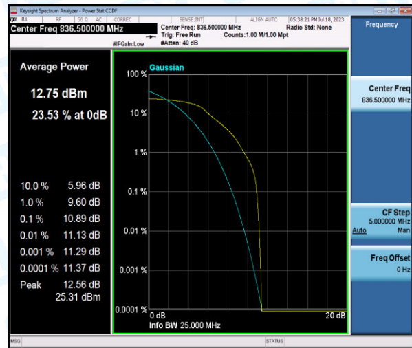
Band5-5MHz-QPSK-20525-6-0-Low-10.89-<=13-PASS
