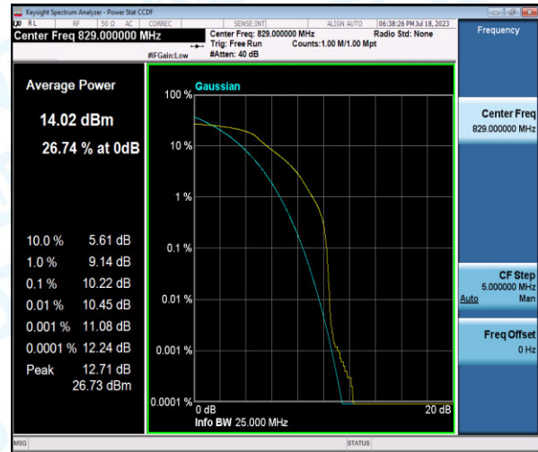
Band5-10MHz-QPSK-20450-6-0-Low-10.22-<=13-PASS
