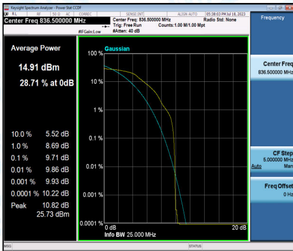
Band5-5MHz-QPSK-20525-1-0-Low-9.71-<=13-PASS
