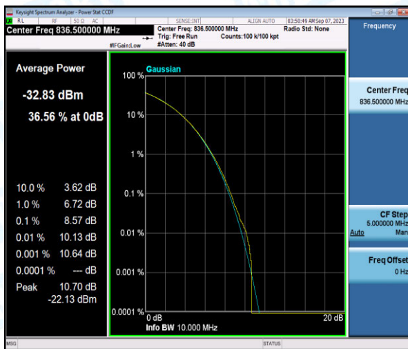
Band5-3MHz-QPSK-20525-1-0-Low-8.57-<=13-PASS
