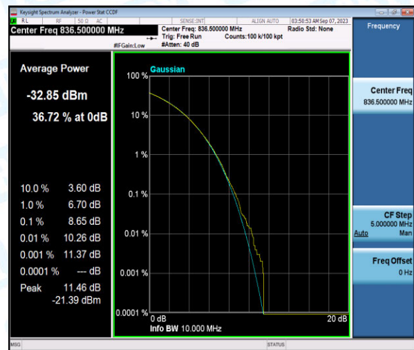
Band5-3MHz-QPSK-20525-6-0-Low-8.65-<=13-PASS
