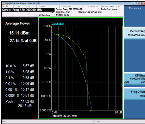
Band5-10MHz-QPSK-20450-1-0-Low-9.88-<=13-PASS
