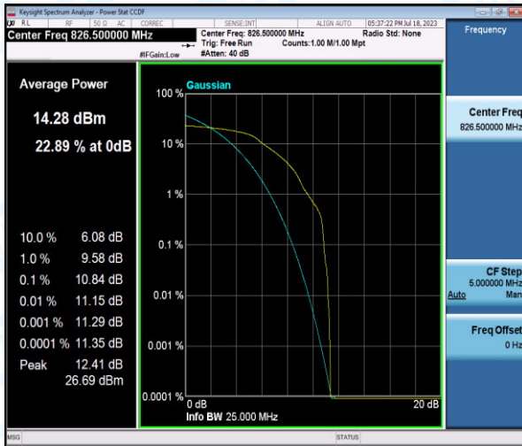
Band5-5MHz-QPSK-20425-1-0-Low-10.84-<=13-PASS
