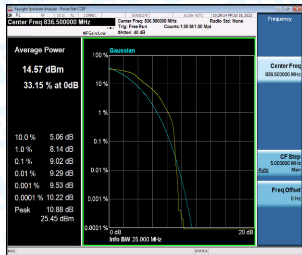
Band5-10MHz-16QAM-20525-6-0-Low-9.02-<=13-PASS
