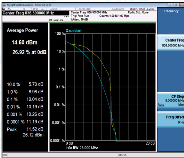
Band5-10MHz-QPSK-20525-1-0-Low-10.04-<=13-PASS
