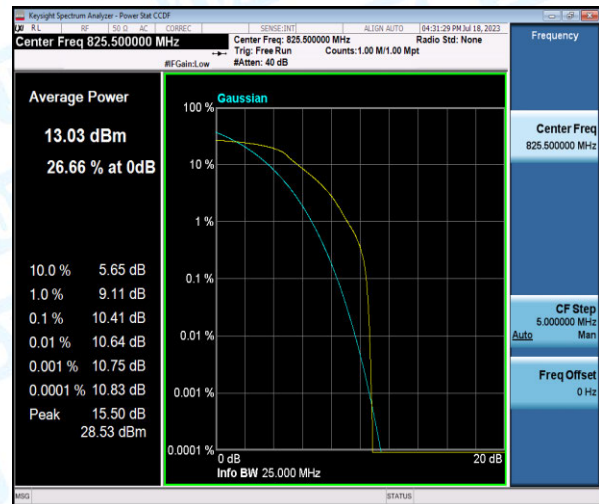
Band5-3MHz-QPSK-20415-6-0-Low-10.41-<=13-PASS
