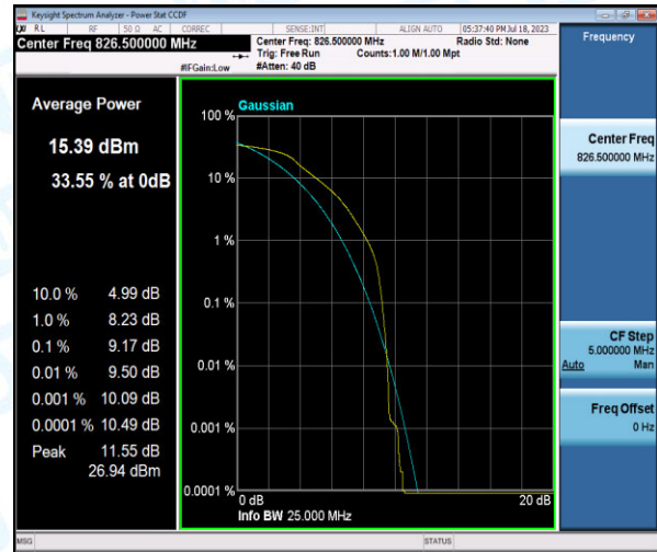
Band5-5MHz-QPSK-20425-6-0-Low-9.17-<=13-PASS
