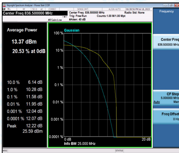
Band5-10MHz-16QAM-20525-1-0-Low-11.58-<=13-PASS
