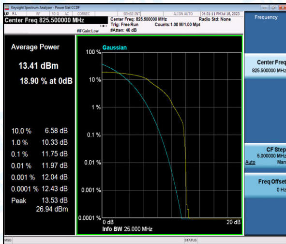
Band5-3MHz-QPSK-20415-1-0-Low-11.75-<=13-PASS
