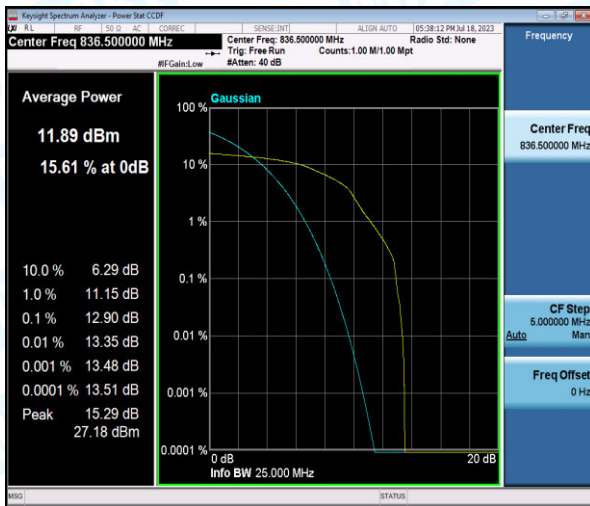
Band5-5MHz-16QAM-20525-1-0-Low-12.90-<=13-PASS
