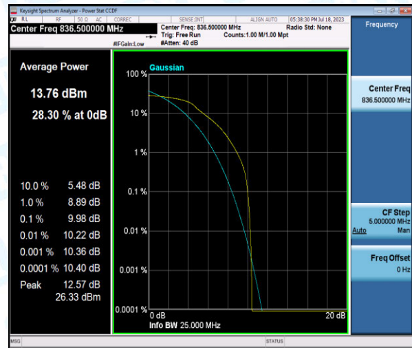
Band5-5MHz-16QAM-20525-6-0-Low-9.98-<=13-PASS
