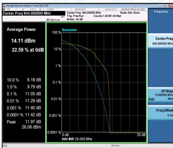
Band5-10MHz-16QAM-20600-1-0-High-11.05-<=13-PASS
