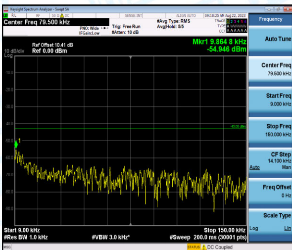
Band4-15MHz-16QAM-20175-1-0-Low-0.009-0.15--54.95-PASS
