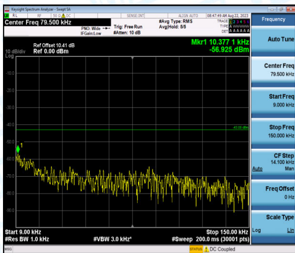
Band4-10MHz-16QAM-20175-1-0-Low-0.009-0.15--56.93-PASS
