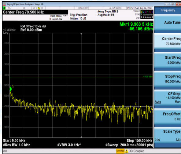
Band4-20MHz-QPSK-20050-1-0-Low-0.009-0.15-56.16-PASS
