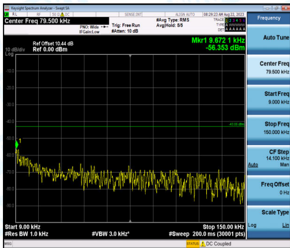
Band4-5MHz-16QAM-20375-1-0-High-0.009-0.15--56.35-PASS
