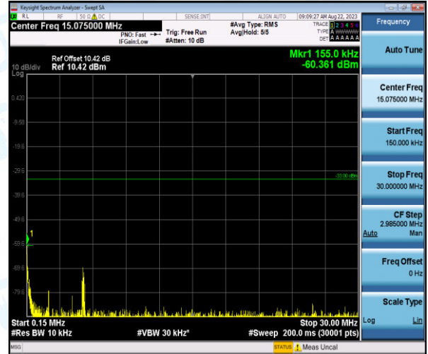
Band4-15MHz-16QAM-20025-1-0-Low-0.15-30--60.36-PASS
