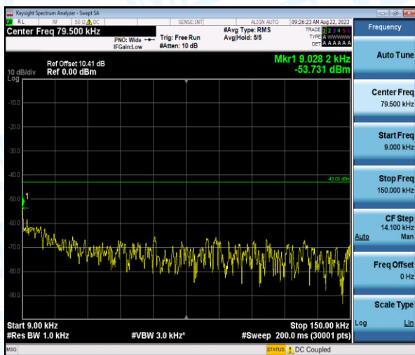
Band4-20MHz-QPSK-20175-1-0-Low-0.009-0.15-53.73-PASS
