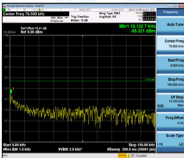
Band4-10MHz-QPSK-20175-1-0-Low-0.009-0.15-55.32-PASS
