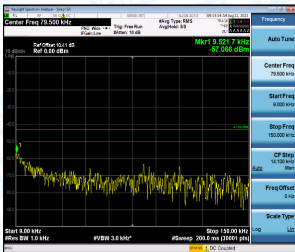
Band4-15MHz-QPSK-20175-1-0-Low-0.009-0.15-57.07-PASS
