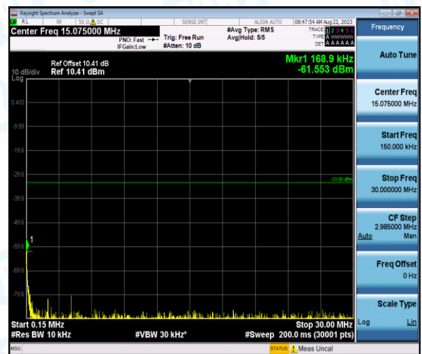
Band4-10MHz-16QAM-20175-1-0-Low-0.15-30--61.55-PASS
