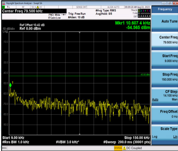
Band4-15MHz-16QAM-20025-1-0-Low-0.009-0.15--54.57-PASS
