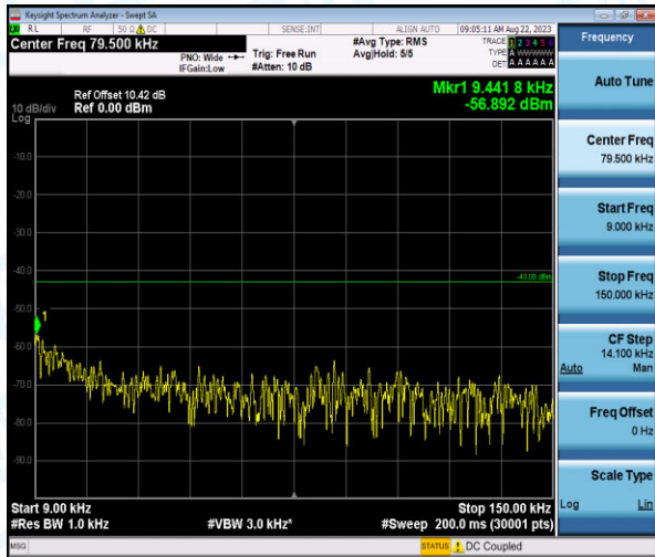
Band4-15MHz-QPSK-20025-1-0-Low-0.009-0.15-56.89-PASS
