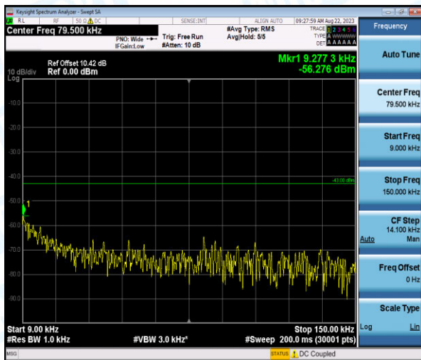
Band4-20MHz-QPSK-20300-1-0-High-0.009-0.15--56.28-PASS
