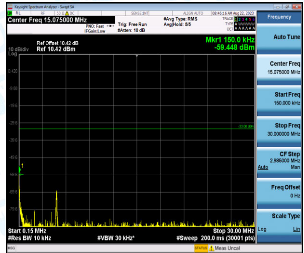
Band4-10MHz-QPSK-20000-1-0-Low-0.15-30--59.45-PASS
