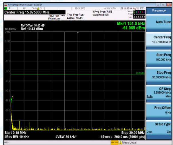
Band4-15MHz-16QAM-20325-1-0-High-0.15-30--61.07-PASS
