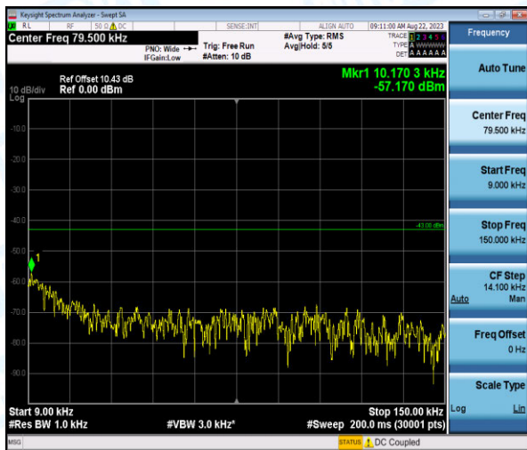
Band4-15MHz-QPSK-20325-1-0-High-0.009-0.15--57.17-PASS
