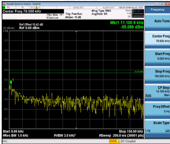
Band4-5MHz-QPSK-19975-1-0-Low-0.009-0.15--55.07-PASS
