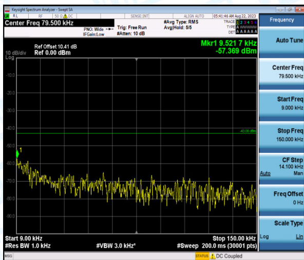
Band4-1.4MHz-16QAM-20175-1-0-Low-0.009-0.15--57.37-PASS
