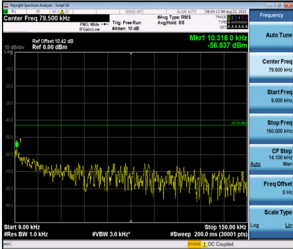
Band4-3MHz-16QAM-19965-1-0-Low-0.009-0.15--56.84-PASS
