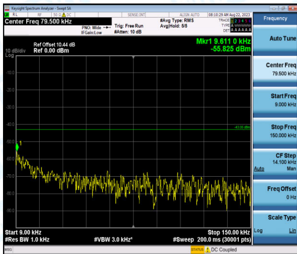
Band4-3MHz-16QAM-20385-1-0-High-0.009-0.15--55.83-PASS
