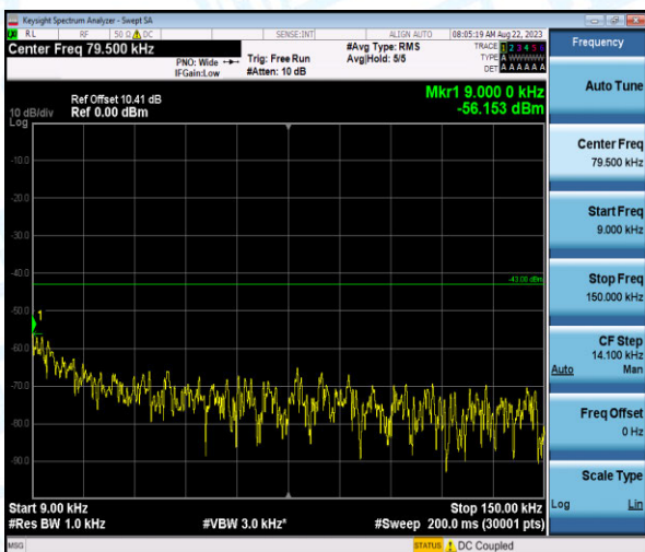
Band4-3MHz-16QAM-20175-1-0-Low-0.009-0.15--56.15-PASS
