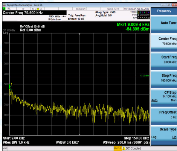
Band4-1.4MHz-QPSK-20393-1-0-High-0.009-0.15--54.9-PASS
