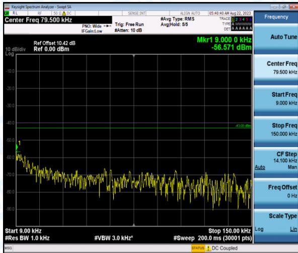
Band4-1.4MHz-16QAM-19957-1-0-Low-0.009-0.15--56.57-PASS
