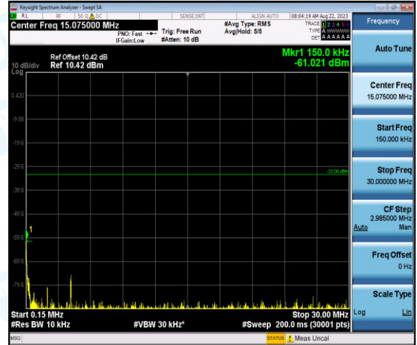
Band4-3MHz-16QAM-19965-1-0-Low-0.15-30--61.02-PASS
