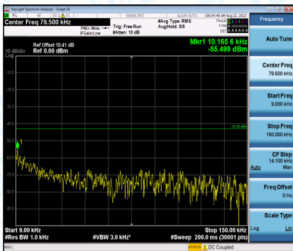
Band4-3MHz-QPSK-20175-1-0-Low-0.009-0.15--55.5-PASS
