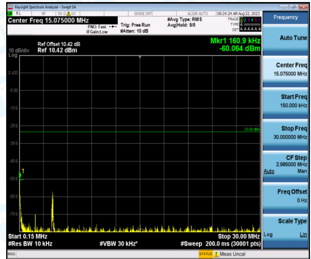
Band4-5MHz-QPSK-19975-1-0-Low-0.15-30--60.06-PASS
