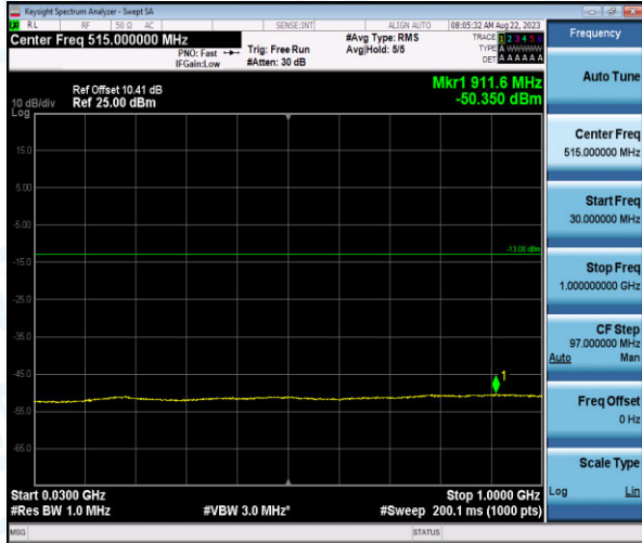
Band4-3MHz-16QAM-20175-1-0-Low-30-1000--50.35-PASS
