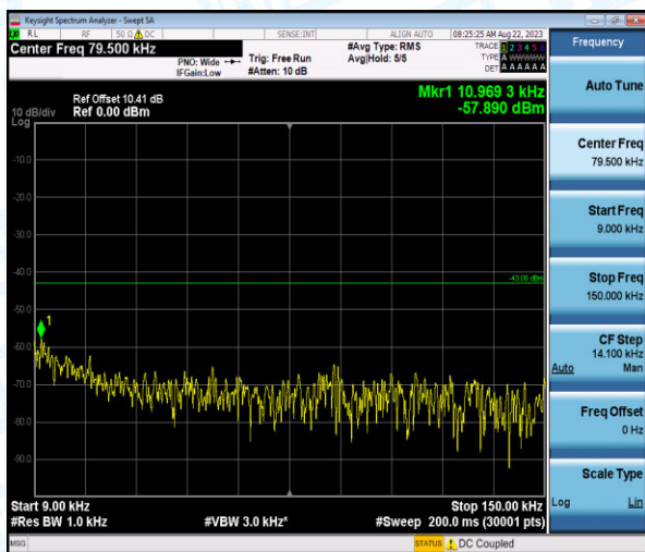
Band4-5MHz-QPSK-20175-1-0-Low-0.009-0.15--57.89-PASS
