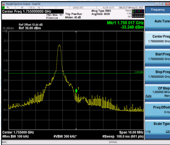
Band4-5MHz-QPSK-20375-1-0-High--33.25-PASS
