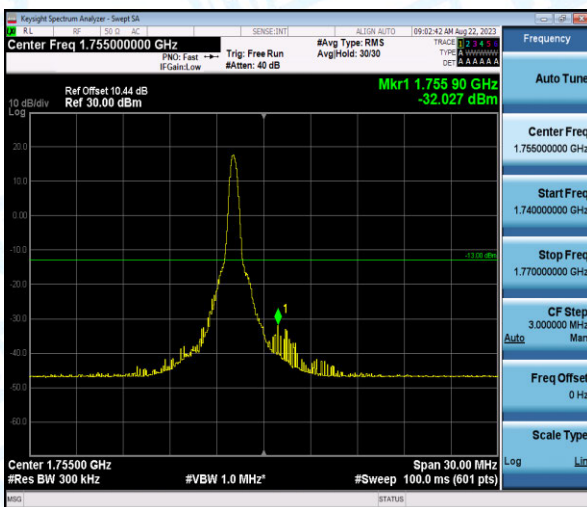
Band4-15MHz-QPSK-20325-1-0-High--32.03-PASS
