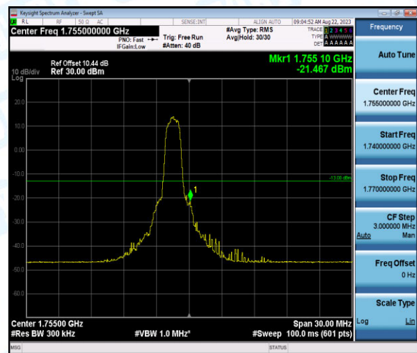
Band4-15MHz-QPSK-20325-6-0-High--21.47-PASS
