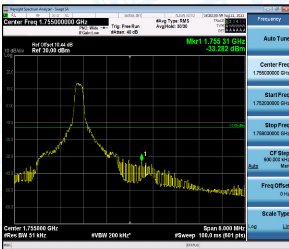
Band4-3MHz-QPSK-20385-1-0-High--33.28-PASS
