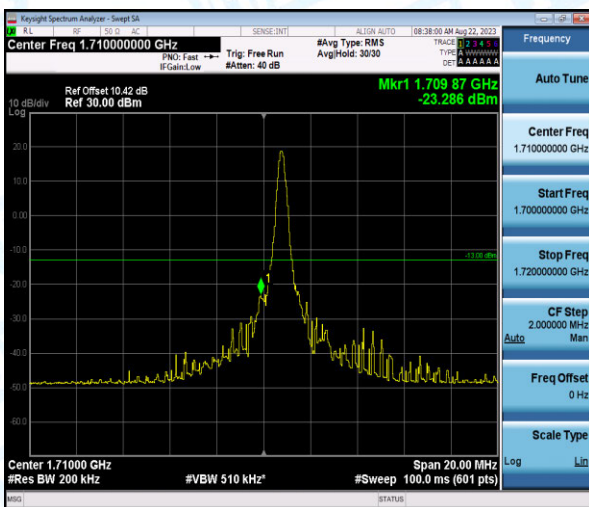
Band4-10MHz-16QAM-20000-1-0-Low--23.29-PASS
