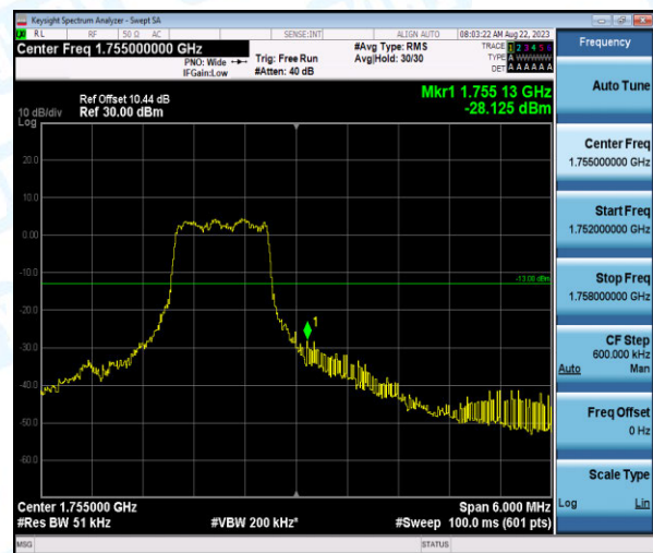
Band4-3MHz-QPSK-20385-6-0-High--28.12-PASS
