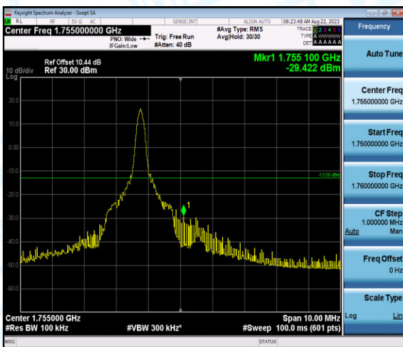
Band4-5MHz-16QAM-20375-1-0-High--29.42-PASS
