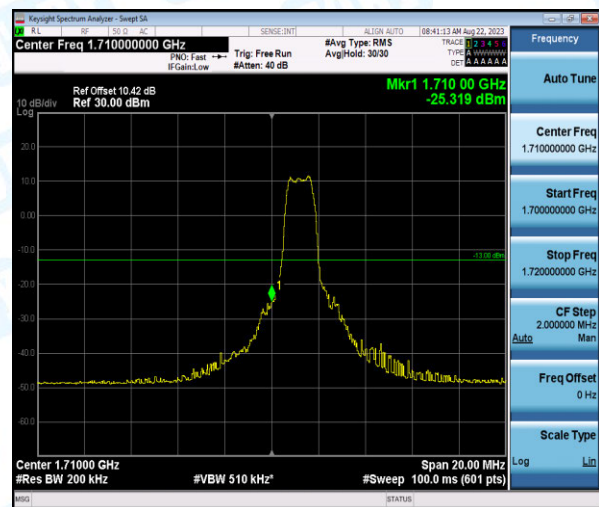
Band4-10MHz-16QAM-20000-6-0-Low--25.32-PASS
