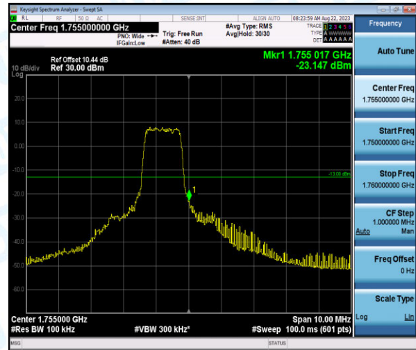
Band4-5MHz-QPSK-20375-6-0-High--23.15-PASS
