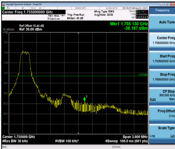
Band4-1.4MHz-QPSK-20393-1-0-High--38.20-PASS
