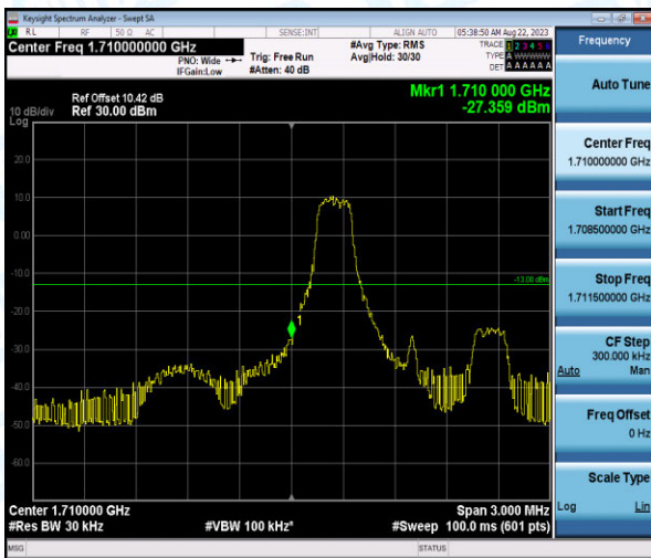
Band4-1.4MHz-16QAM-19957-1-0-Low--27.36-PASS
