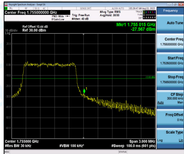
Band4-1.4MHz-QPSK-20393-6-0-High--27.57-PASS
