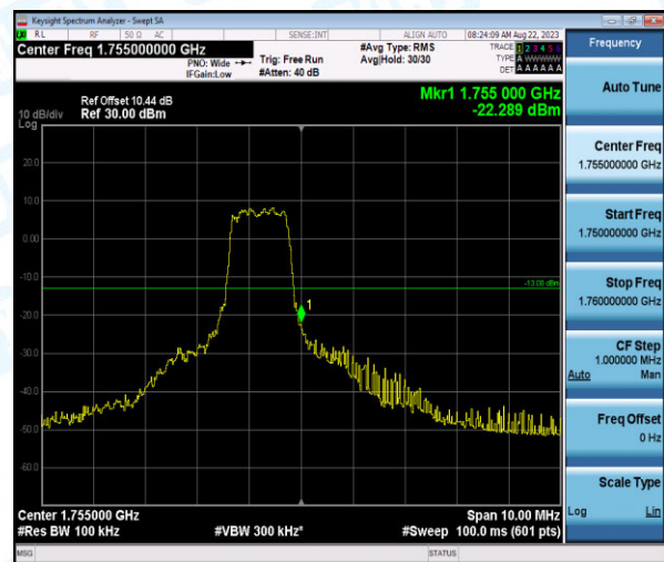
Band4-5MHz-16QAM-20375-6-0-High--22.29-PASS
