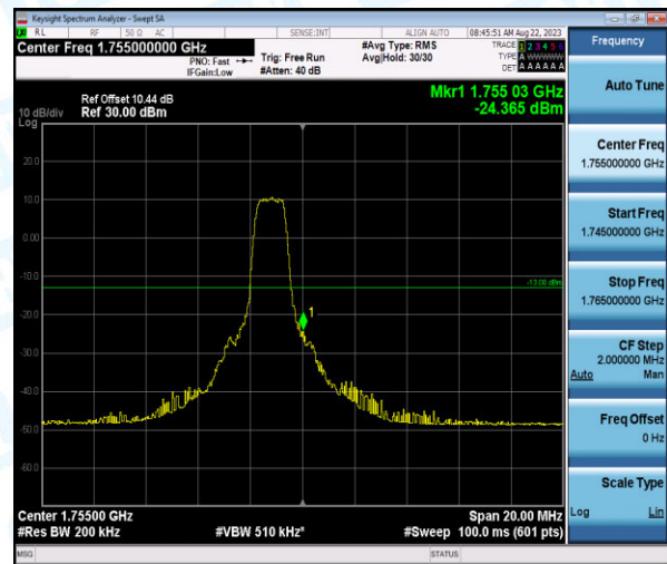
Band4-10MHz-QPSK-20350-6-0-High--24.37-PASS
