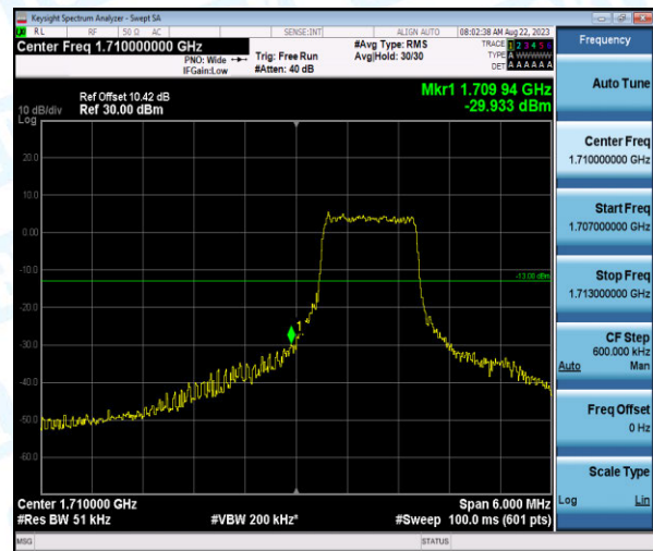
Band4-3MHz-QPSK-19965-6-0-Low--29.93-PASS
