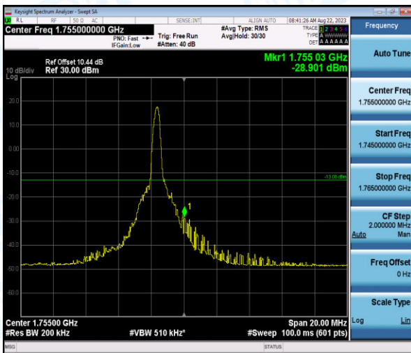
Band4-10MHz-QPSK-20350-1-0-High--28.90-PASS
