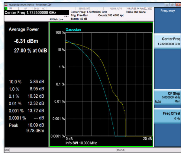
Band4-20MHz-16QAM-20175-6-0-Low-10.32-<=13-PASS
