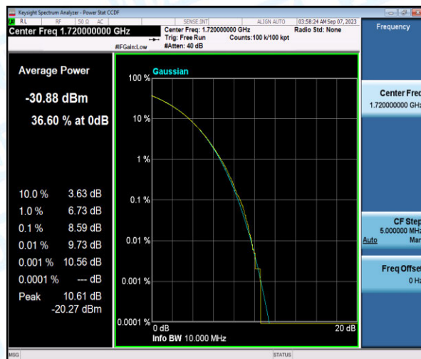
Band4-20MHz-QPSK-20050-6-0-Low-8.59-<=13-PASS
