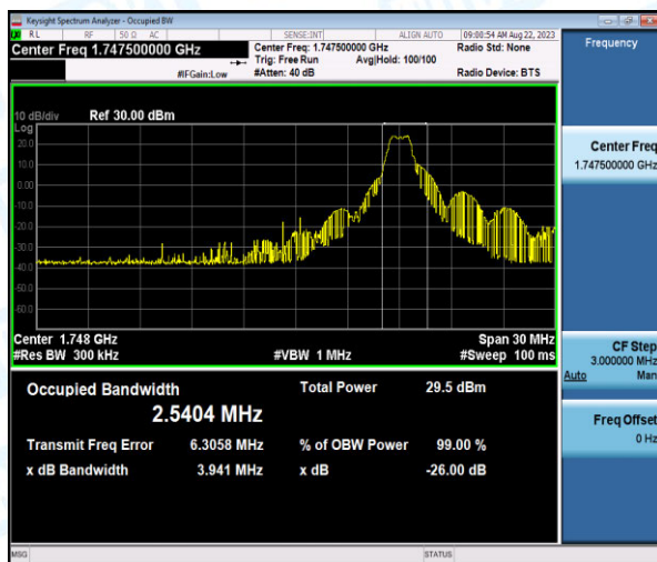
Band4-15MHz-QPSK-20325-6-0-High-2.5404-3.941-PASS
