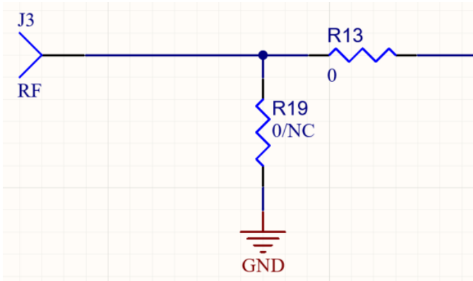
π Type Matching Network
