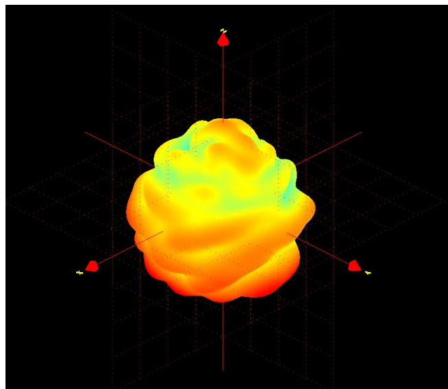
3D Radiation Pattern
