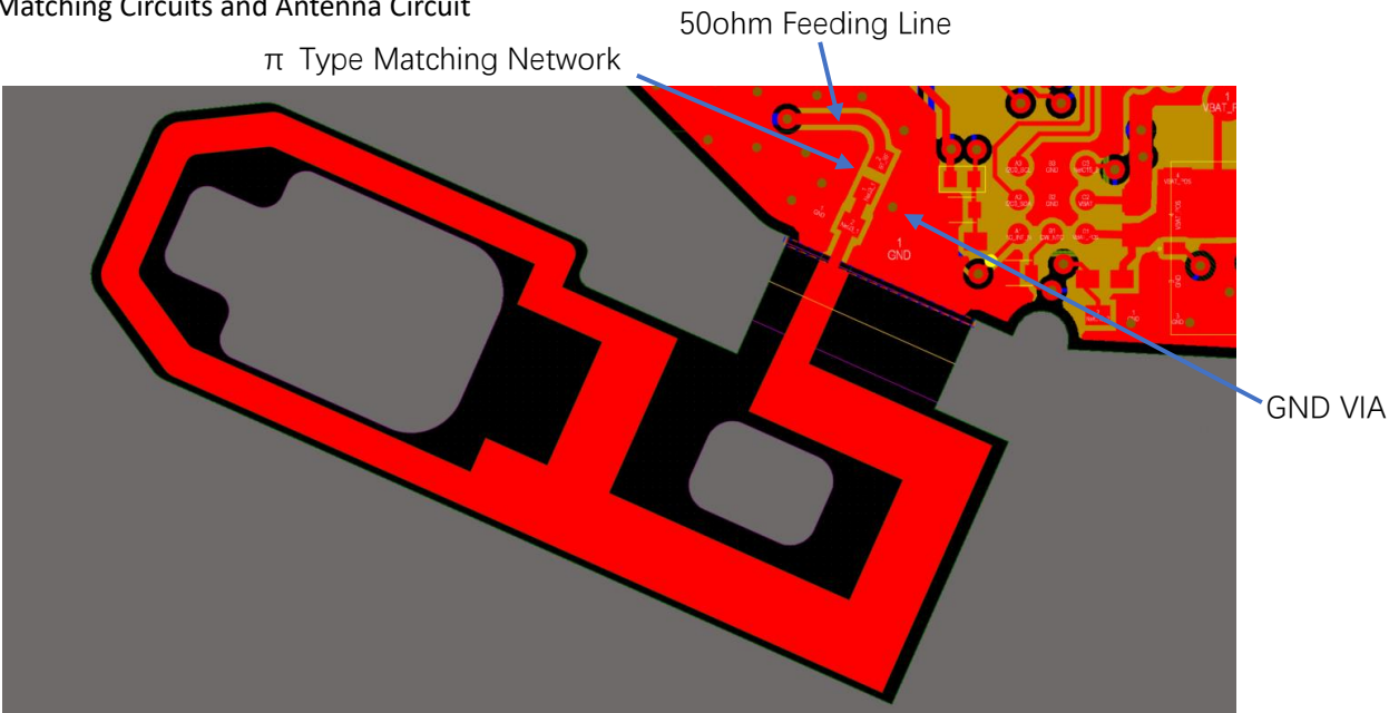
Antenna Layout
