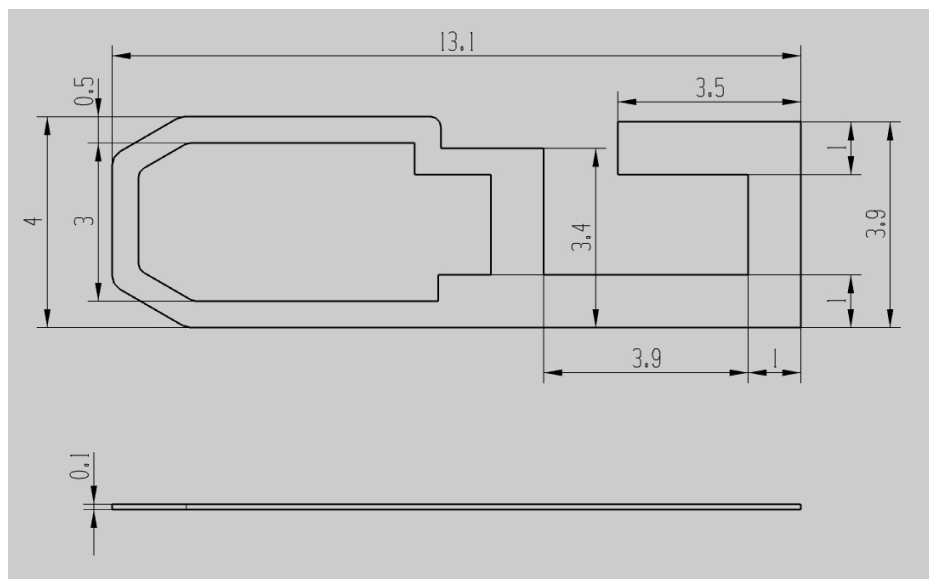
Antenna Dimensions
