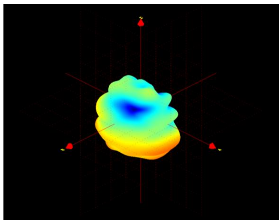
3D Radiation Pattern
