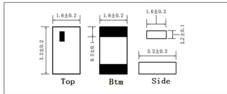
Antenna Dimensions (mm)
