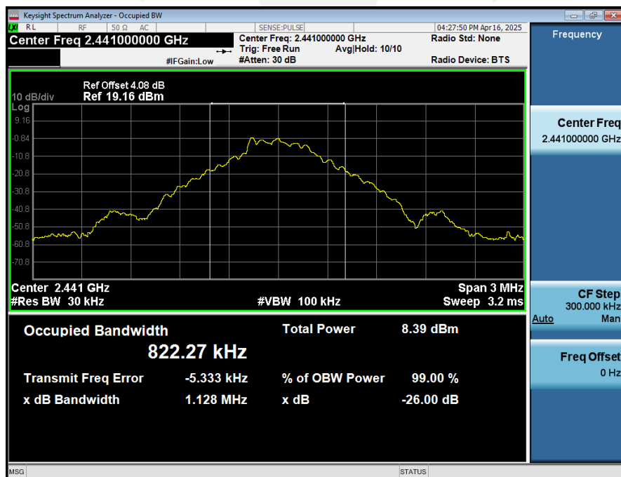
99%_Occupied_Bandwidth_NVNT_ANT1_1-DH1_2441_00
