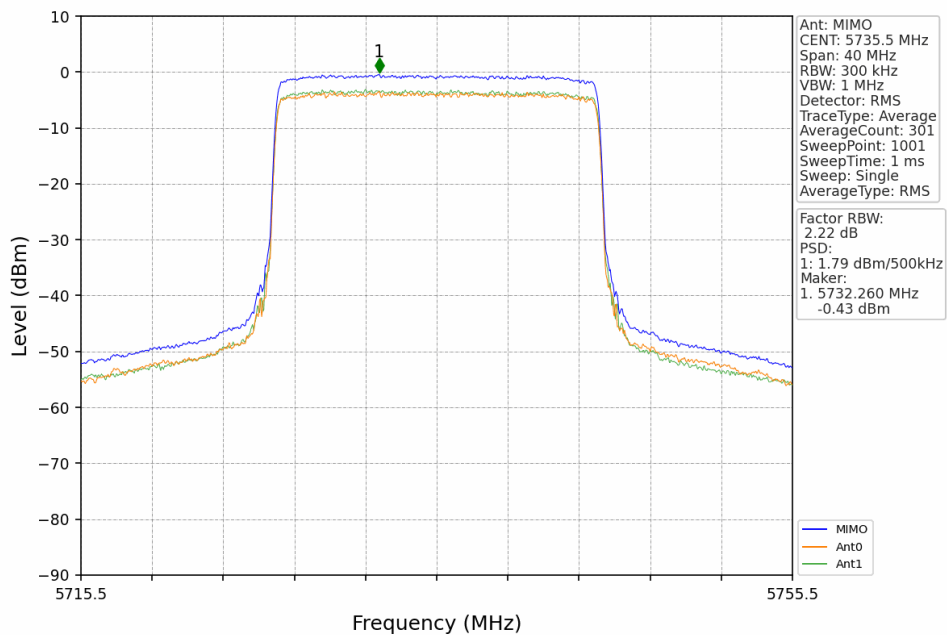
20M_LCH_5735.5MHz_MIMO_NTNV
