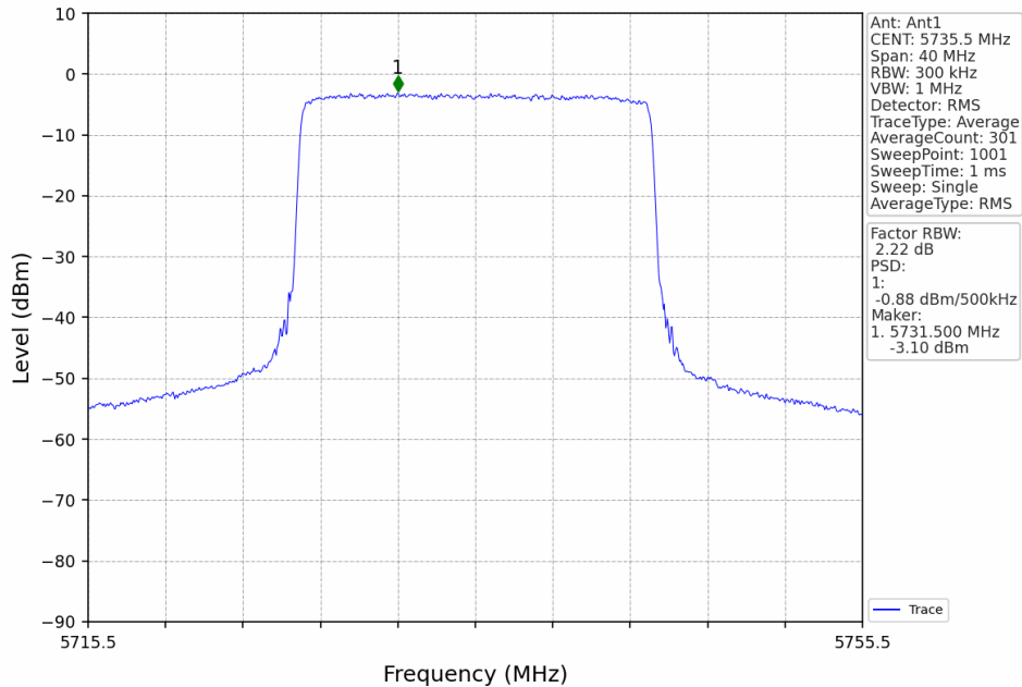
20M_LCH_5735.5MHz_MIMO_NTNV
