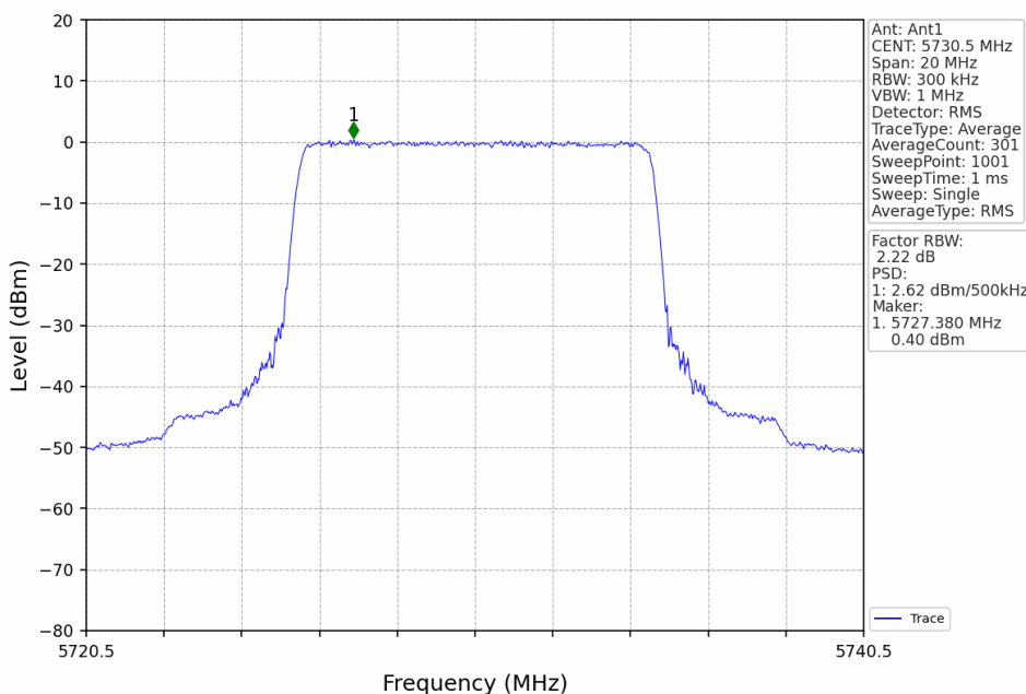
10M_LCH_5730.5MHz_Ant1_NTNV
