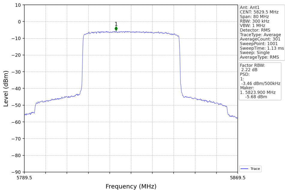
40M_HCH_5829.5MHz_Ant1_NTNV
