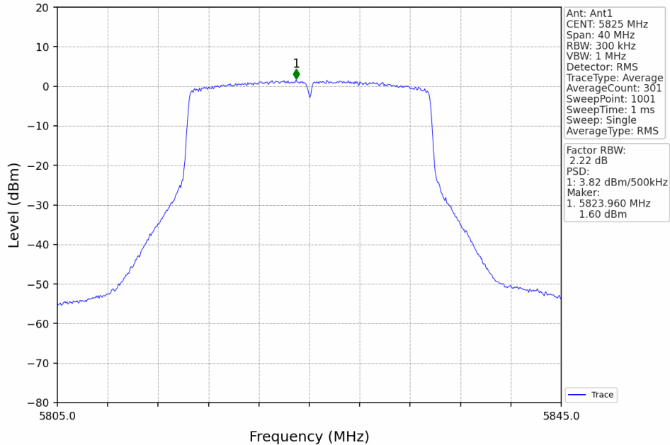
802.11ax(HEW20)_HCH_5825MHz_RU242_Left_MIMO_NTNV
