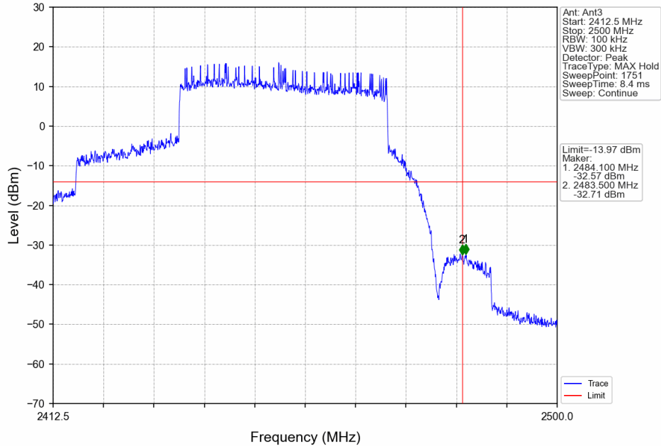
40M_HCH_2452.5MHz_Ant3_NTNV
