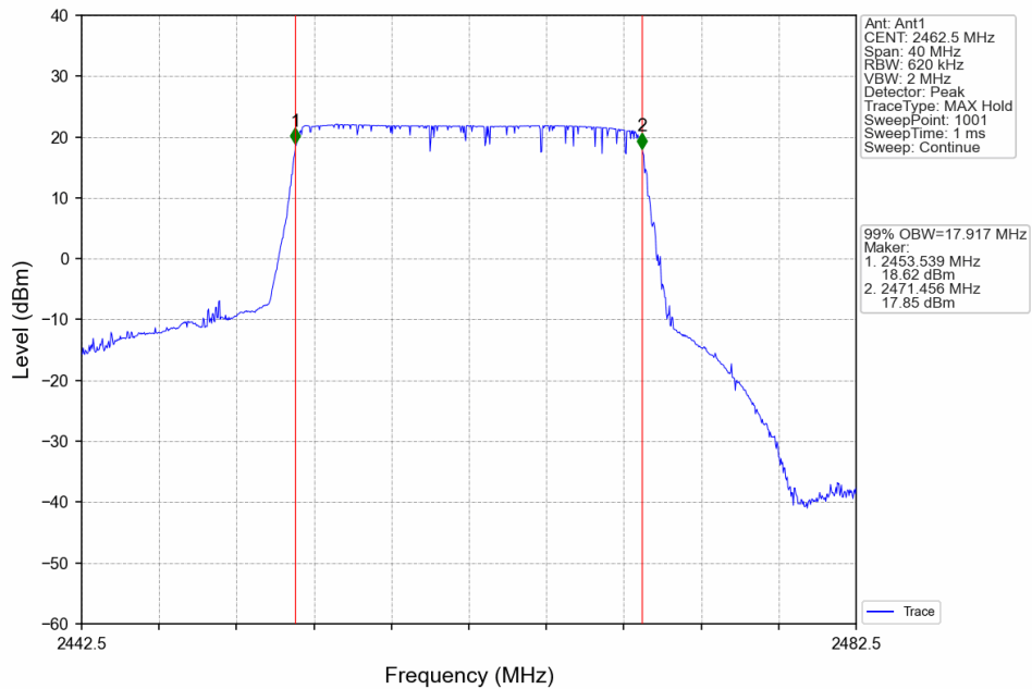
20M_HCH_2462.5MHz_Ant1_NTNV
