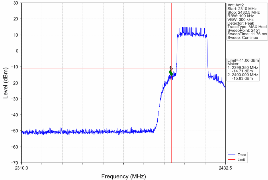
20M_LCH_2412.5MHz_Ant2_NTNV
