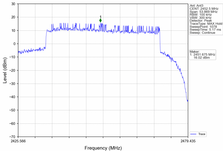
40M_HCH_2452.5MHz_Ant3_NTNV
