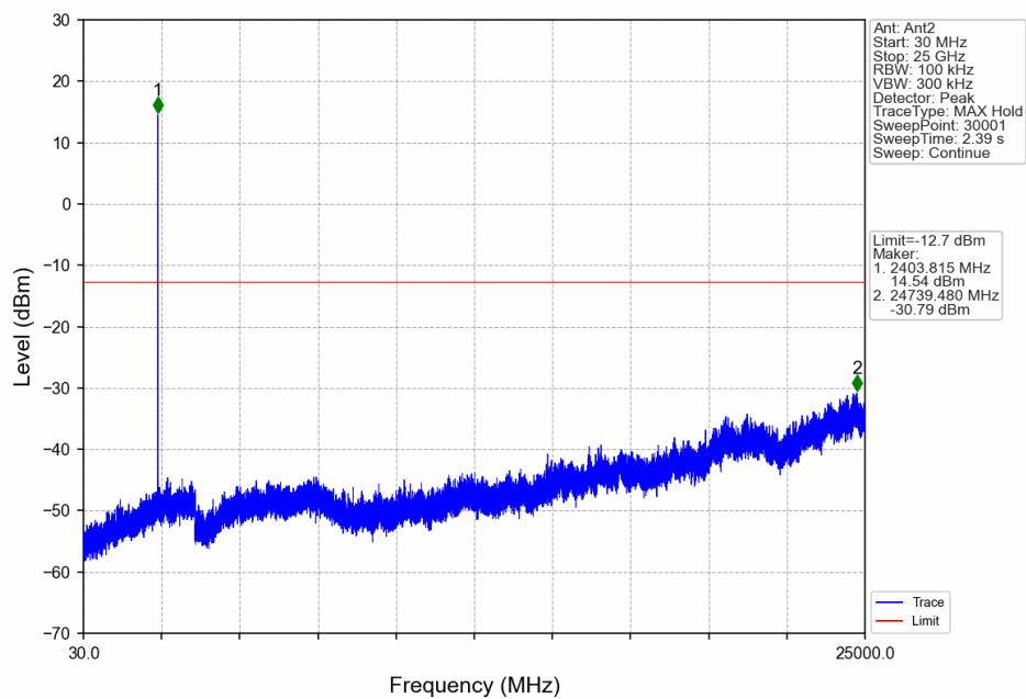
1.4M_LCH_2403.5MHz_Ant2_NTNV
