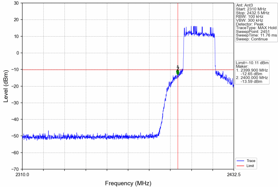
20M_LCH_2412.5MHz_Ant3_NTNV
