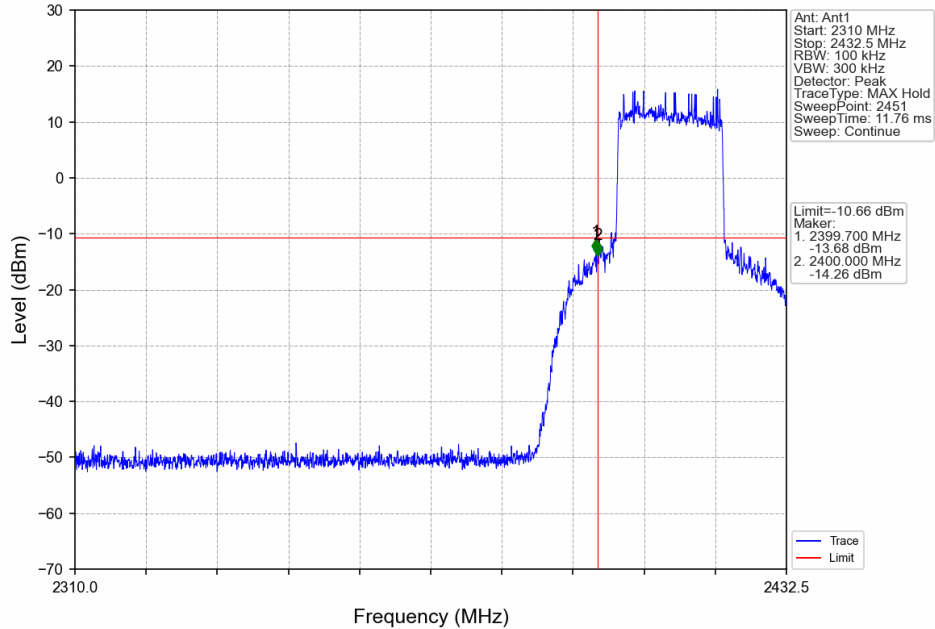
20M_LCH_2412.5MHz_Ant1_NTNV
