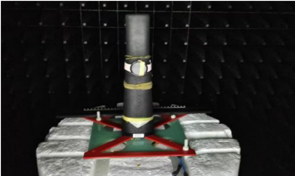
Antenna test environment
