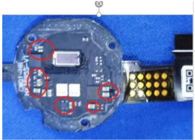
CW Watch S1变更后心率板 CW Watch S1 Post-Modification Heart Rate Board".
