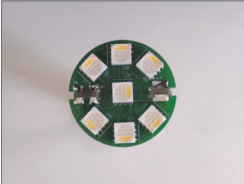
View of Sub1 PCB
