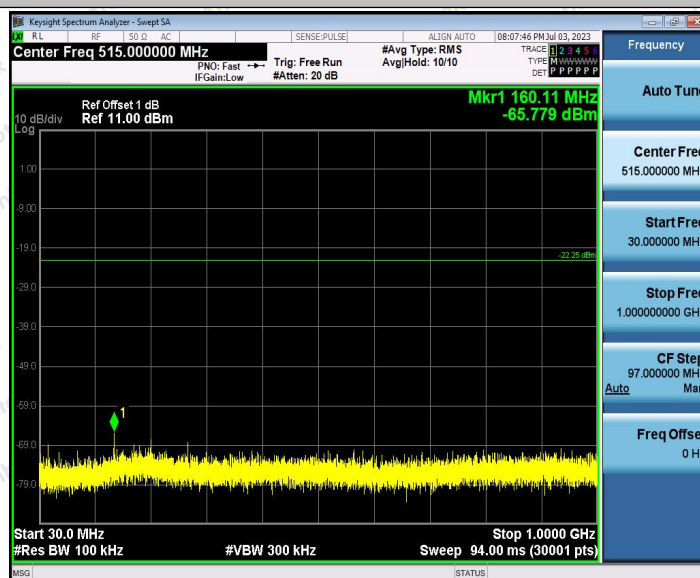
2.4G_Ant1_2451_30~1000
