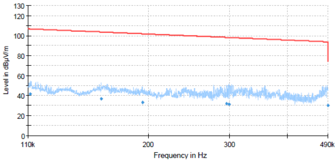
Radiates Emission from 110kHz to 490kHz
