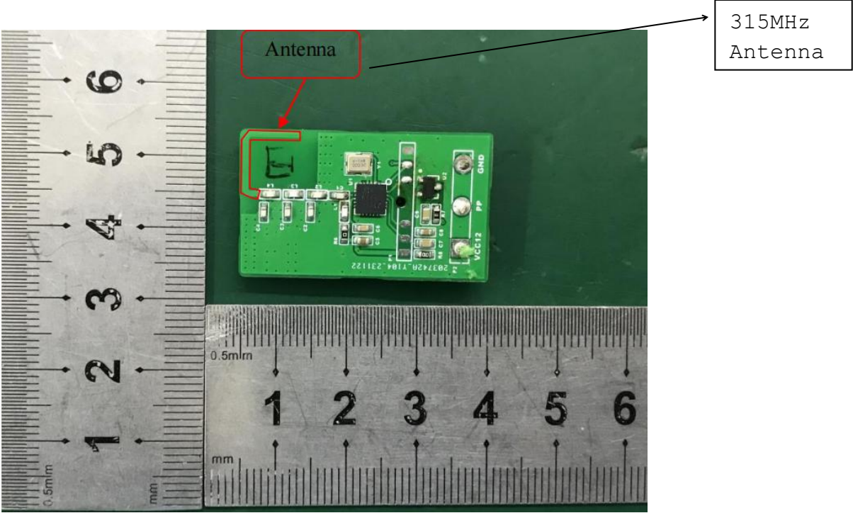
INTERNAL PHOTO OF SAMPLE PCB
