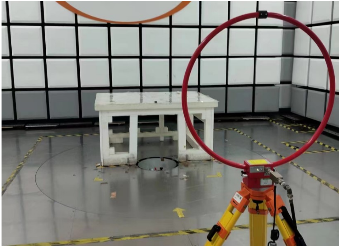
Description: Test Setup
