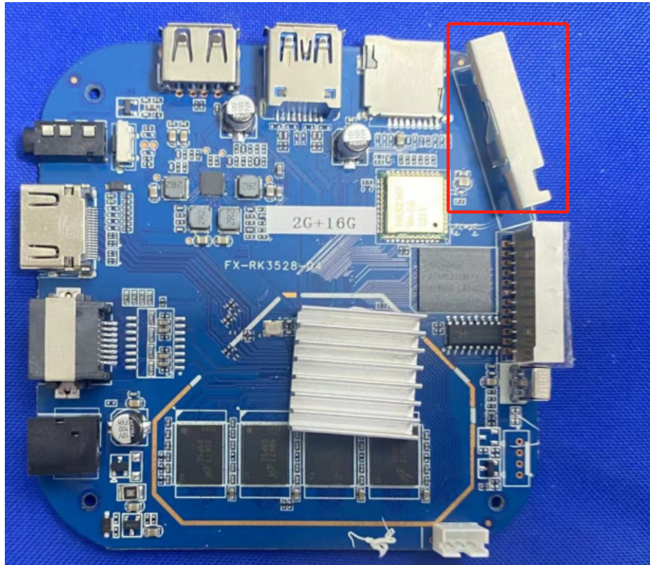
Antenna pattern
