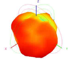
2400.0MHz H+V, Eff: 39.9%
