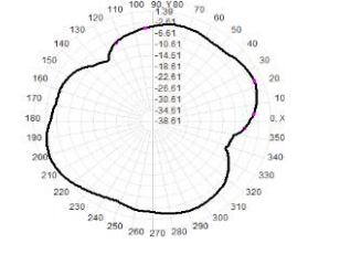
Total(H-XY), Max= -1.79dBi, CirD=9.93
