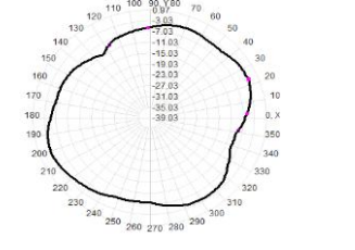
Total(H-XY), Max= -2.60dBi, CirD=8.18
