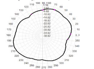
Total(H-XY), Max= -2.43dBi, CirD=7.34
