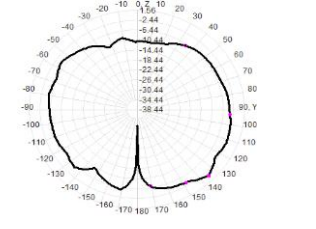
2420.0MHz Total(E2-YZ), Max= -1.31dBi
