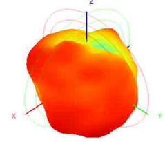
2420.0MHz H+V, Eff: 39.8%
