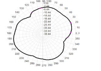
Total(H-XY), Max= -2.01dBi, CirD=8.55
