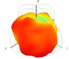
2430.0MHz H+V, Eff: 39.0%
