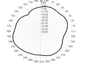
Total(H-XY), Max= -1.83dBi, CirD=7.97
