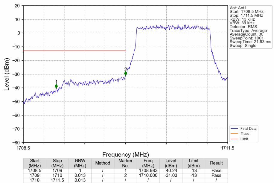
Band4_1.4MHz_QPSK_LCH_1710.7MHz_RB_6_0_NTNV
