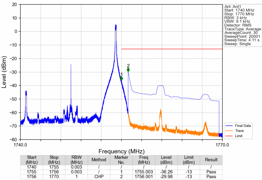
Band4_15MHz_16QAM_HCH_1747.5MHz_RB_1_74_NTNV
