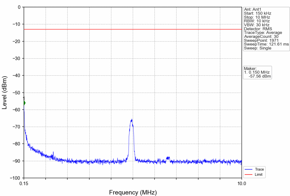
Band4_15MHz_16QAM_LCH_1717.5MHz_RB_1_0_NTNV
