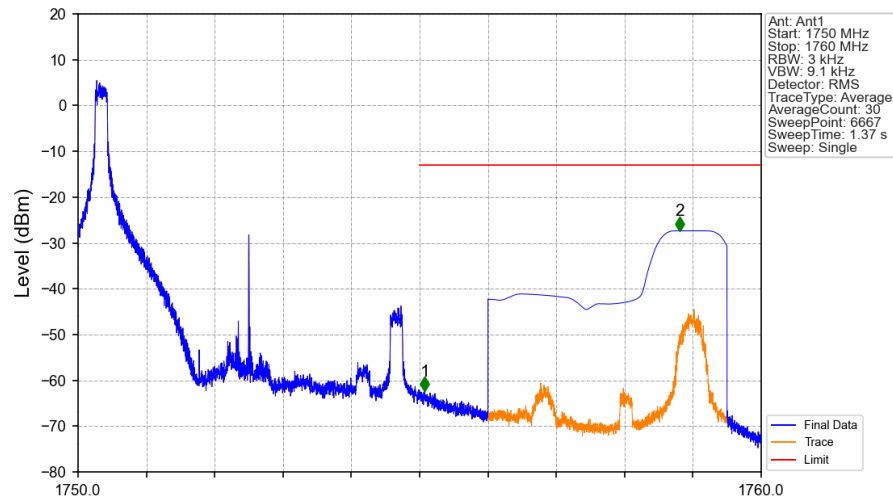
Band4_5MHz_16QAM_HCH_1752.5MHz_RB_1_0_NTNV
