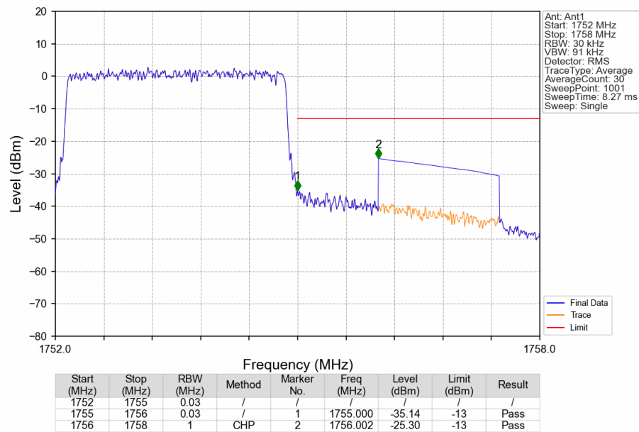
Band4_3MHz_16QAM_HCH_1753.5MHz_RB_15_0_NTNV
