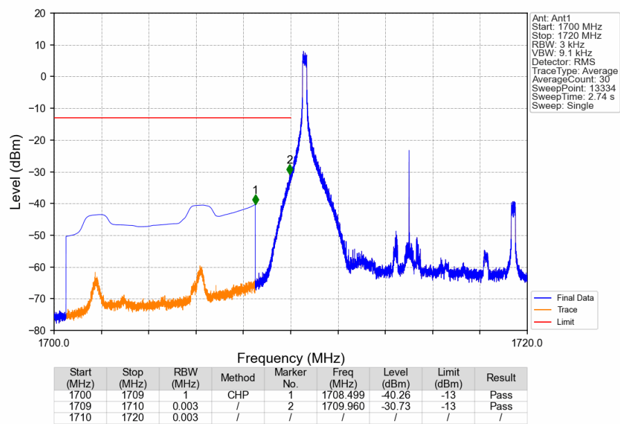
Band4_10MHz_16QAM_LCH_1715MHz_RB_1_0_NTNV
