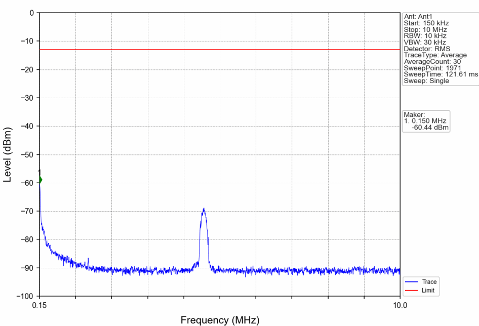
Band4_10MHz_16QAM_LCH_1715MHz_RB_1_0_NTNV
