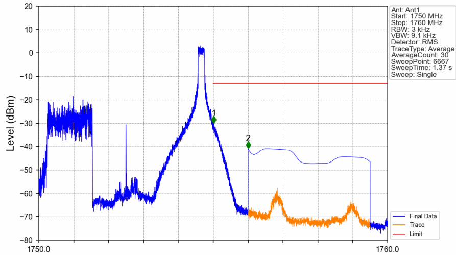
Band4_5MHz_QPSK_HCH_1752.5MHz_RB_1_24_NTNV
