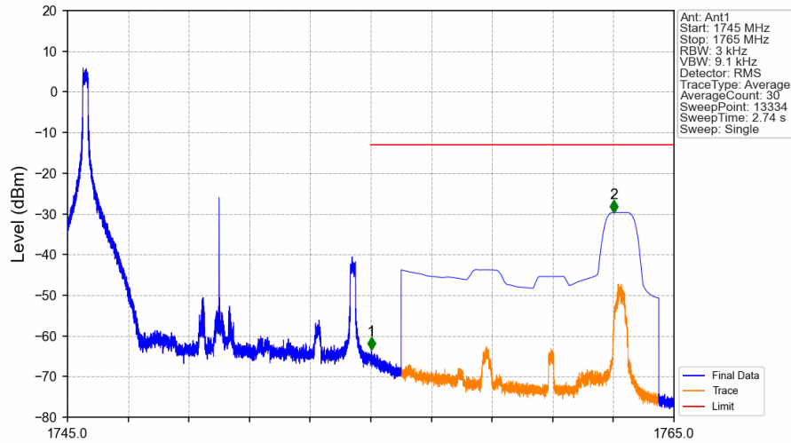
Band4_10MHz_16QAM_HCH_1750MHz_RB_1_0_NTNV
