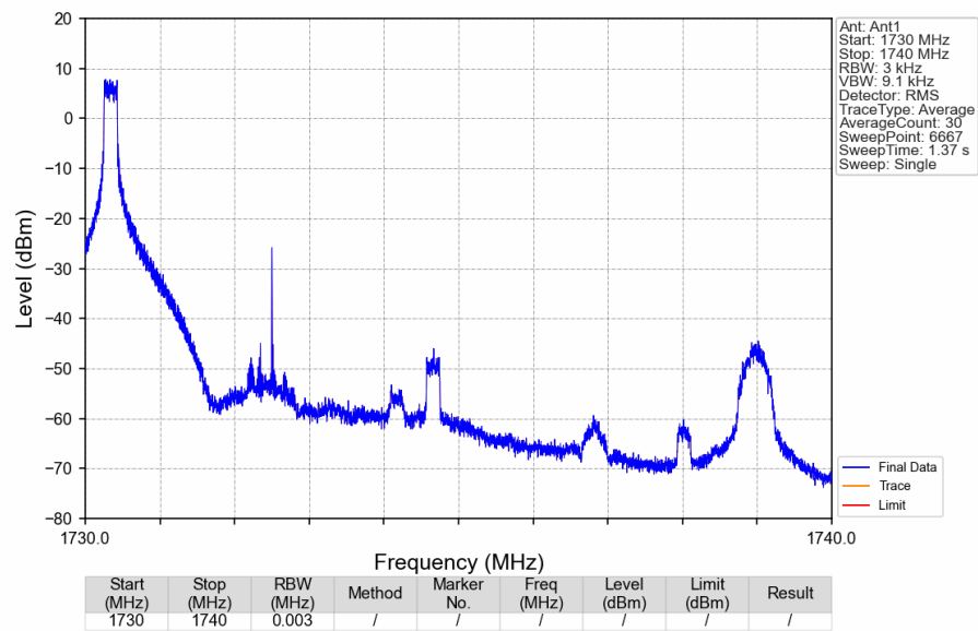
Band4_5MHz_16QAM_MCH_1732.5MHz_RB_1_0_NTNV
