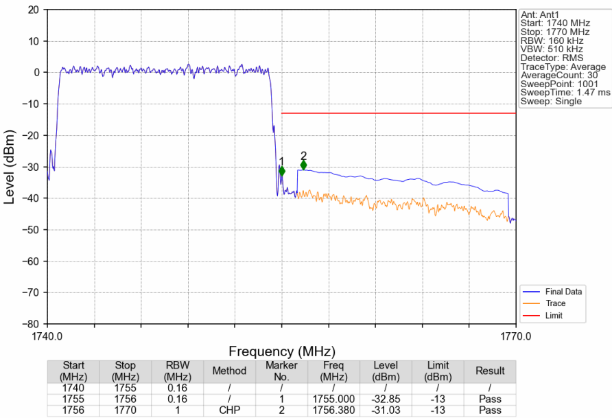
Band4_15MHz_16QAM_HCH_1747.5MHz_RB_75_0_NTNV
