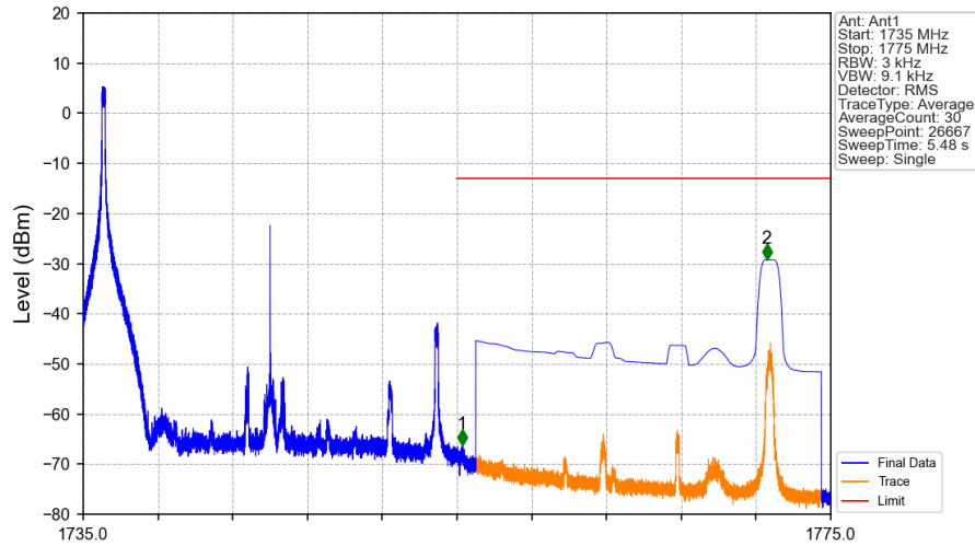
Band4_20MHz_16QAM_HCH_1745MHz_RB_1_0_NTNV
