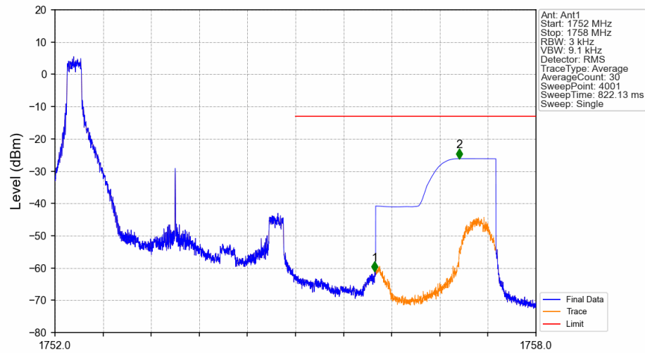
Band4_3MHz_16QAM_HCH_1753.5MHz_RB_1_0_NTNV
