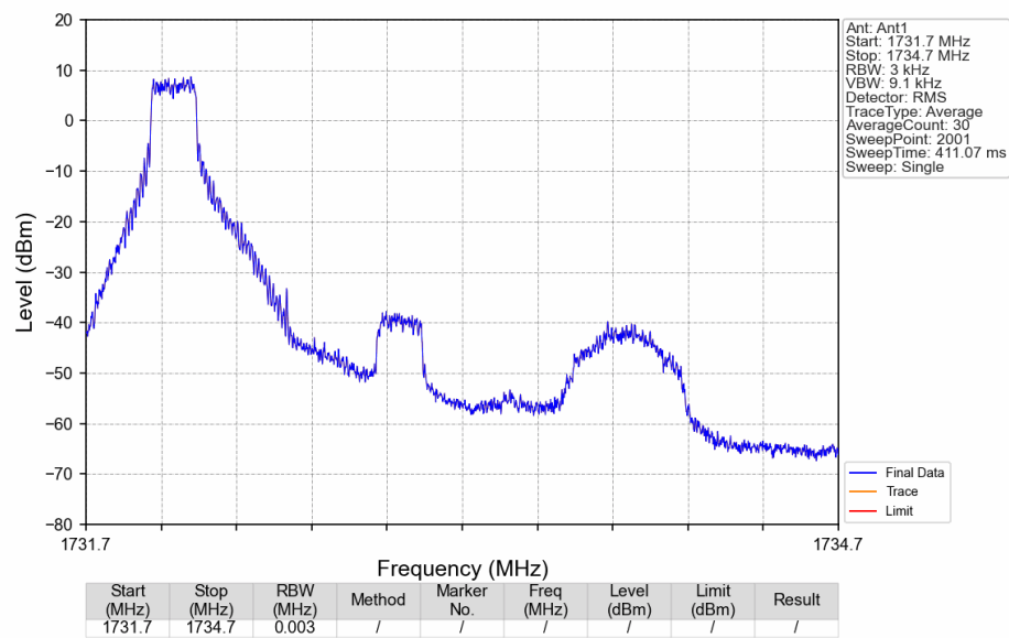
Band4_1.4MHz_QPSK_MCH_1732.5MHz_RB_1_0_NTNV
