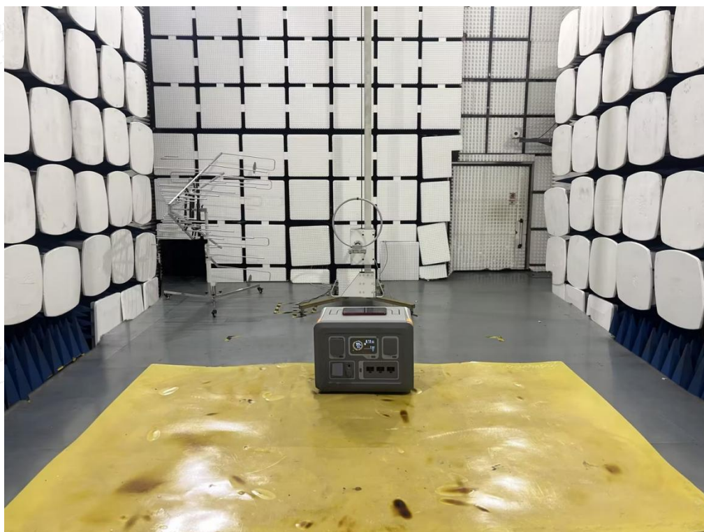
Radiated Emission below 30MHz-TM4
