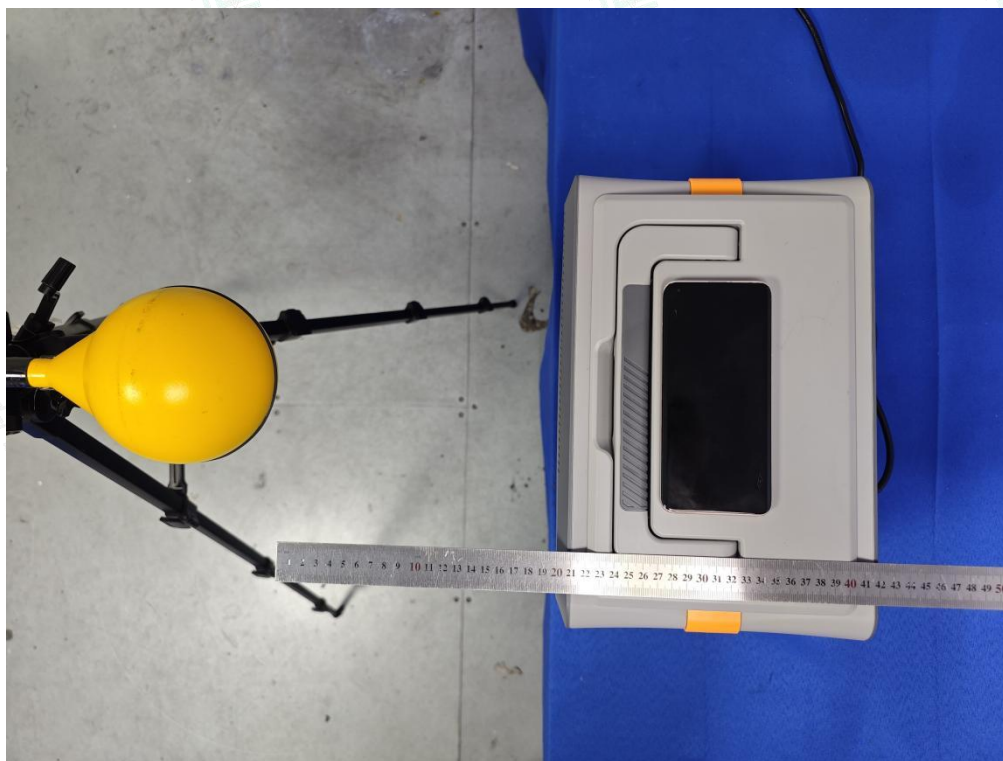
Test Position B(20cm) - Exposure photo from side edge surface-Rear(TM4)
