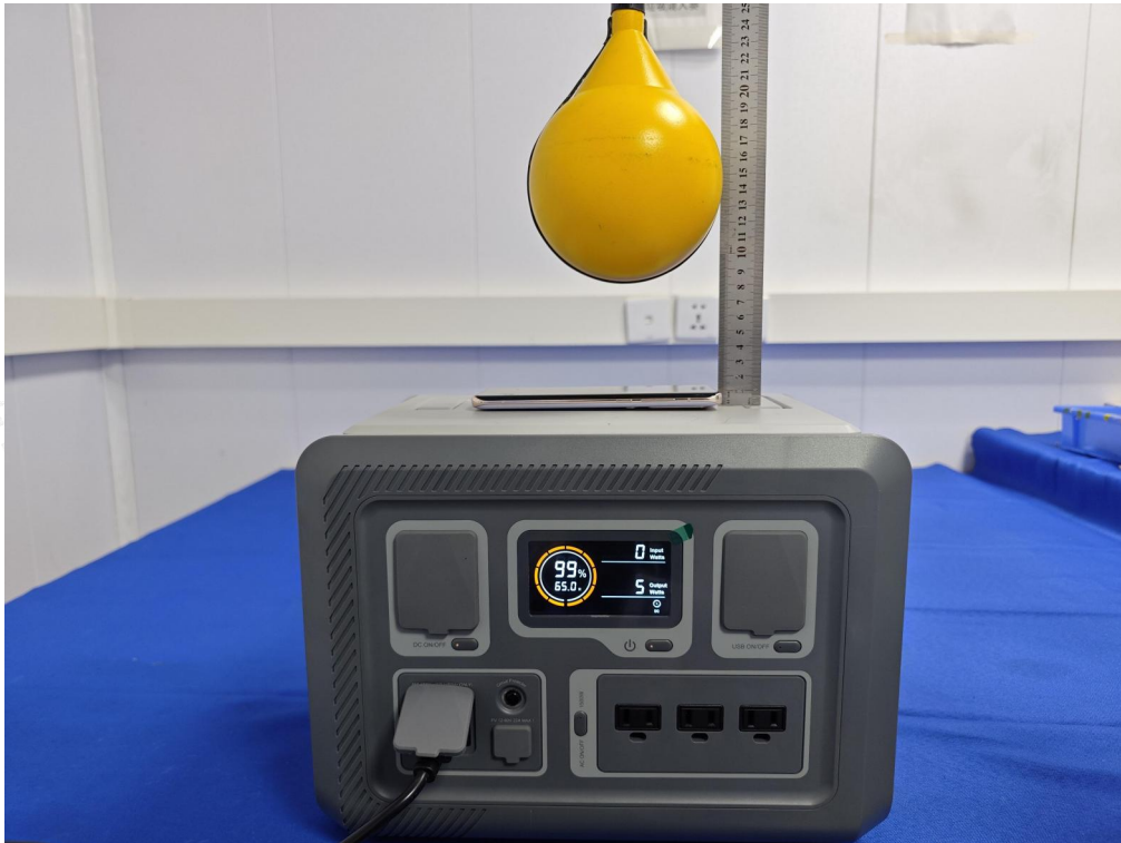
Test Position A (8cm) - Exposure photo from top surface (TM4)
