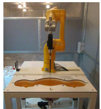
Figure 4.1 DASY5 Test System
