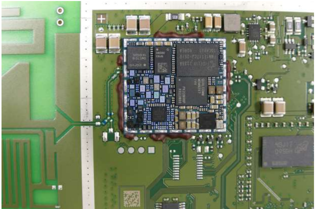
LARA-R6 without shielding
