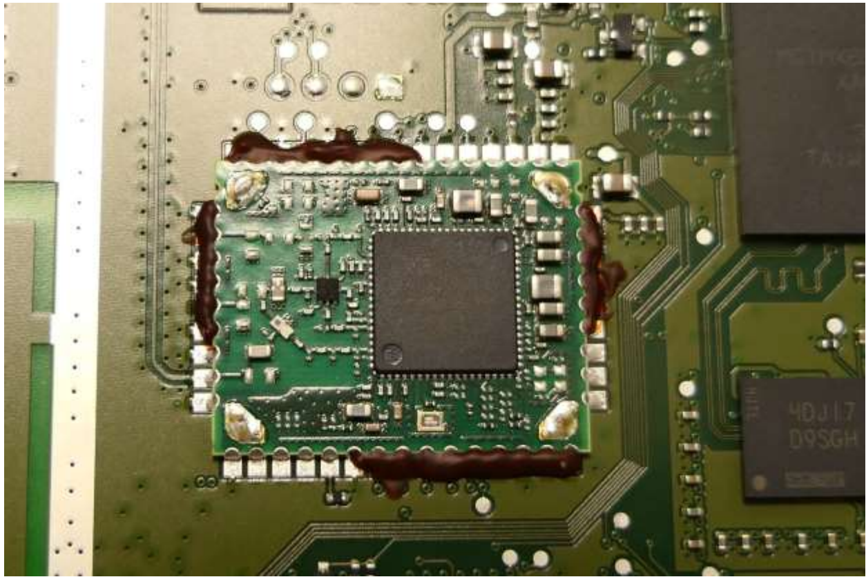
ALPS WLAN Module without shielding
