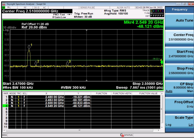
Right bandedge
