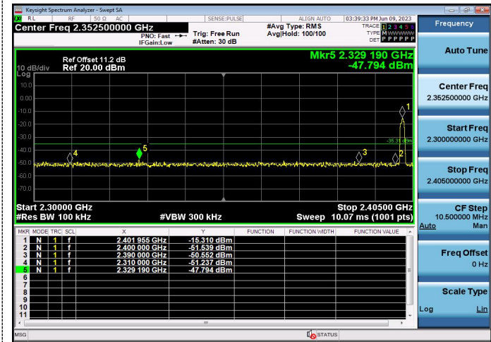
Left bandedge
