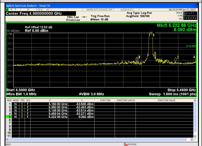
Out Of Band Emission IEEE 802.11n_Channel 44_20MHz_Antenna 0
