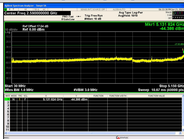
Spurious Emission:30.0~5150 MHz IEEE 802.11n_Channel 44_20MHz_Antenna 0
