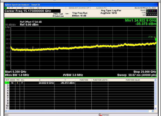
Spurious Emission:5350~25000.0 MHz IEEE 802.11n_Channel 44_20MHz_Antenna 0
