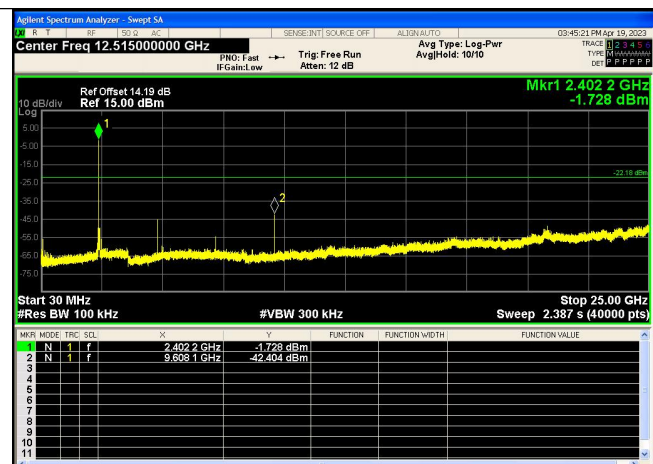
Spurious Emission 8DPSK_3-DH5_Channel 0
