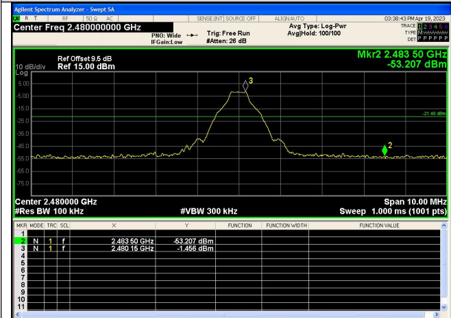
Out Of Band Emission GFSK_DH5_Channel 78
