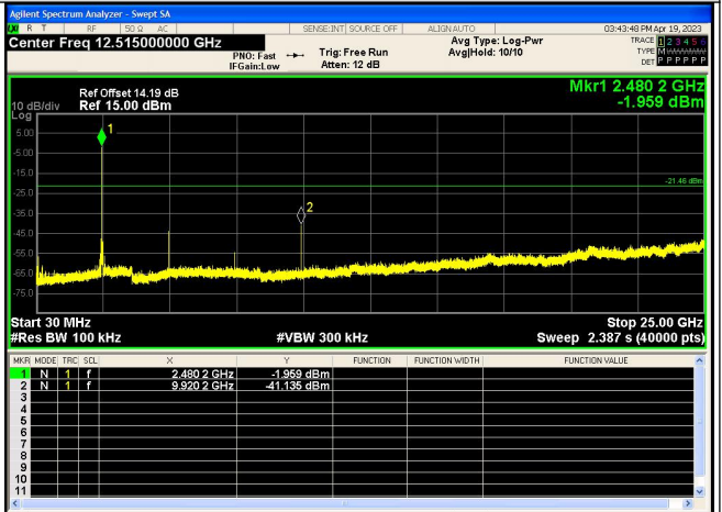
Spurious Emission \pi/4 DQPSK_2-DH5_Channel 78
