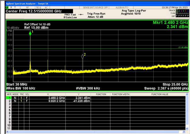
Spurious Emission GFSK_DH5_Channel 78
