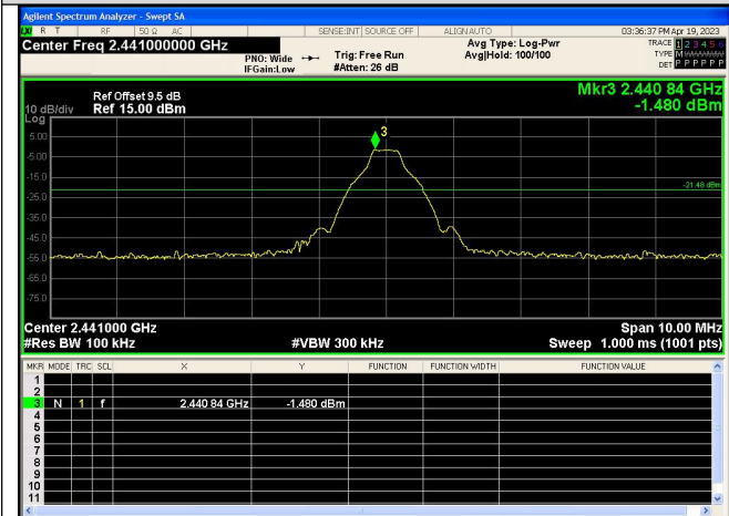
Out Of Band Emission GFSK_DH5_Channel 39
