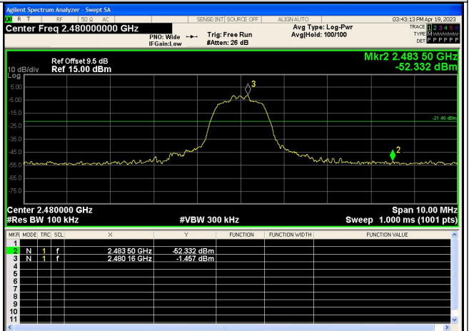
Out Of Band Emission \pi/4 DQPSK_2-DH5_Channel 78
