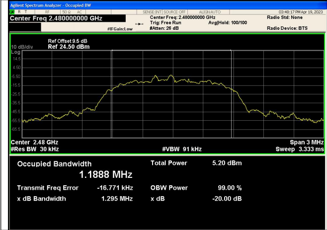
8DPSK_3-DH5_Channel 78
