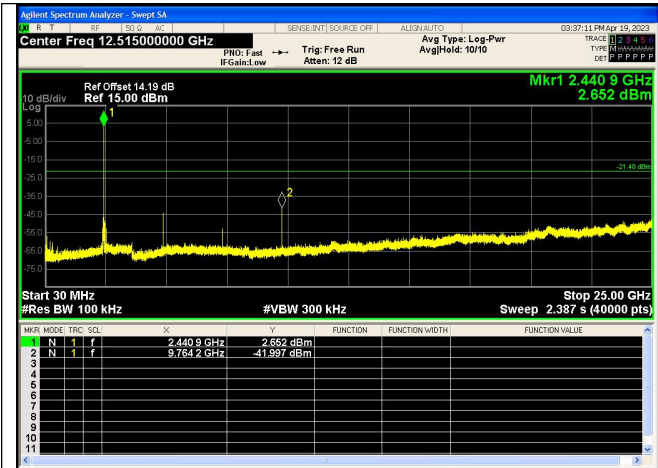
Spurious Emissions GFSK_DH5_Channel 39
