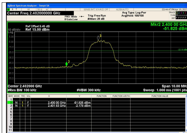
Out Of Band Emission 8DPSK_3-DH5_Channel 0
