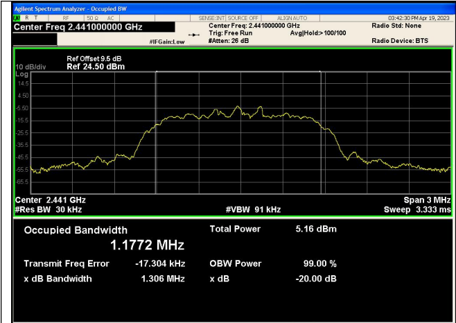
\pi/4 DQPSK_2-DH5_Channel 39
