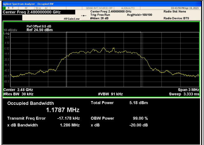
\pi/4 DQPSK_2-DH5_Channel 78
