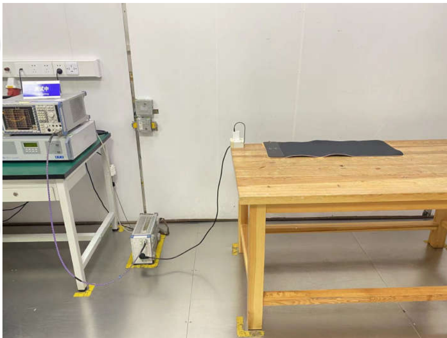
Conducted Emissions-1
