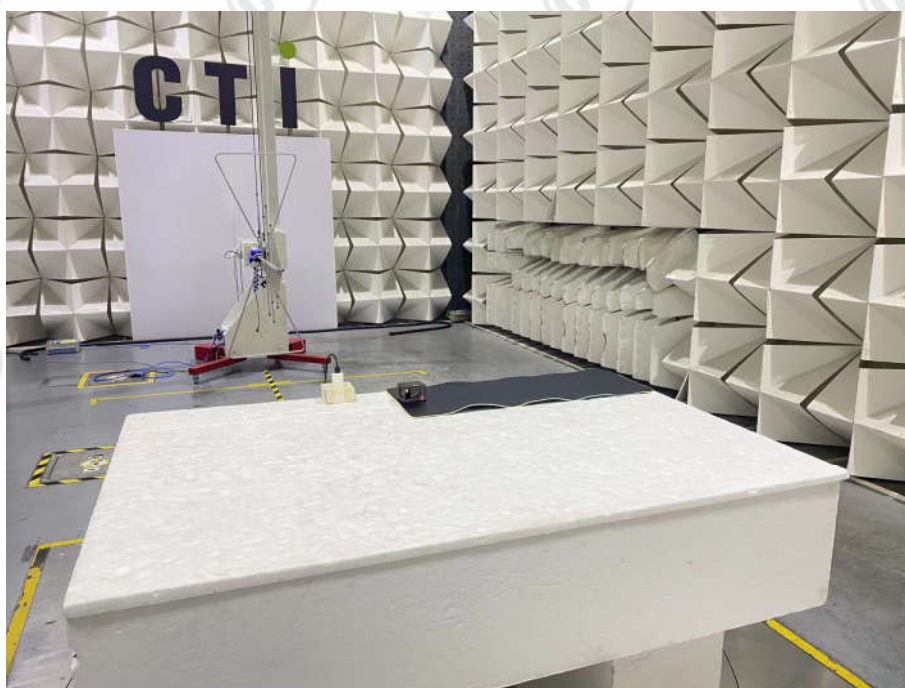
Radiated Spurious Emissions Test Setup (9kHz~30MHz)-2
