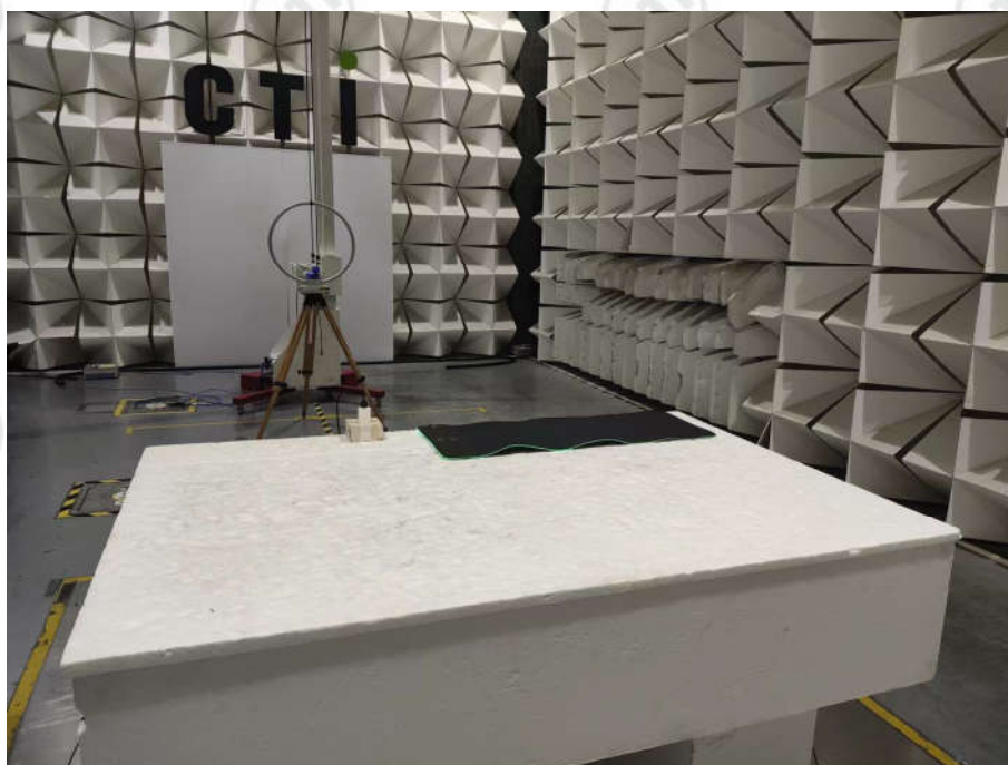
Radiated Spurious Emissions Test Setup (9kHz~30MHz)-1
