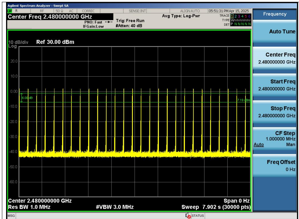
Test_Graph_BR_HOP_ANT1_NA_2Mbps_2480_Number of Burst
