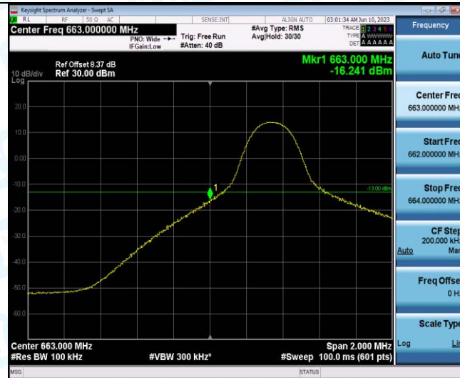
Band71-5MHz-16QAM-133147-1RB#24
