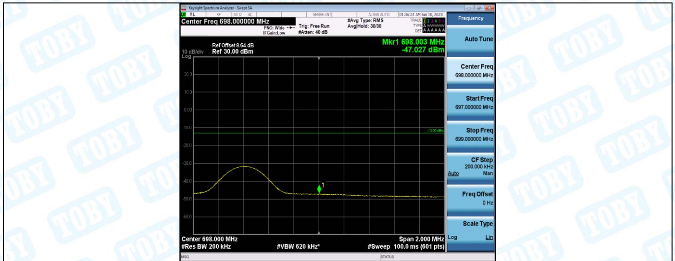
Band71-10MHz-16QAM-133422-1RB#49
