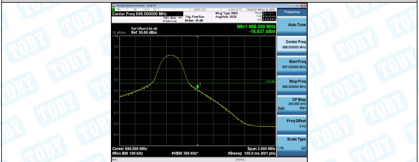
Band71-5MHz-16QAM-133447-25RB#0
