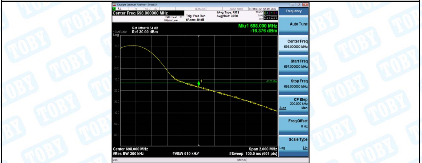
Band71-15MHz-QPSK-133397-75RB#0
