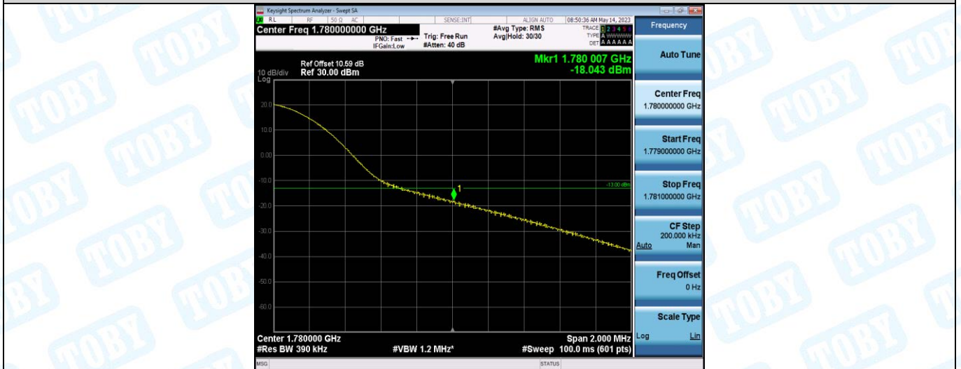
Band66-20MHz-16QAM-132572-100RB#0
