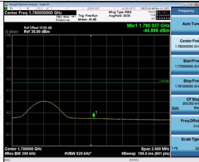
Band66-10MHz-16QAM-132622-1RB#49
