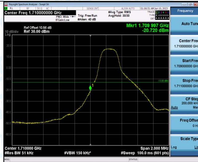
Band66-3MHz-QPSK-131987-1RB#14
