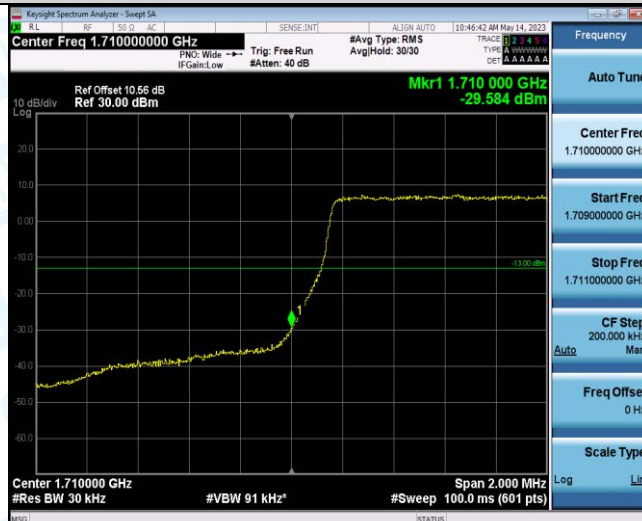
Band66-1.4MHz-QPSK-131979-6RB#0
