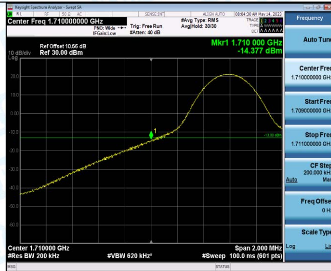
Band66-10MHz-16QAM-132022-1RB#49
