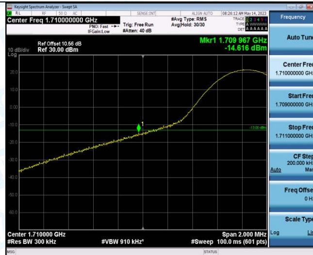
Band66-15MHz-16QAM-132047-1RB#74
