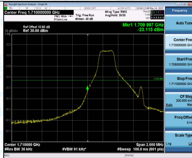
Band66-1.4MHz-16QAM-131979-1RB#5
