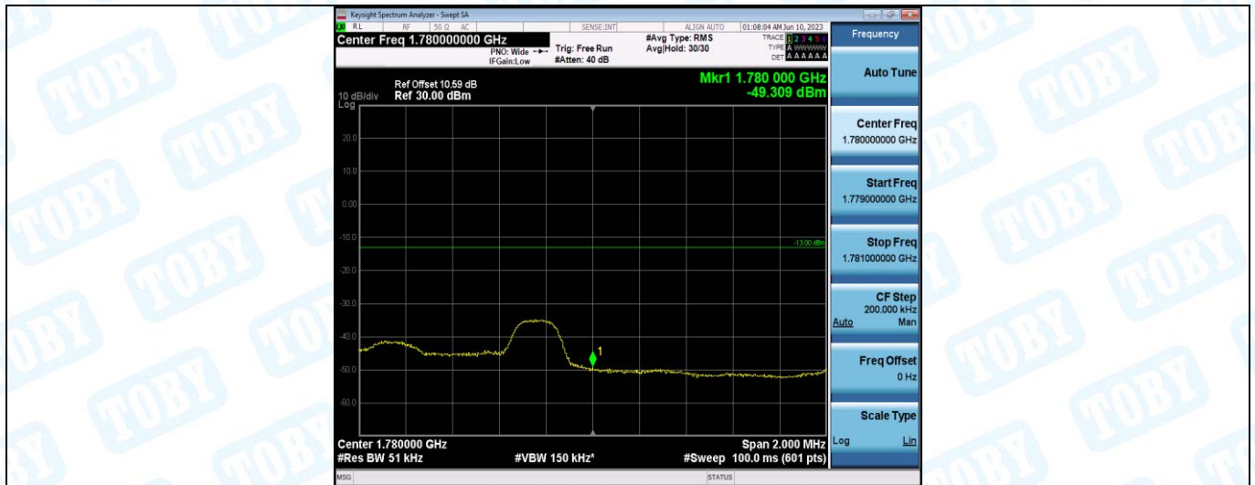
Band66-3MHz-QPSK-132657-1RB#14
