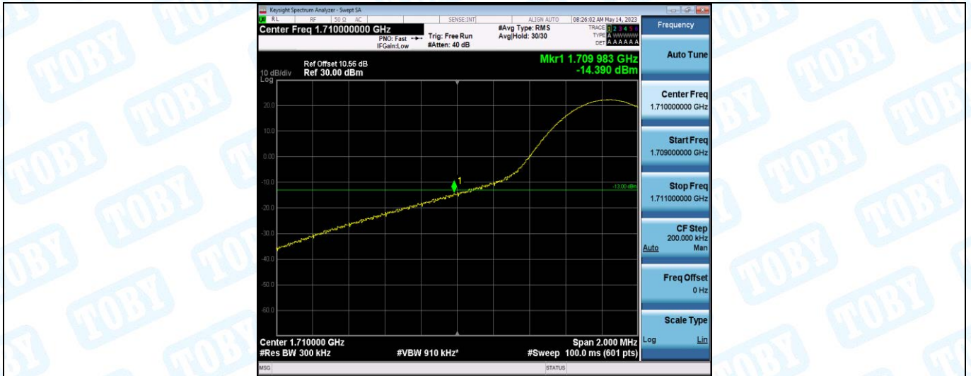
Band66-15MHz-QPSK-132047-1RB#74
