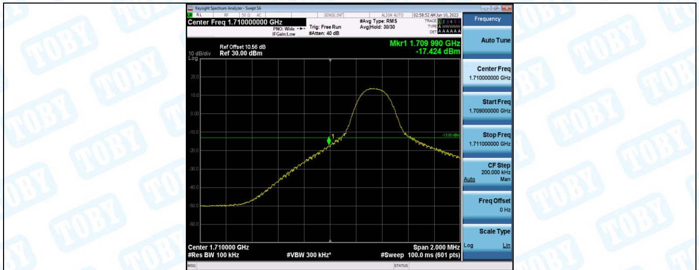
Band66-5MHz-QPSK-131997-1RB#24
