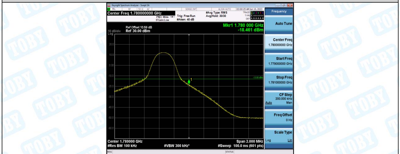
Band66-5MHz-QPSK-132647-25RB#0
