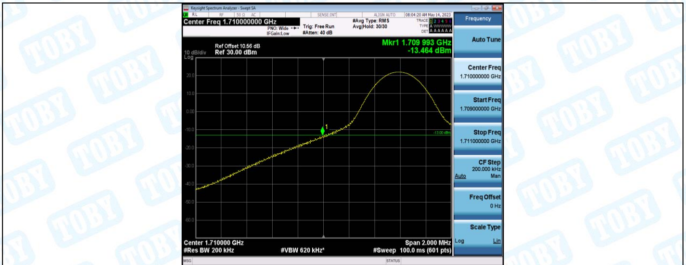
Band66-10MHz-QPSK-132022-1RB#49
