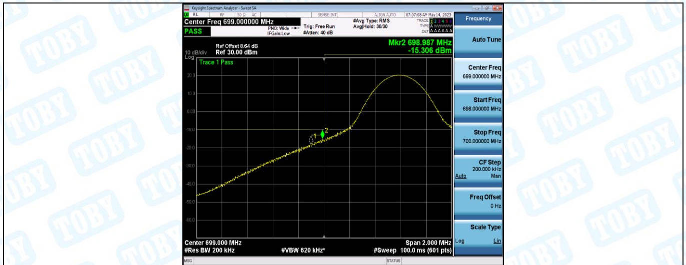
Band12-10MHz-QPSK-23060-1RB#49
