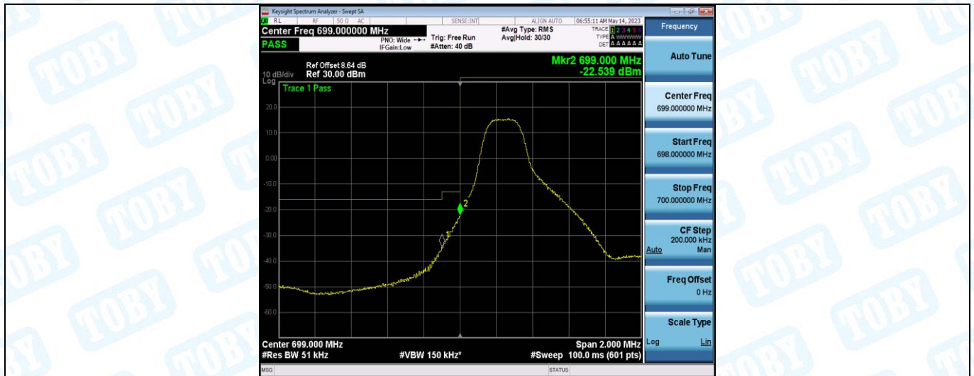
Band12-3MHz-16QAM-23025-1RB#14
