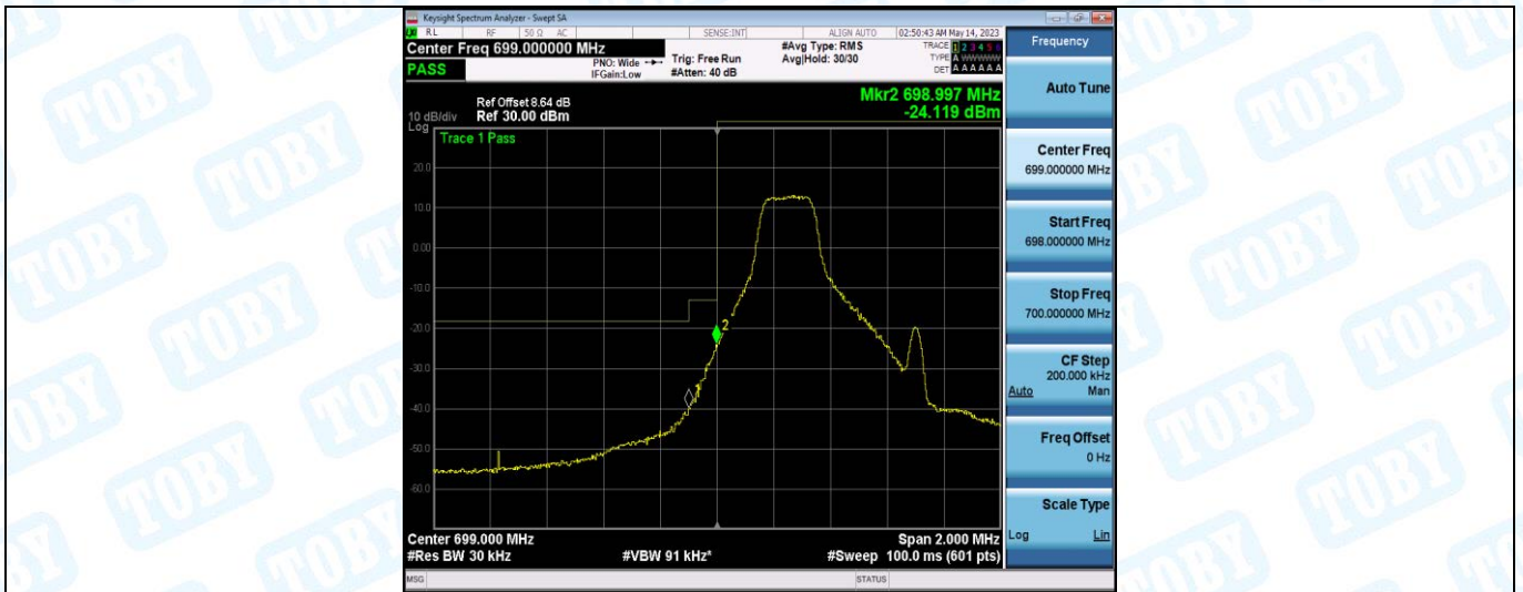
Band12-1.4MHz-16QAM-23017-1RB#5
