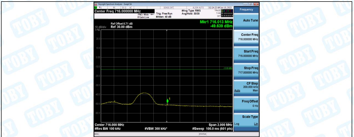
Band12-5MHz-16QAM-23155-1RB#24
