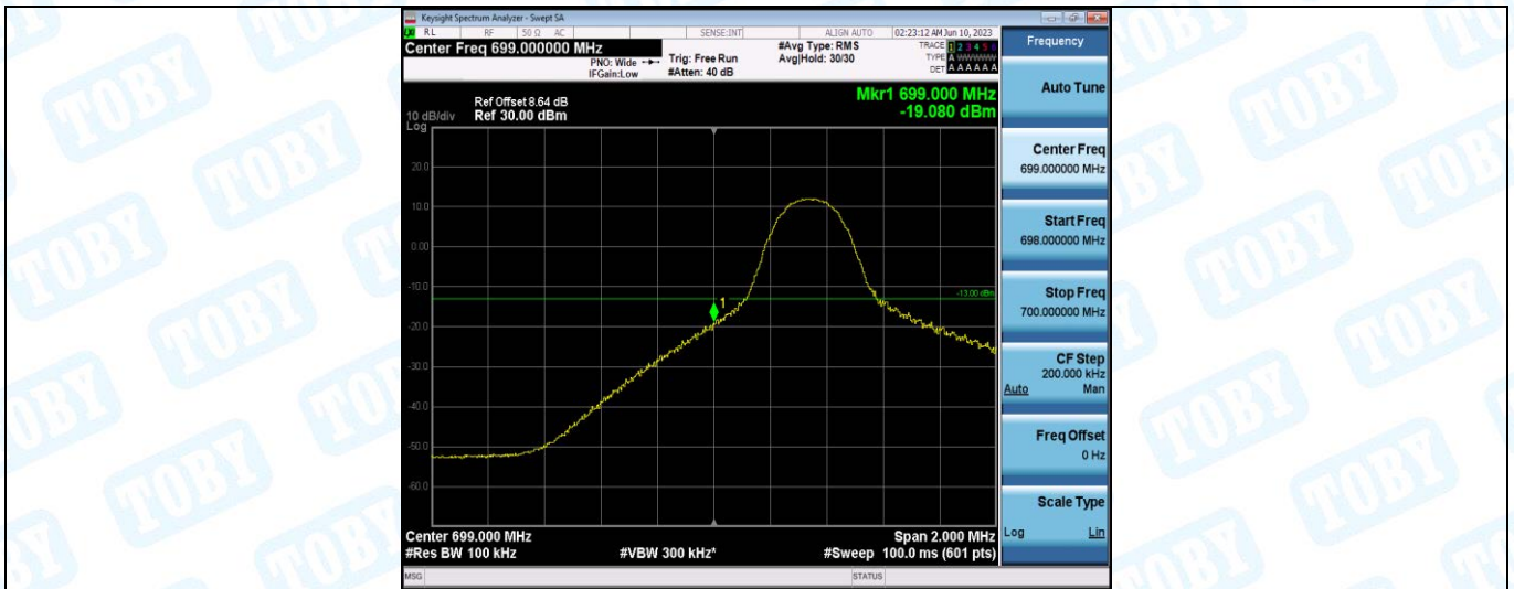
Band12-5MHz-16QAM-23035-1RB#24
