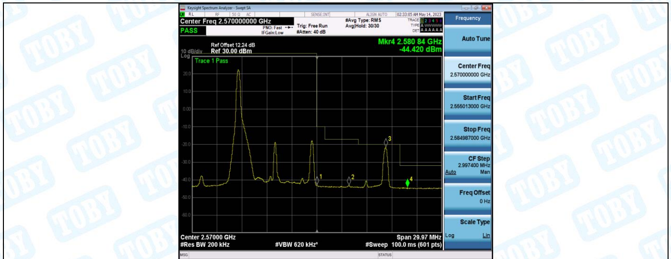
Band7-10MHz-QPSK-21400-1RB#49
