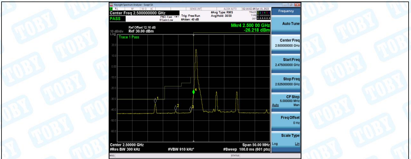
Band7-15MHz-16QAM-20825-1RB#74
