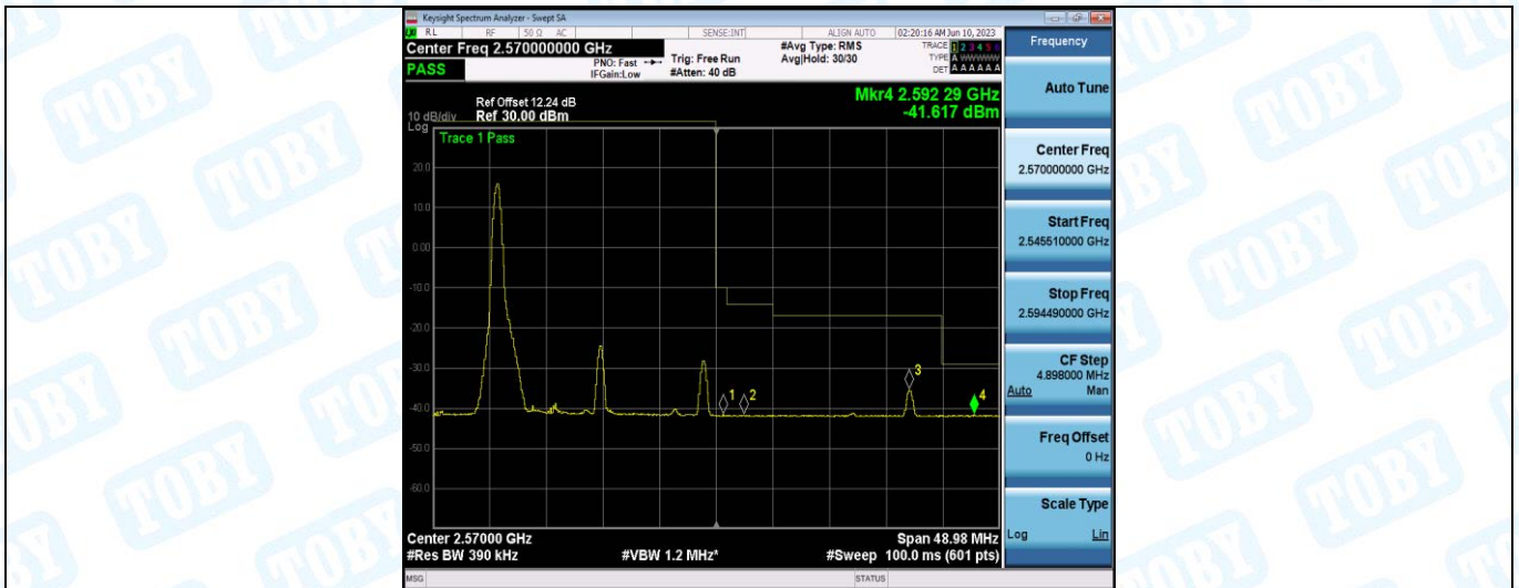
Band7-20MHz-16QAM-21350-1RB#99
